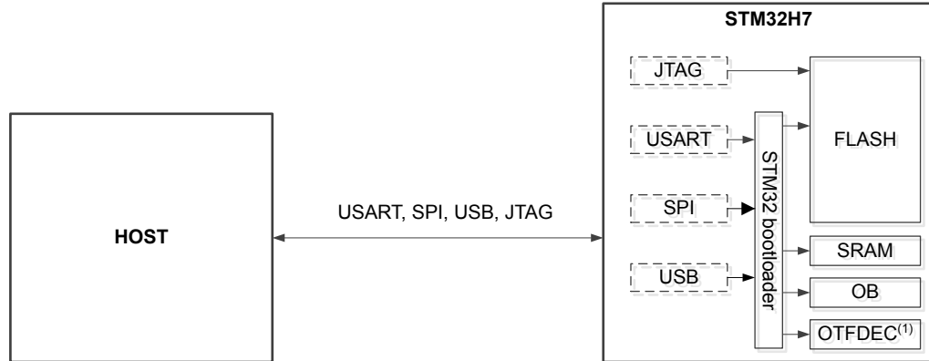
Figure 8. STM32H75xxx/STM32H7B0xx/STM32H7B3xx/STM32H730xx/STM32H733xx/STM32H735xx secure bootloader
