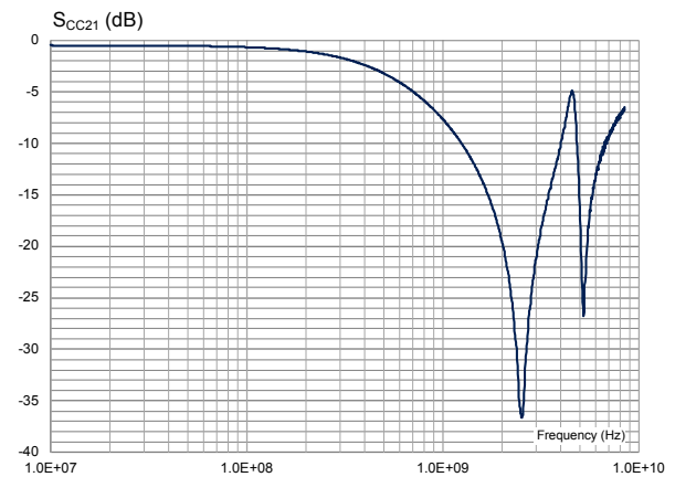
Figure 40. ECMF4-2450A60N10 common mode attenuation
