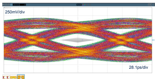
Figure 44. Eye diagram without ECMF4-2450A60N10, HDMI1.4 5.94Gbps
