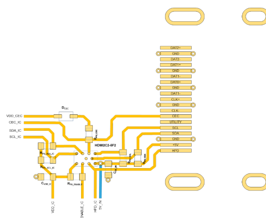
Figure 63. HDMI2C2-5F2 layout example
