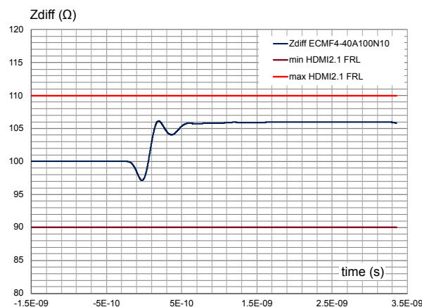
Figure 26. ECMF4-40A100N10 TDR measurements, t_r 10 %-90 % = 200 ps typical value
