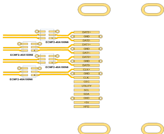
Figure 38. Layout example with 4xECMF2-40A100N6
