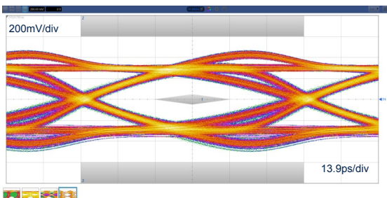
Figure 48. Eye diagram without ECMF4-2450A60N10, HDMI2.1 12Gbps worst cable
