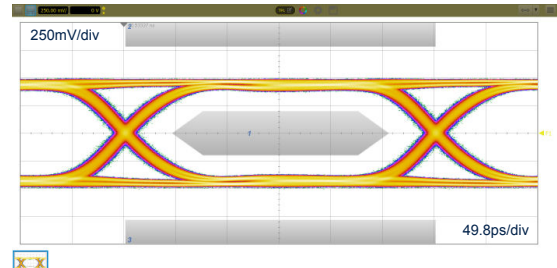
Figure 15. Eye diagram with HSP053-4M5, 3.4Gbps
