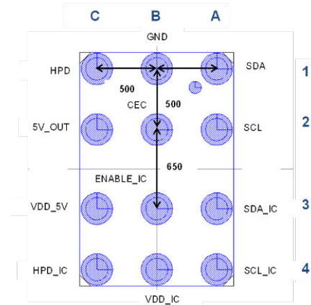
Figure 57. HDMI2C4-5F2 pinout, bump side view
