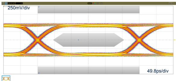
Figure 14. Eye diagram without HSP053-4M5, 3.4Gbps
