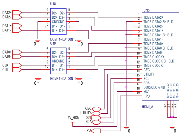
Figure 35. ECMF4-40A100N10 electrical schematic
