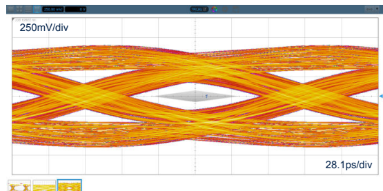
Figure 45. Eye diagram with ECMF4-2450A60N10, HDMI1.4 5.94Gbps
