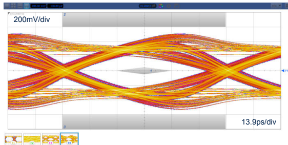
Figure 20. Eye diagram without HSP053-4M5, HDMI2.1 12Gbps worst cable
