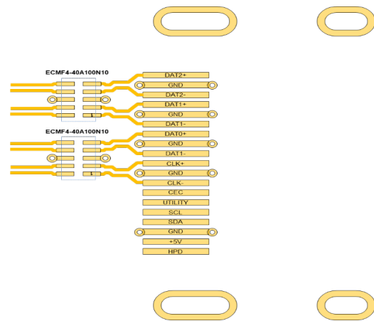
Figure 36. Layout example with 2xECMF4-40A100N10
