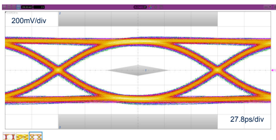
Figure 46. Eye diagram without ECMF4-2450A60N10, HDMI2.1 6Gbps
