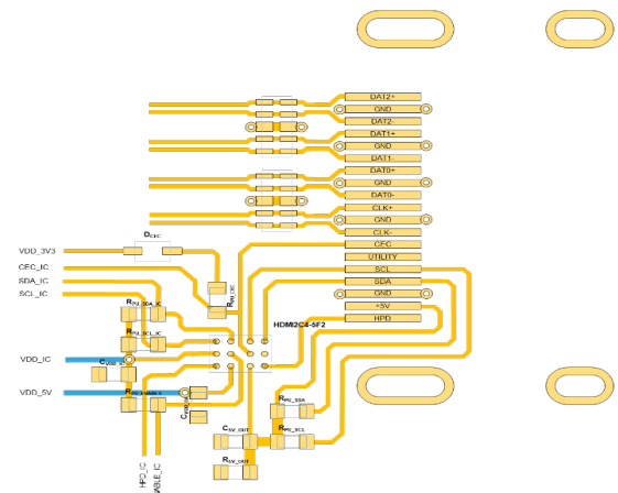
Figure 59. HDMI2C4-5F2 layout example
