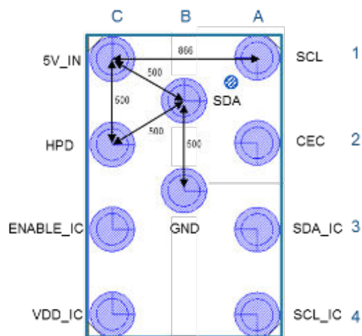
Figure 61. HDMI2C2-5F2 pinout, bump side
