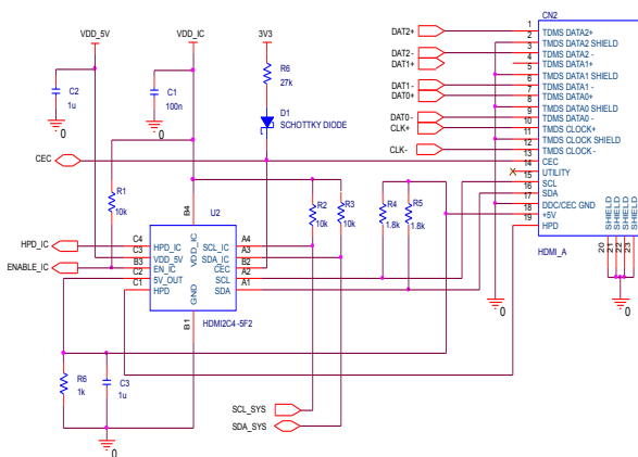
Figure 58. HDMI2C4-5F2 electrical schematic
