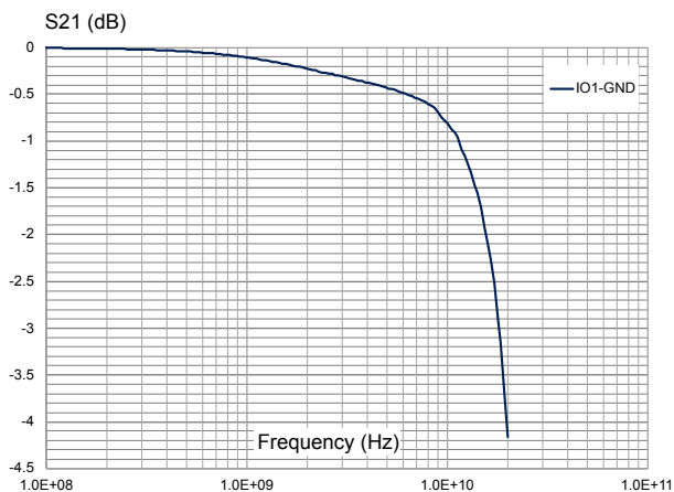
Figure 12. HSP053-4M5 attenuation
