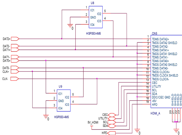
Figure 22. HSP053-4M5 electrical schematic
