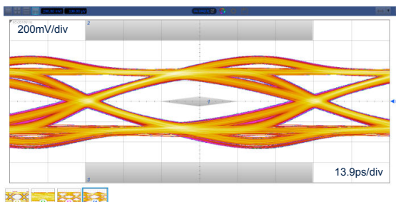
Figure 49. Eye diagram with ECMF4-2450A60N10, HDMI 2.1 12Gbps worst cable
