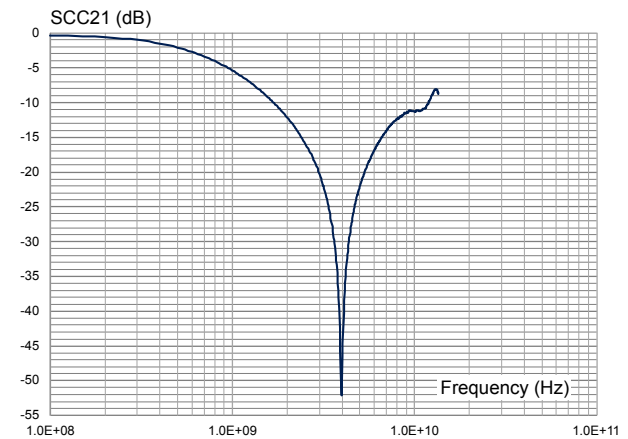
Figure 25. ECMF4-40A100N10 common mode attenuation
