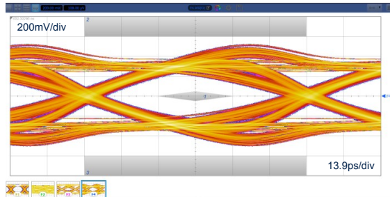
Figure 21. Eye diagram with HSP053-4M5, HDMI 2.1 12Gbps worst cable
