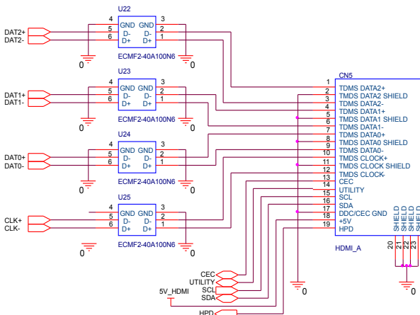
Figure 37. ECMF2-40A100N6 electrical schematic
