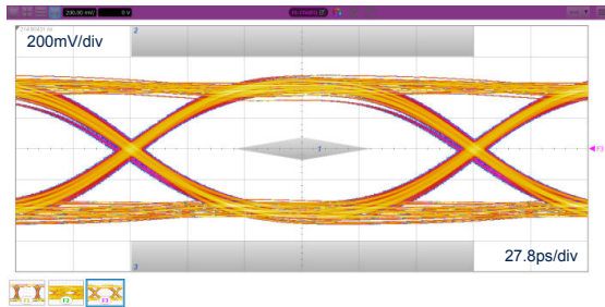
Figure 18. Eye diagram without HSP053-4M5, HDMI2.1 6Gbps
