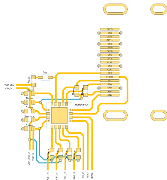
Figure 55. HDMI2C1-6C1 layout example
