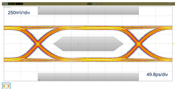
Figure 42. Eye diagram without ECMF4-2450A60N10, 3.4Gbps
