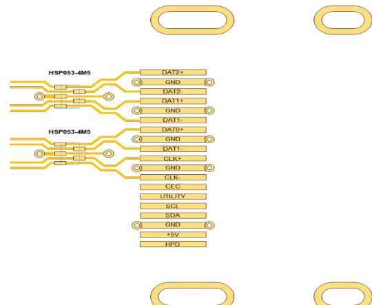
Figure 23. Layout example with 2xHSP053-4M5
