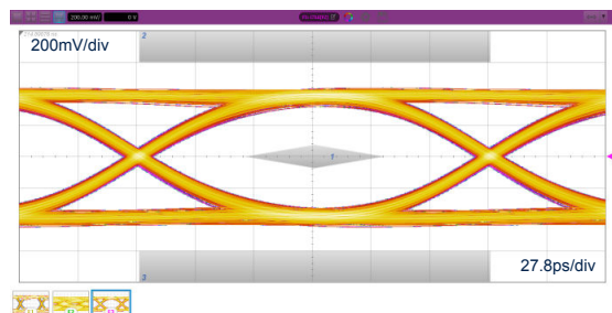
Figure 47. Eye diagram with ECMF4-2450A60N10, HDMI 2.1 6Gbps
