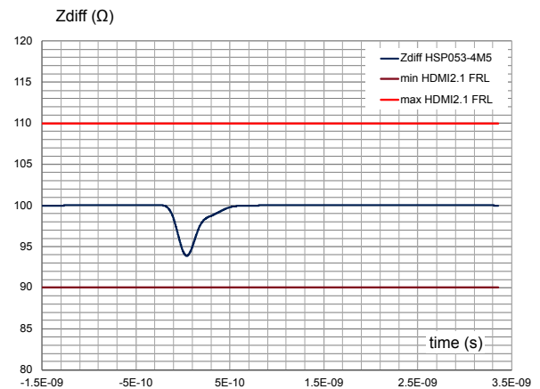
Figure 13. HSP053-4M5 TDR measurements, t_r 10 %-90 % = 200 ps typical value
