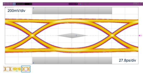
Figure 19. Eye diagram with HSP053-4M5, HDMI 2.1 6Gbps
