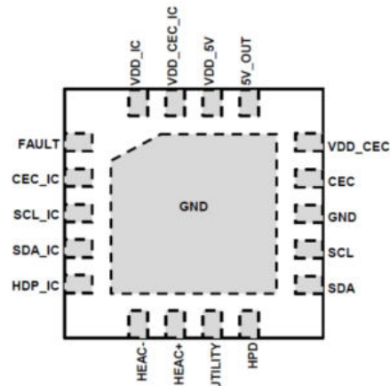
Figure 53. HDMI2C1-6C1 pin-out, top view
