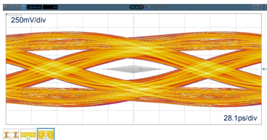
Figure 16. Eye diagram without HSP053-4M5, HDMI1.4 5.94Gbps
