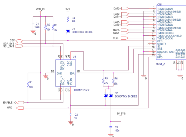
Figure 62. HDMI2C2-5F2 electrical schematic
