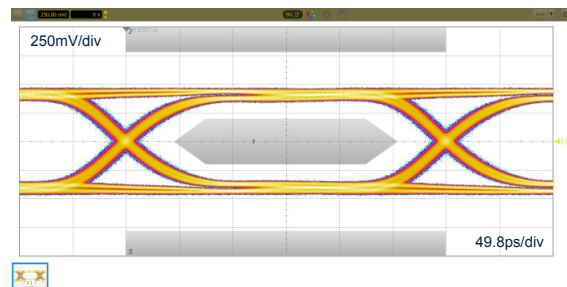
Figure 43. Eye diagram with ECMF4-2450A60N10, 3.4Gbps
