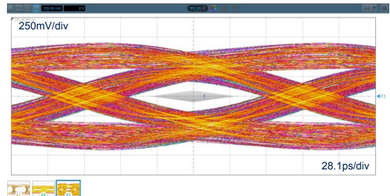
Figure 17. Eye diagram with HSP053-4M5, HDMI1.4 5.94Gbps
