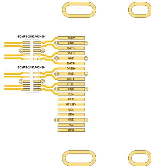
Figure 51. Layout example with 2xECMF4-2450A60N10
