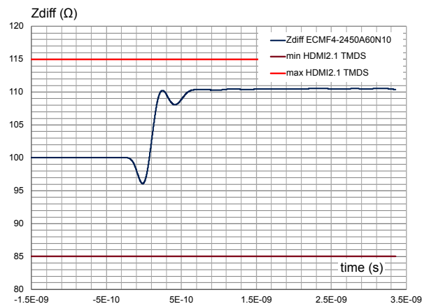
Figure 41. ECMF4-2450A60N10 TDR measurements, t_r 10 %-90 % = 200 ps typical value
