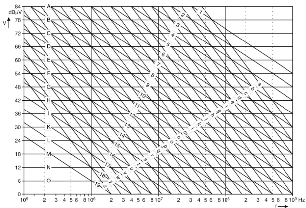
Figure 10. ST internal EMI level classification
