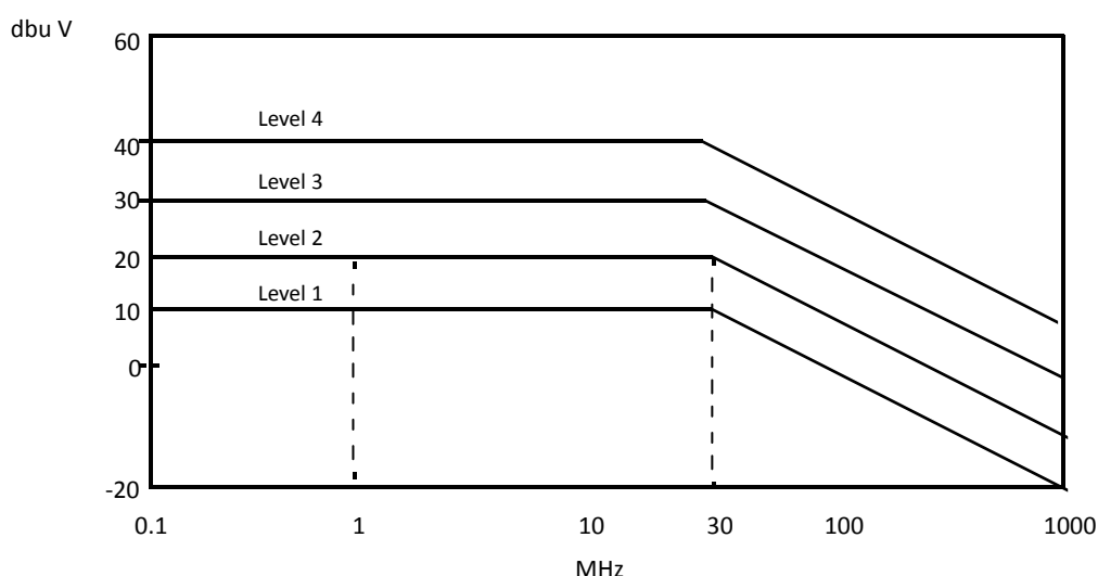
Figure 21. ST internal EMI level classification before December 14, 2015
