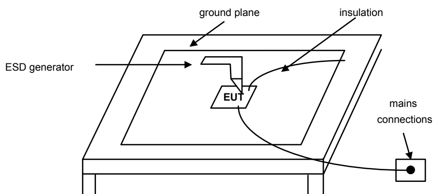
Figure 1. ESD test equipment
