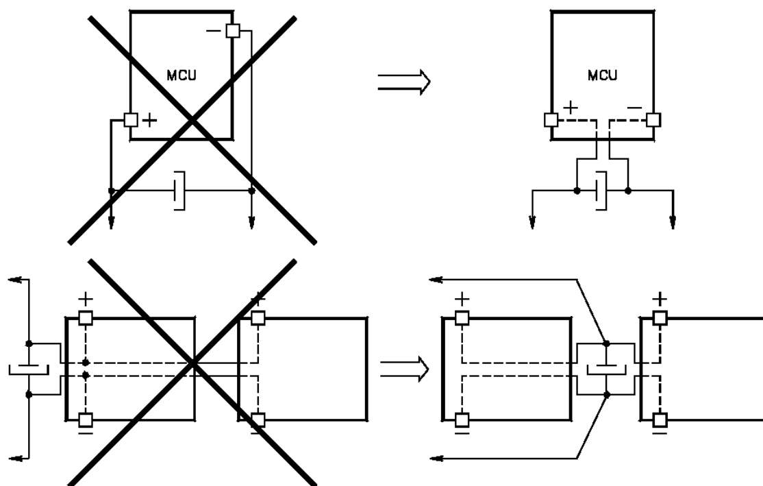
Figure 19. Power-supply layout examples
