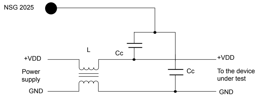
Figure 5. Coupling network
