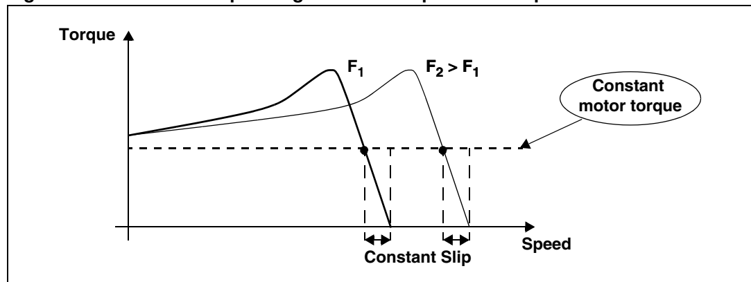
Figure 40. Controlled slip during acceleration provides torque control
