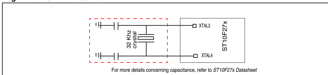
Figure 4. 32 kHz oscillator
