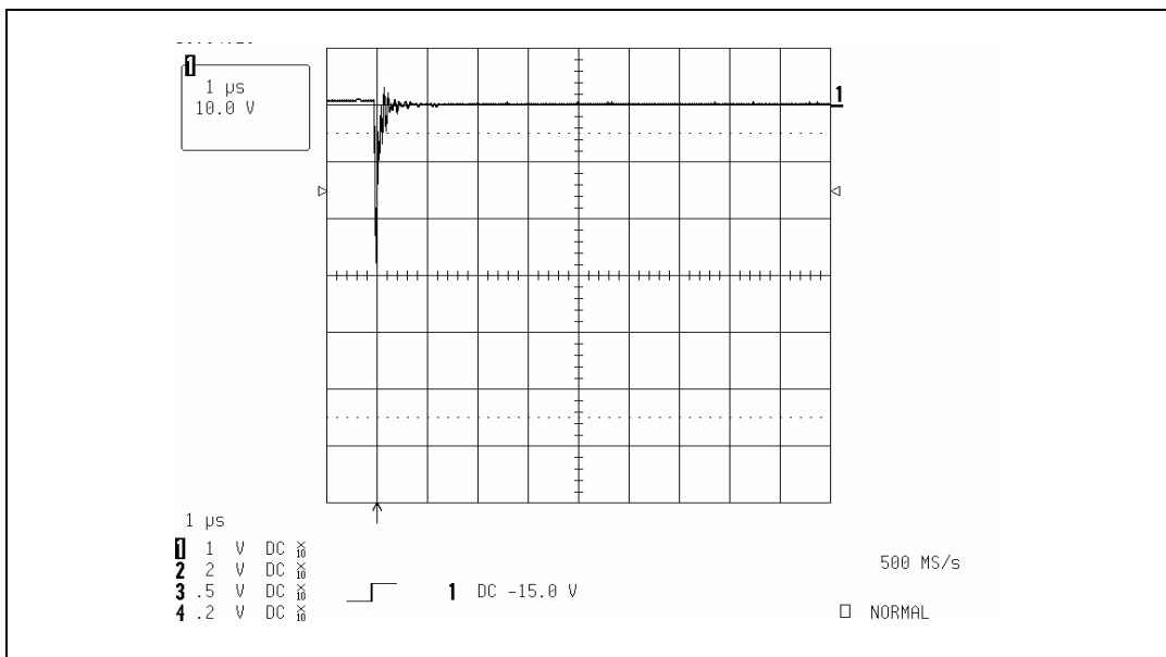
Figure 10. Remaining voltage ( V_{out} ) after an ESD pulse of -15 kV ( V_{in} ) was applied to a DVIULC6-4SC6 device
