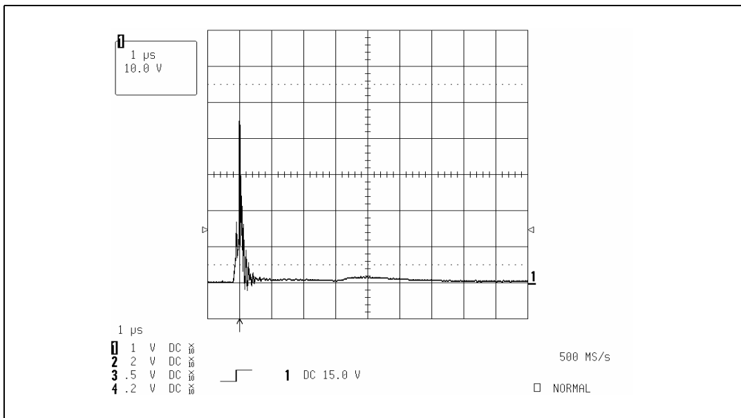
Figure 9. Remaining voltage ( V_{out} ) after an ESD pulse of +15 kV ( V_{in} ) was applied to a DVIULC6-4SC6 device
