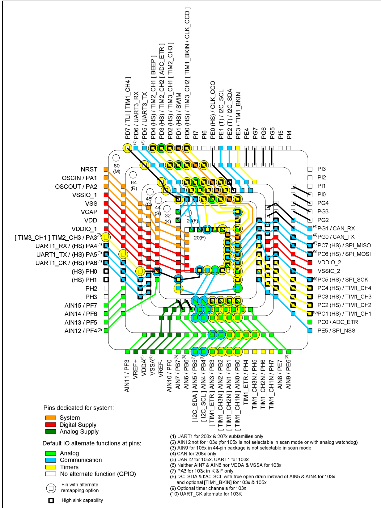
Figure 2. STM8S pinout compatibility guide from 80-pin to 20-pin packages
