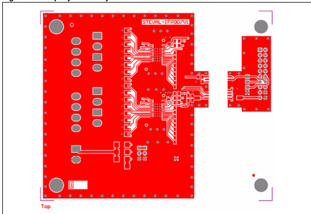
Figure 9. Top layer PCB layout
