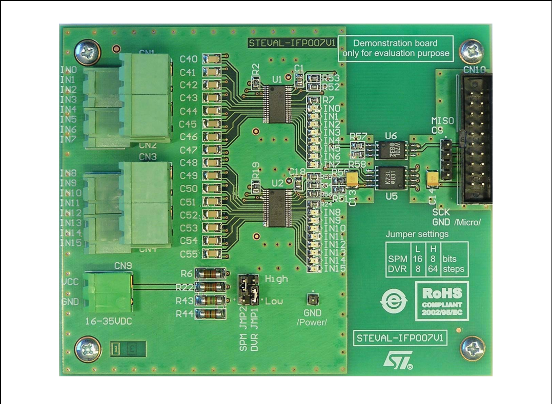
Figure 7. Demonstration board photo - top view
