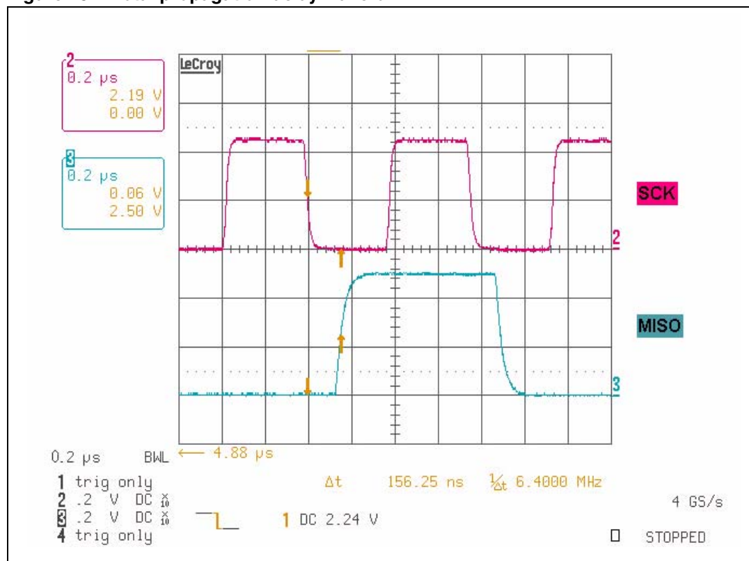
Figure 15. Total propagation delay waveform
