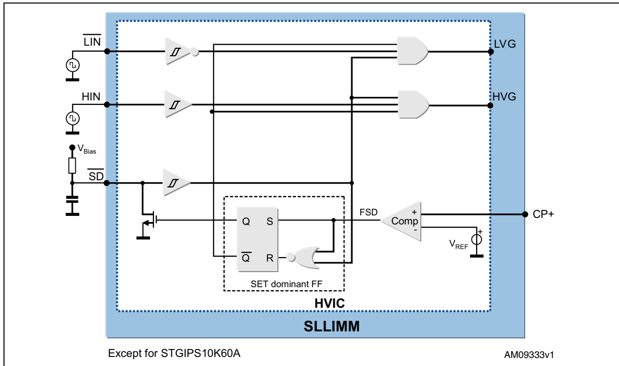
Figure 15. Smart shutdown equivalent circuitry
