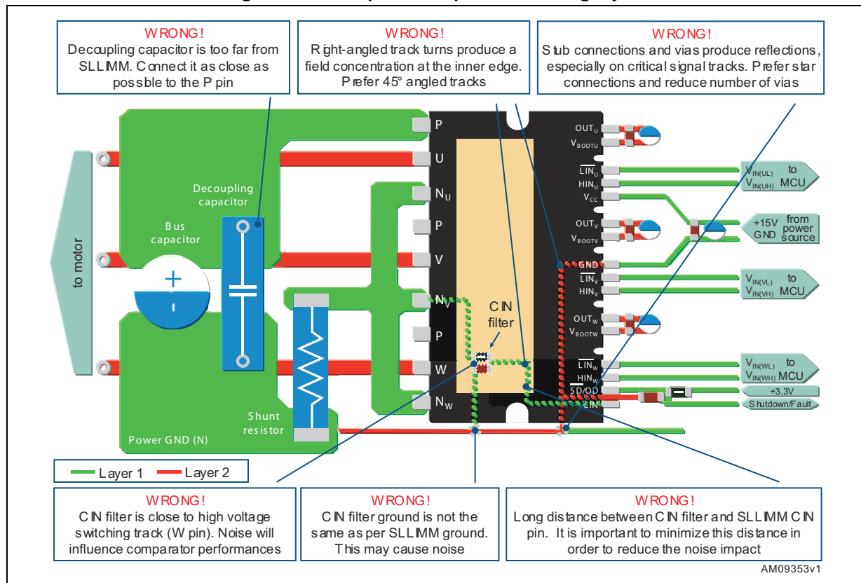
Figure 43. Example 1 of a possible wrong layout
