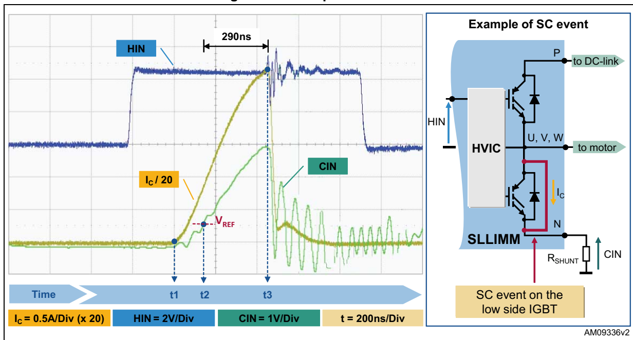
Figure 18. Example of SC event
