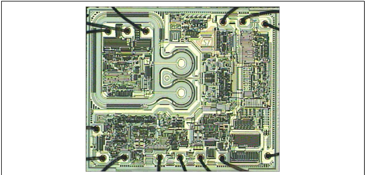
Figure 9. High voltage gate drive die image
