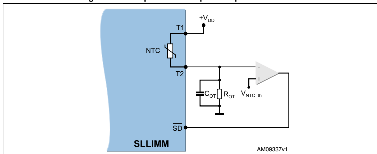
Figure 20. Example of overtemperature protection circuit
