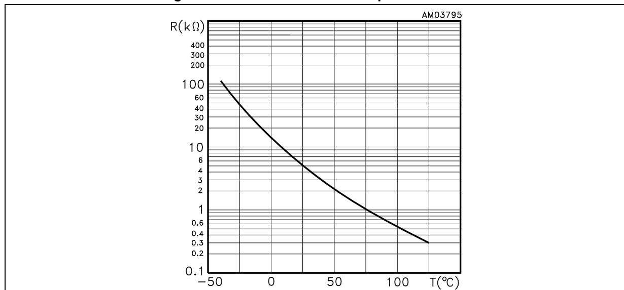
Figure 19. NTC resistance vs. temperature curve
