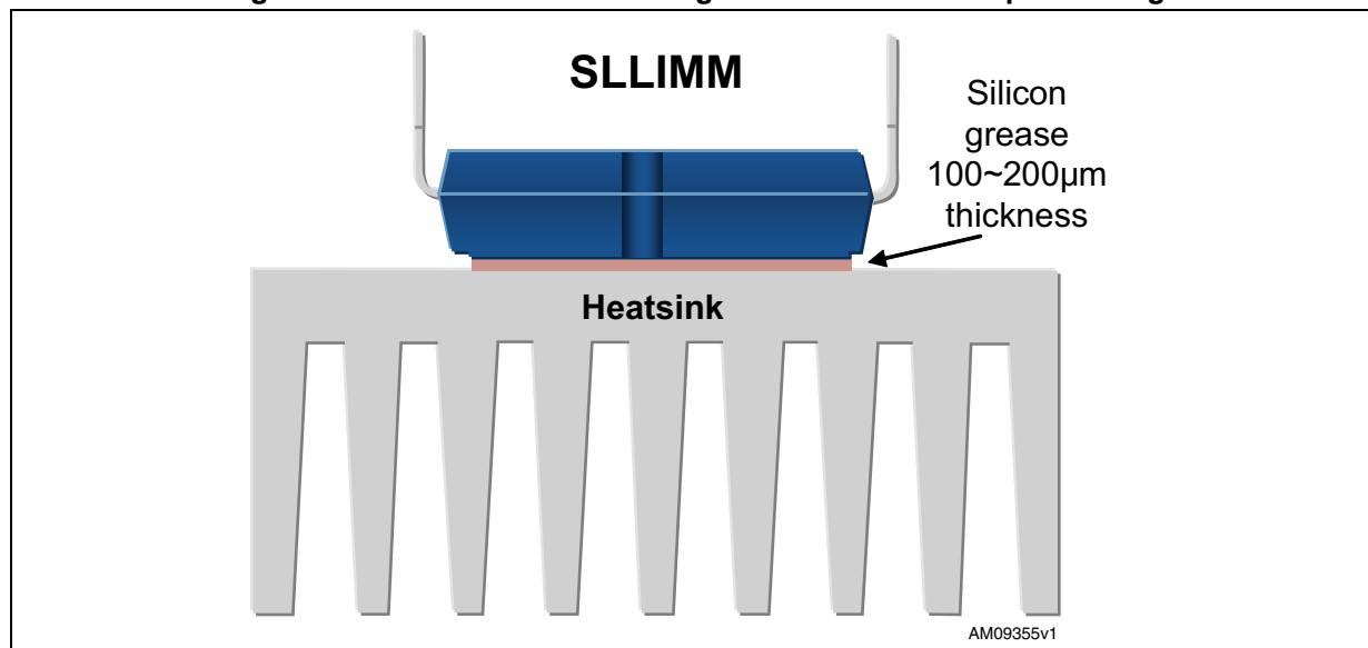
Figure 45. Recommended silicon grease thickness and positioning
