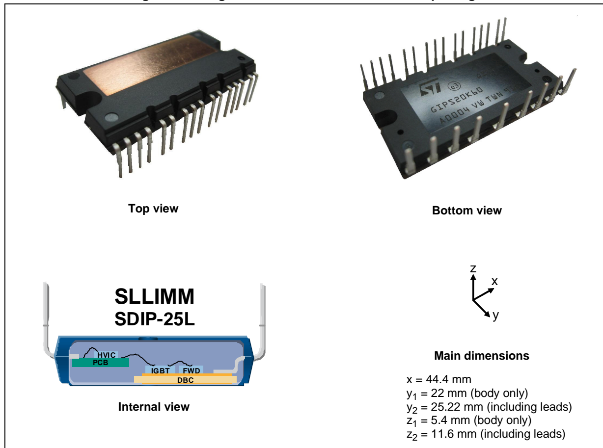
Figure 28. Images and internal view of SDIP-25L package
