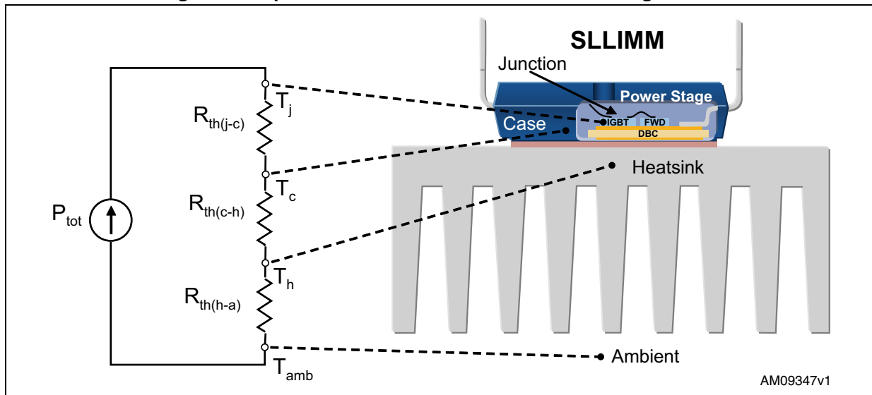
Figure 37. Equivalent thermal circuit with heatsink single IGBT
