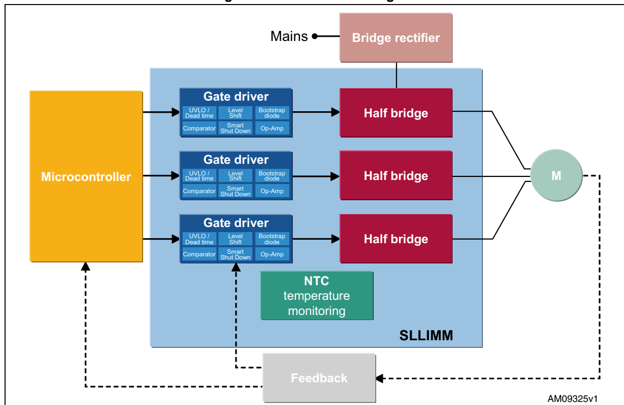
Figure 3. SLLIMM block diagram
