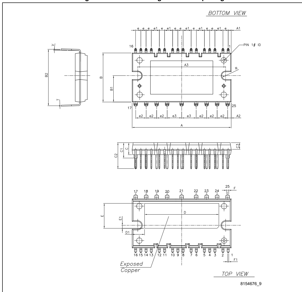
Figure 30. Outline drawing of SDIP-25L package
