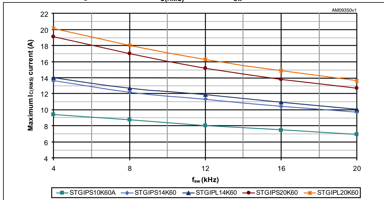
Figure 40. Maximum I_{C(RMS)} current vs. f_{sw} simulated curves
