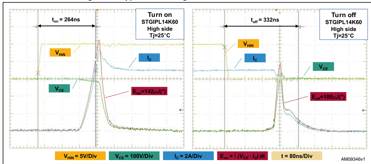
Figure 36. Typical switching waveforms of STGIPL14K60
