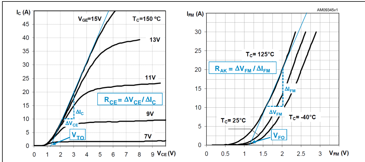
Figure 35. IGBT and diode approximation of the output characteristics
