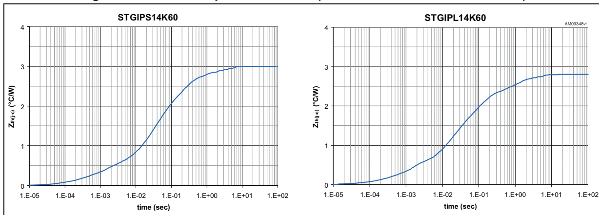
Figure 38. Thermal impedance curves (STGIPS14K60 and STGIPL14K60)
