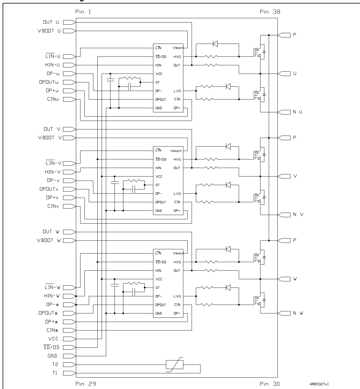
Figure 7. Internal circuit of STGIPL14K60 and STGIPL20K60
