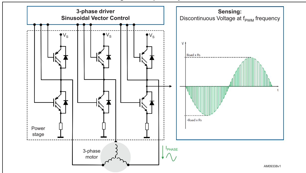
Figure 21. 3-phase system
