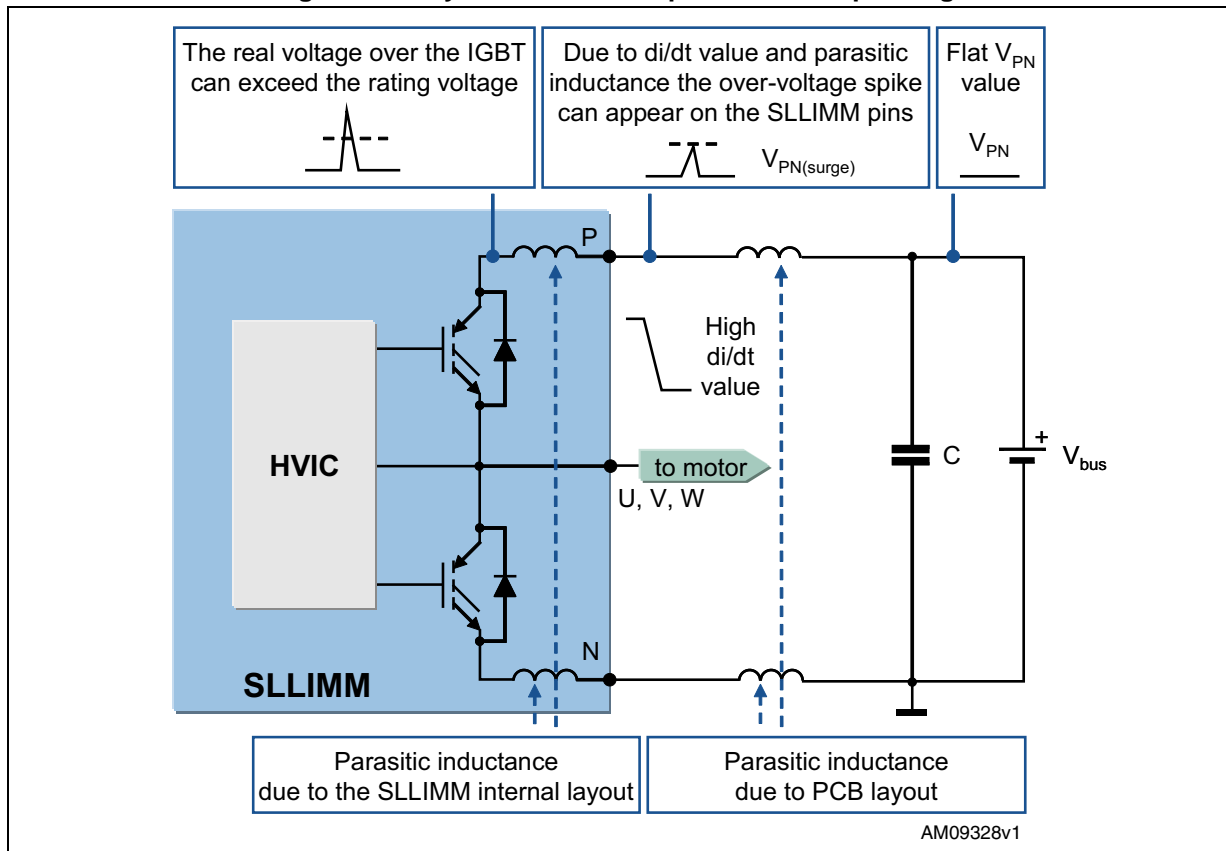
Figure 8. Stray inductance components of output stage
