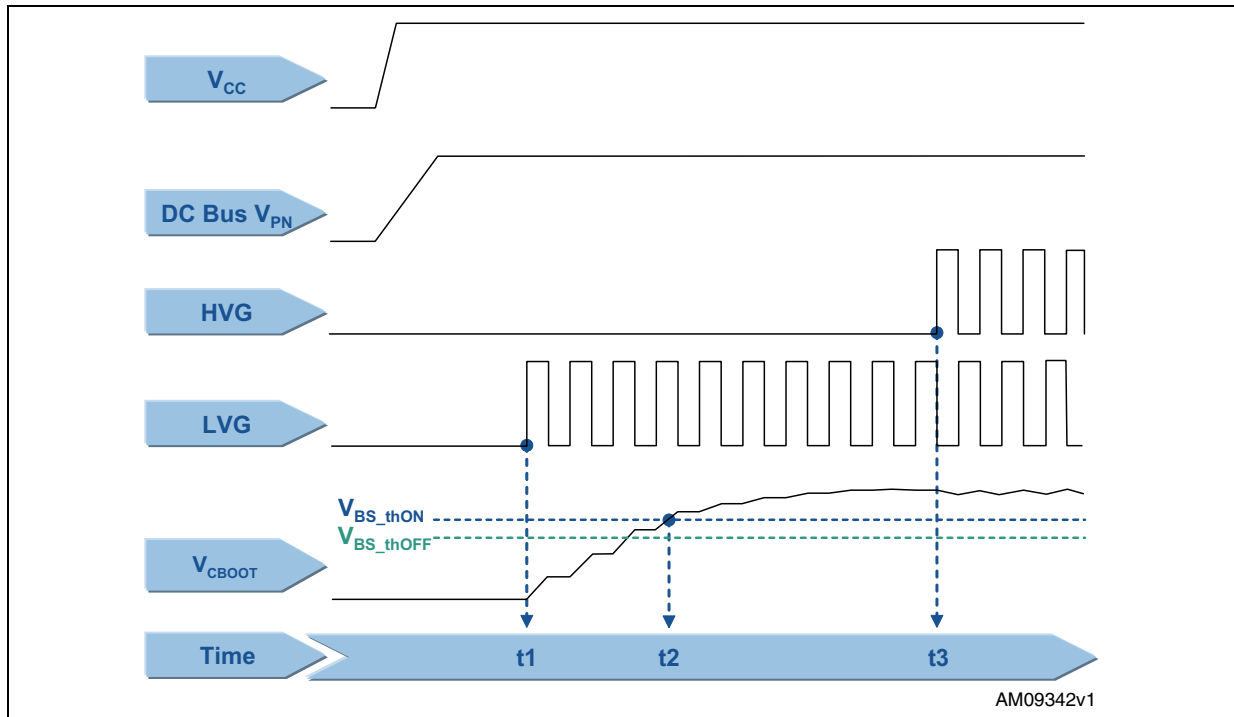
Figure 25. Initial bootstrap charging time
