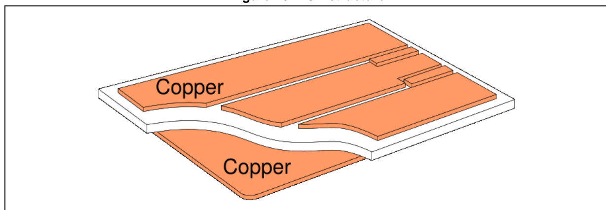
Figure 26. DCB structure
