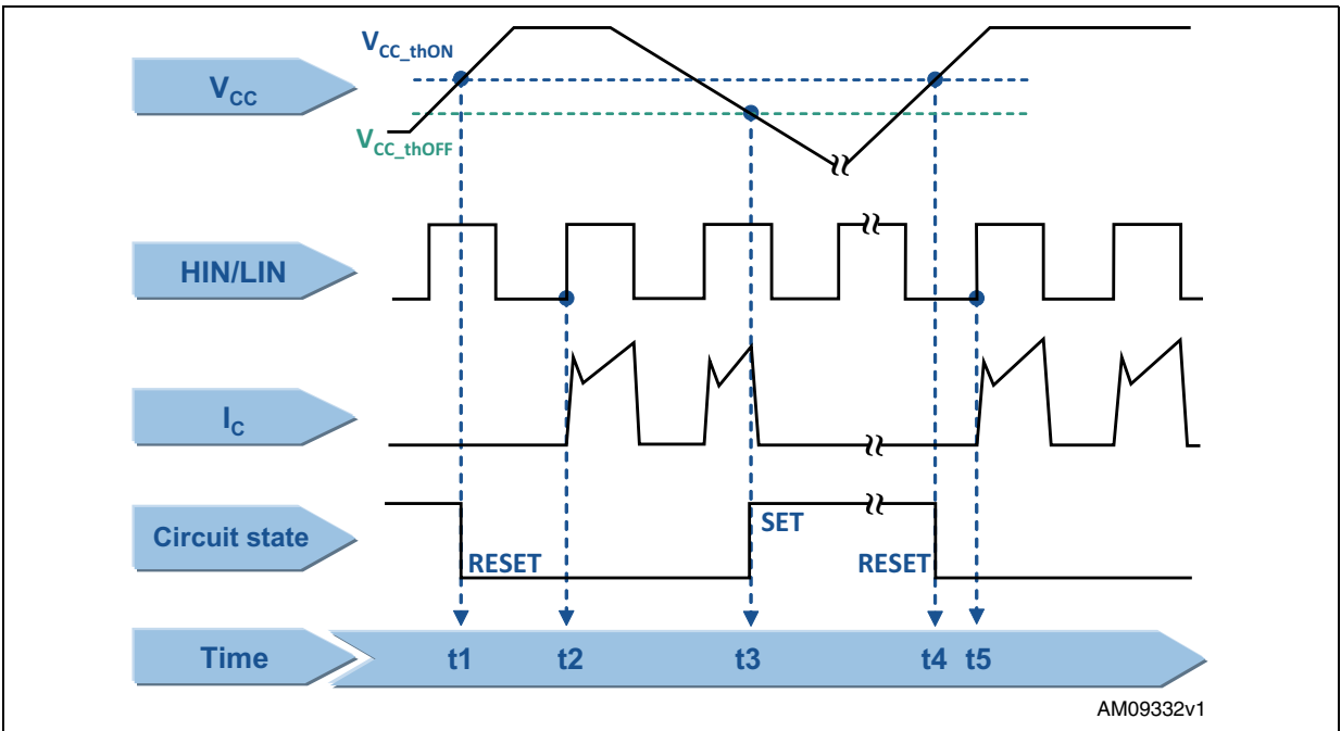
Figure 13. Timing chart of undervoltage lockout function
