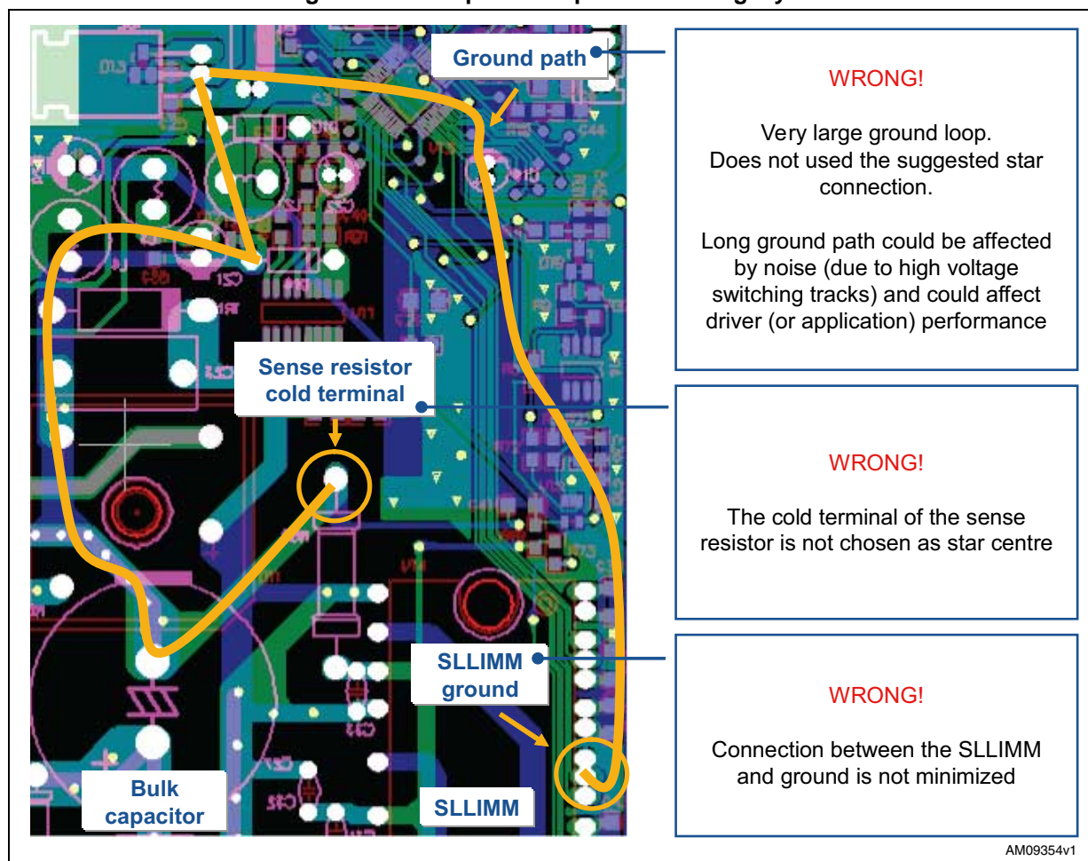
Figure 44. Example 2 of a possible wrong layout
