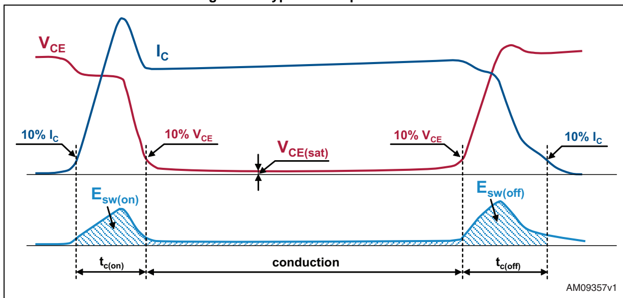
Figure 34. Typical IGBT power losses
