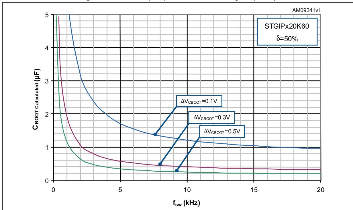
Figure 24. Bootstrap capacitor vs. switching frequency
