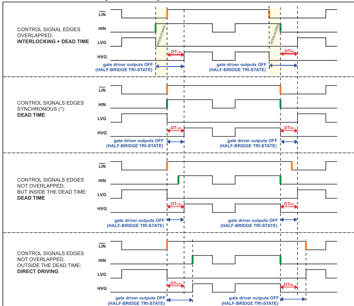
Figure 14. Timing chart of dead time function
