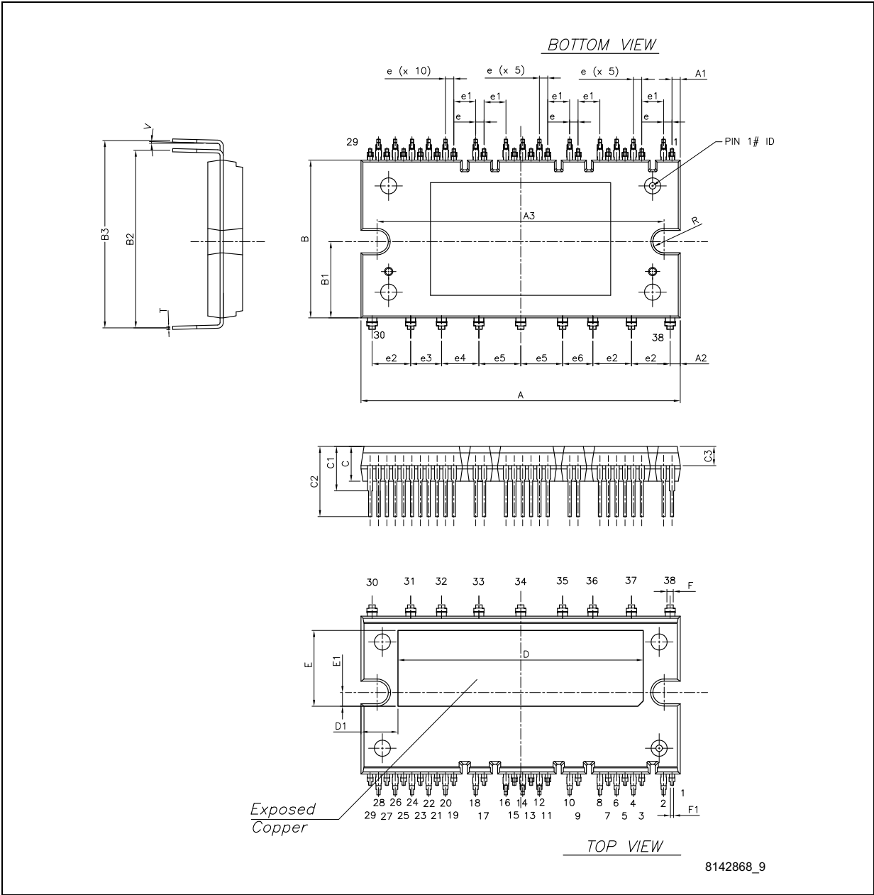
Figure 31. Outline drawing of SDIP-38L package
