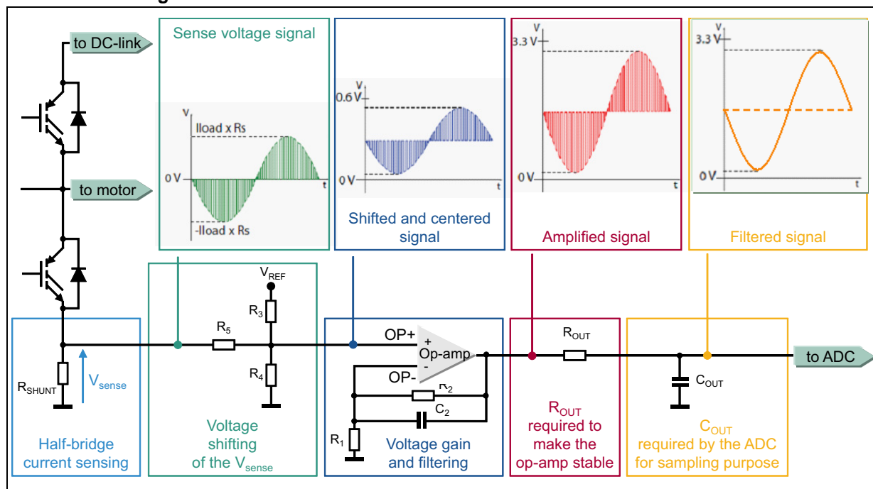
Figure 22. General advanced current sense scheme and waveforms
