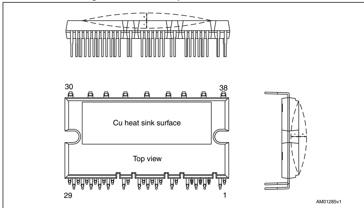
Figure 46. Measurement point of Cu heatsink flatness
