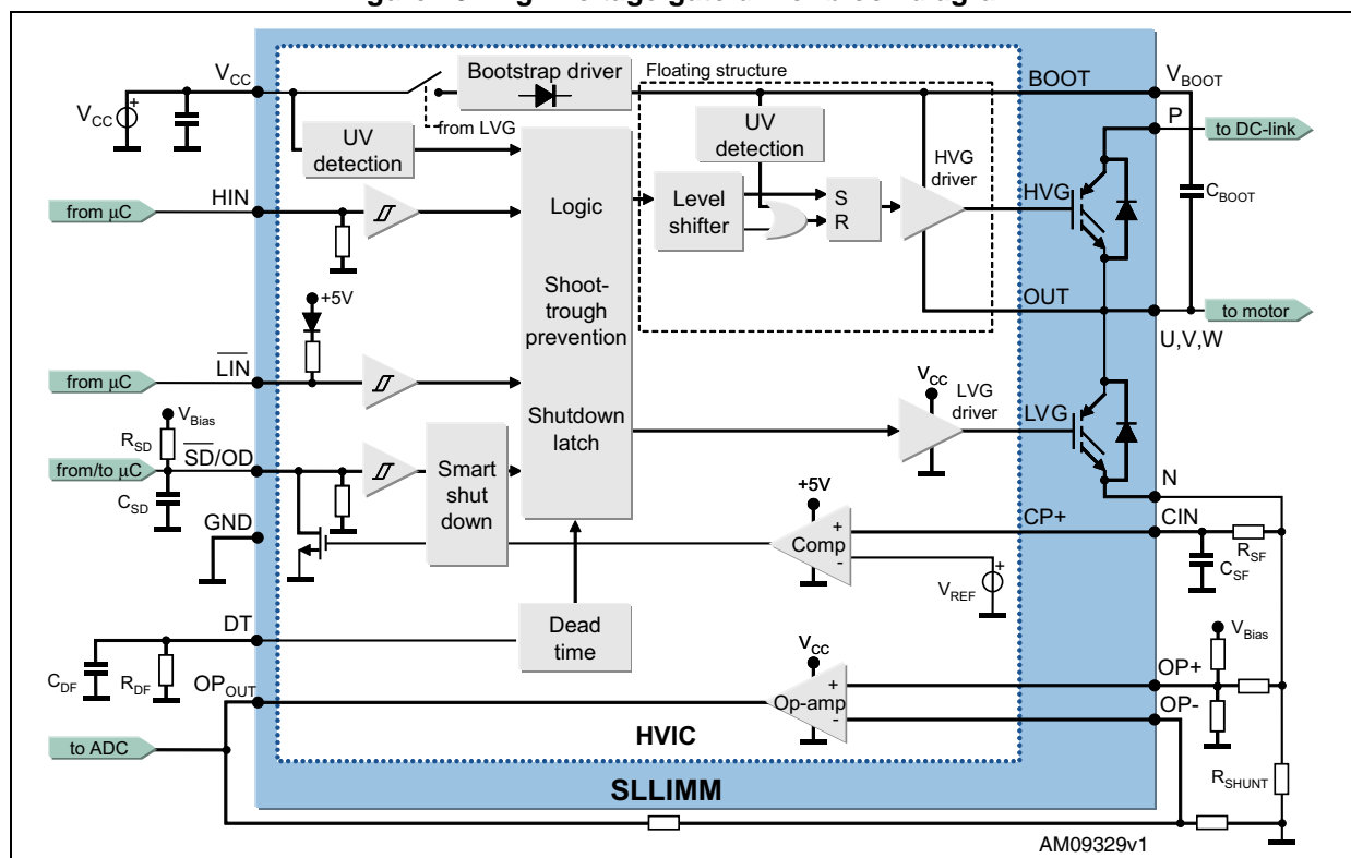
Figure 10. High voltage gate driver block diagram
