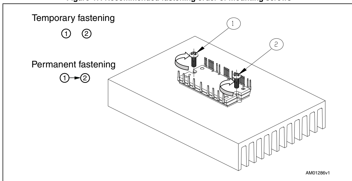
Figure 47. Recommended fastening order of mounting screws
