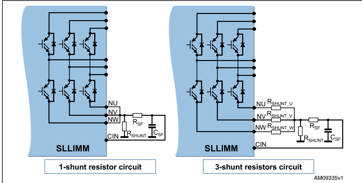
Figure 17. Examples of SC protection circuit
