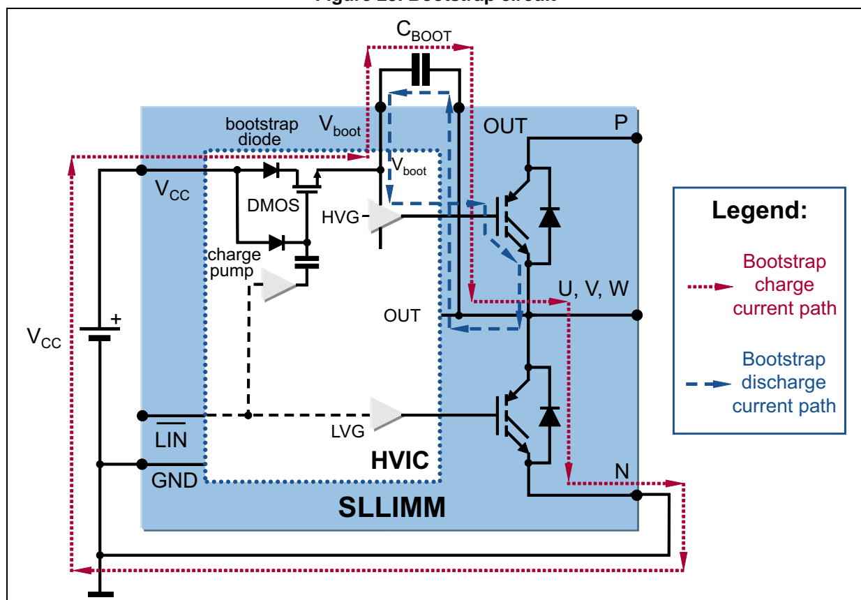
Figure 23. Bootstrap circuit
