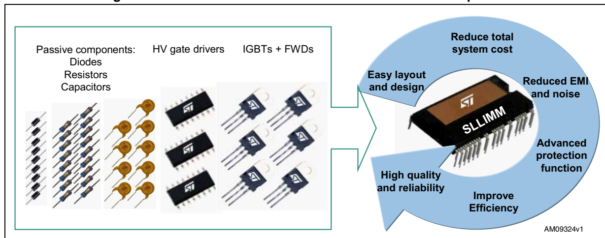
Figure 2. Discrete-based inverter vs. SLLIMM solution comparison
