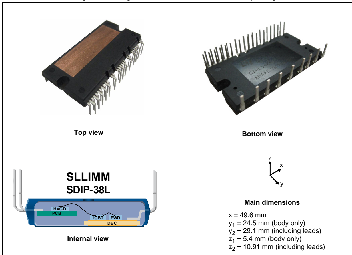
Figure 29. Images and internal view of SDIP-38L package
