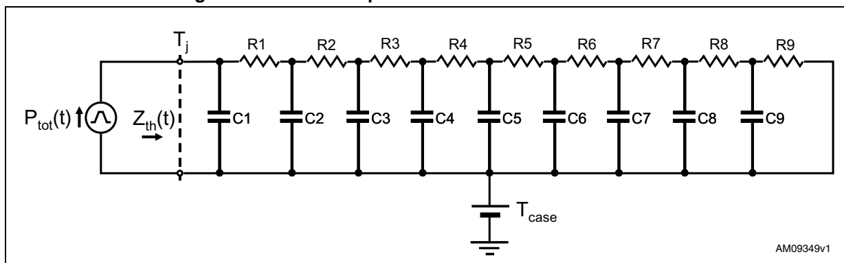
Figure 39. Thermal impedance RC Cauer thermal network
