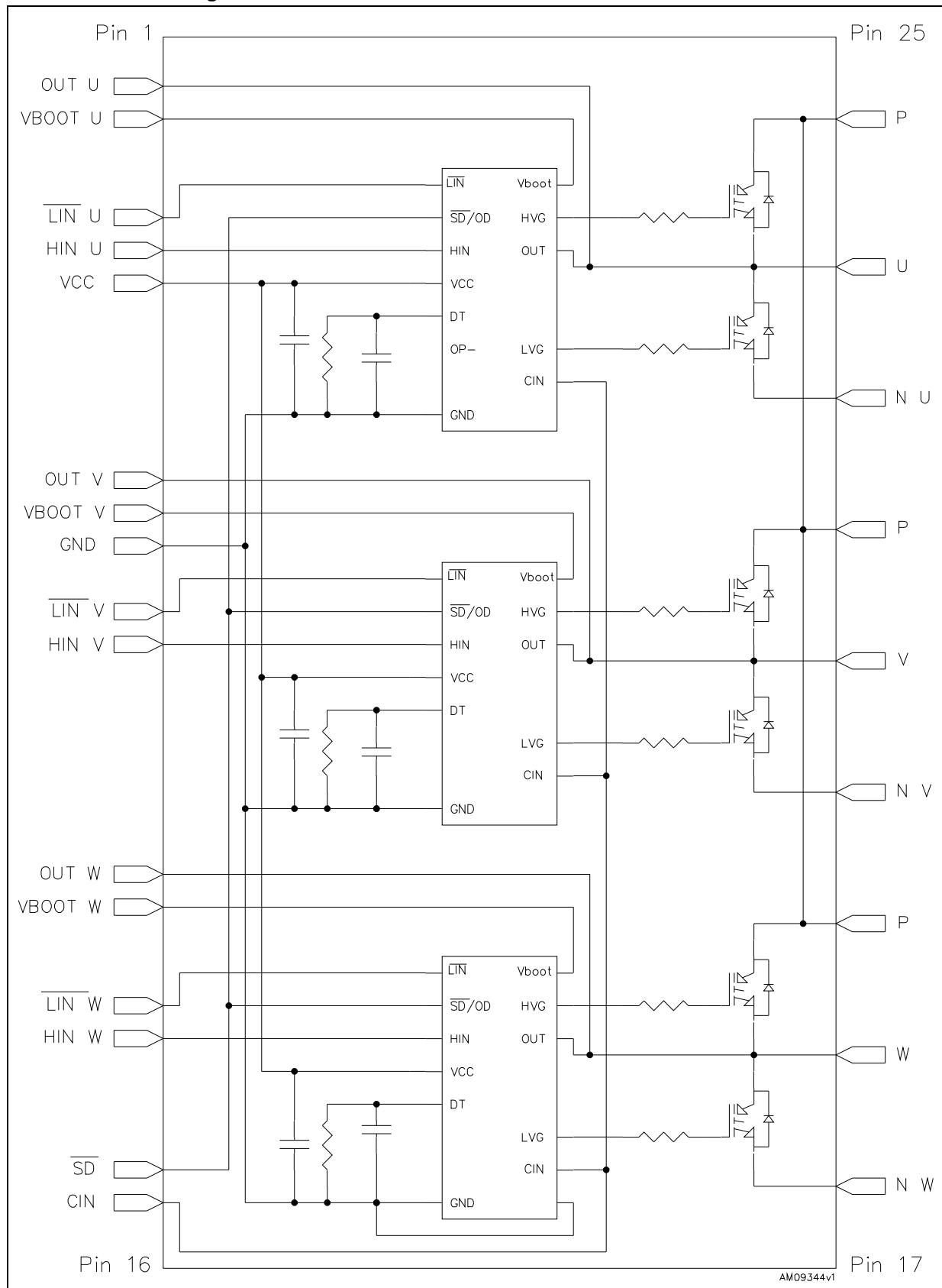
Figure 6. Internal circuit of STGIPS14K60 and STGIPS20K60
