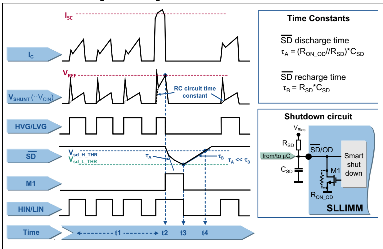
Figure 16. Timing chart of smart shutdown function
