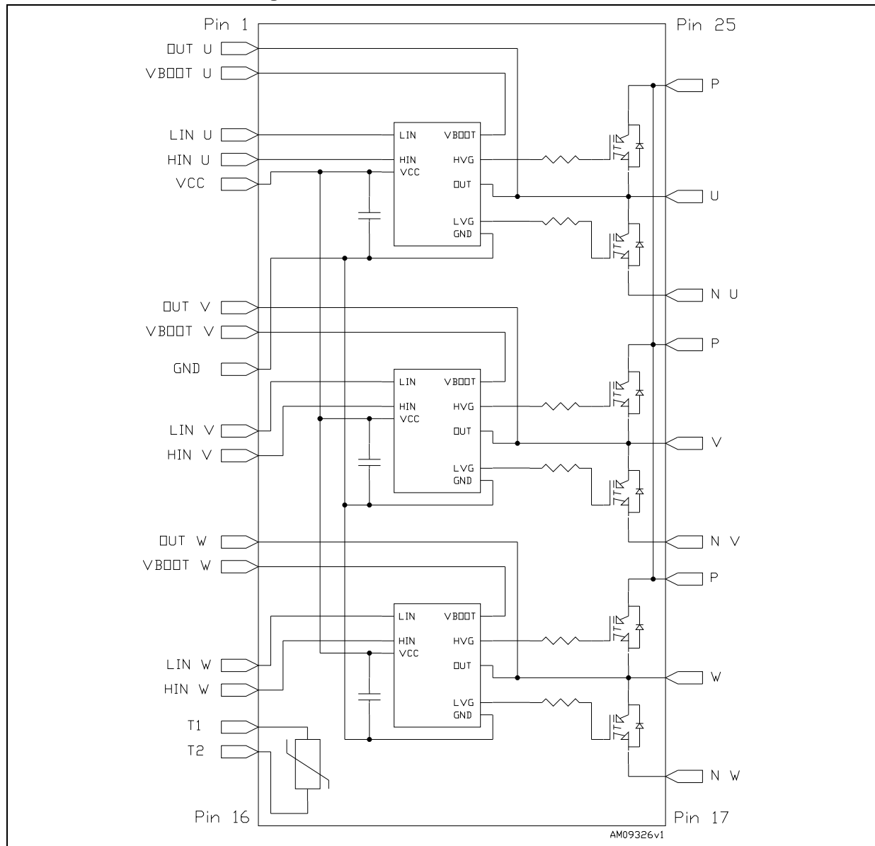
Figure 5. Internal circuit of STGIPS10K60A
