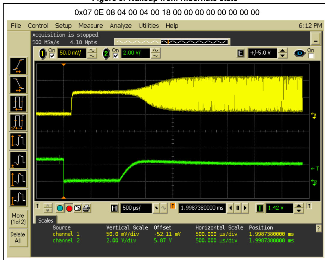
Figure 3. Wakeup from Hibernate state
