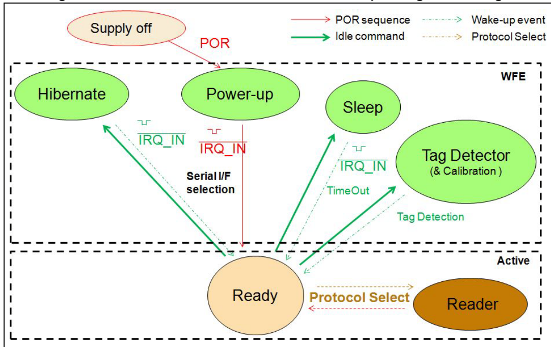
Figure 1. ST25R95 and CR95HF initialization and operating state change
