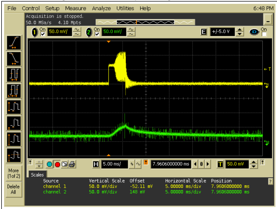
Figure 7. Power consumption in tag detection mode
