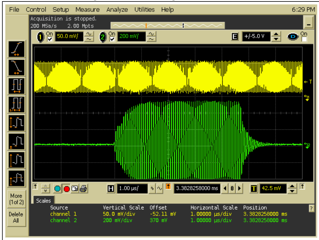
Figure 6. RF burst in tag detection mode
