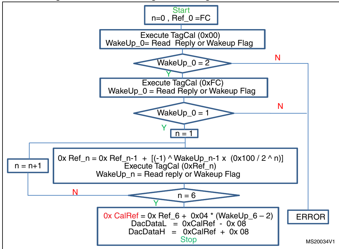
Figure 11. dichotomous algorithm for tag detection calibration
