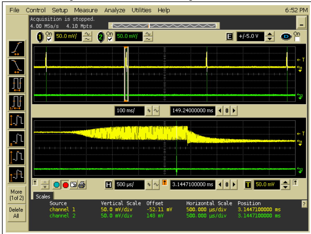
Figure 5. Restart of resources in tag detection mode
