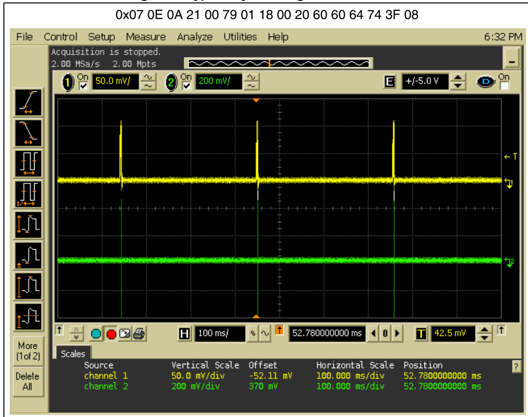
Figure 4. Typical cycle in tag detection mode
