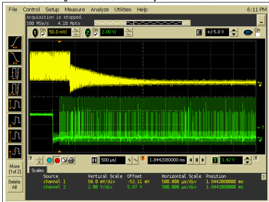
Figure 2. Transition from Ready to Hibernate state
