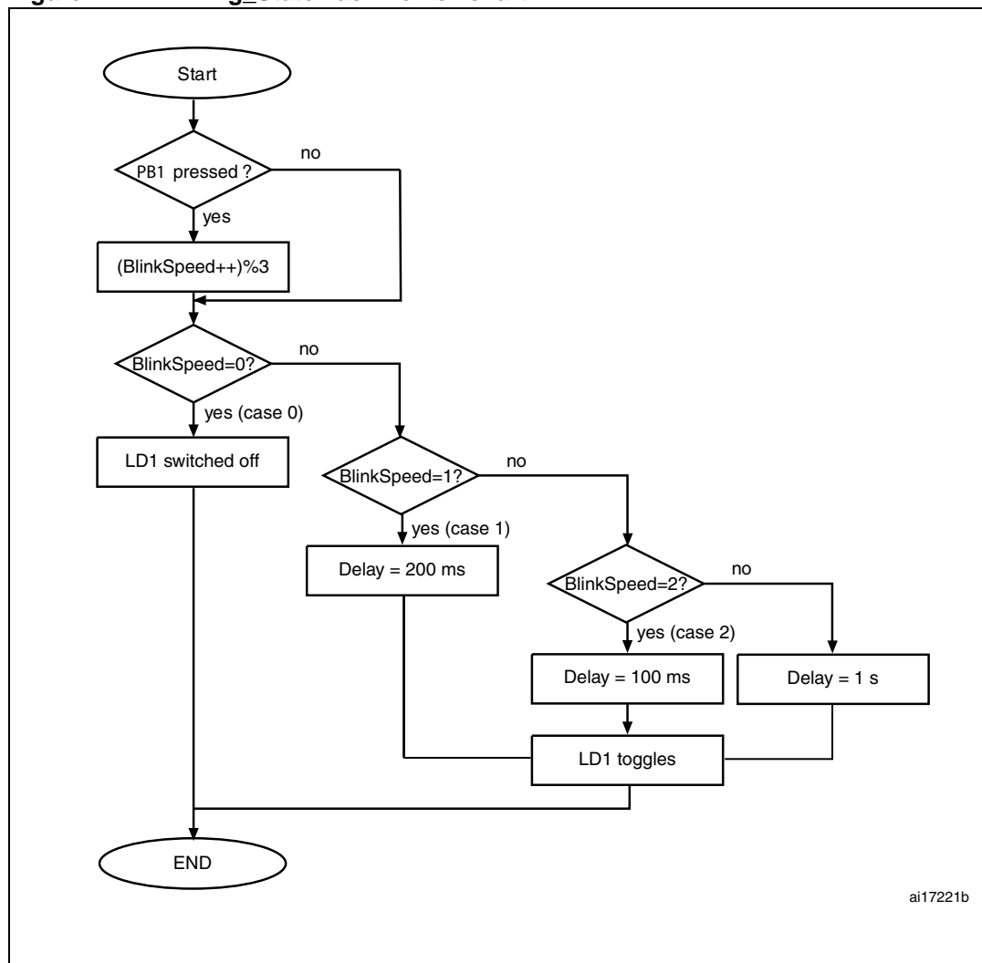
Figure 2. Blinking_StateMachine flowchart
