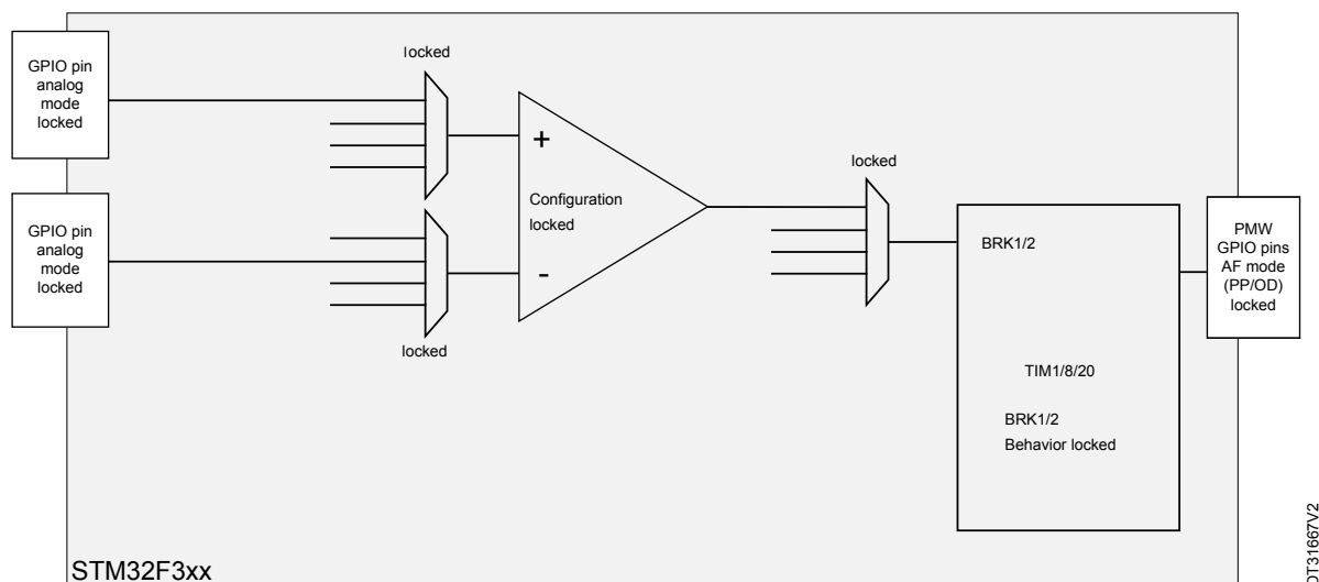
Figure 13. Comparator chain configuration locking
