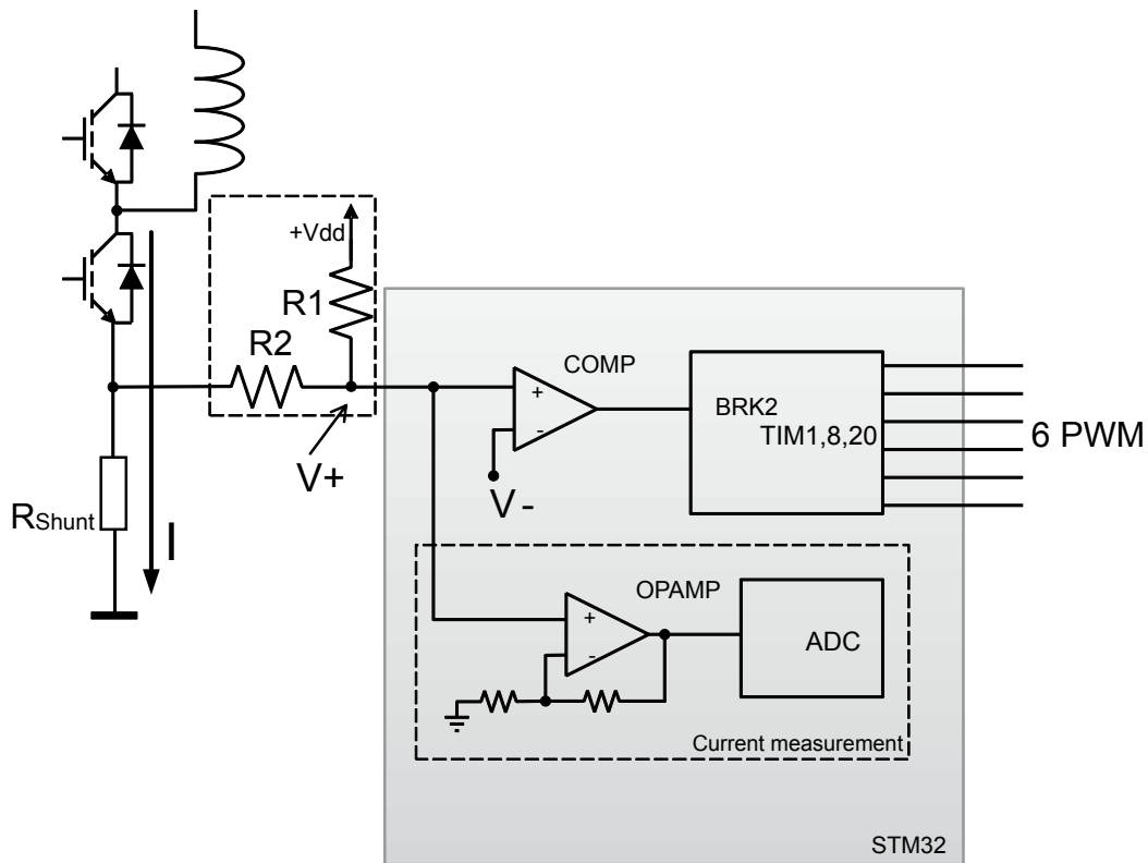
Figure 11. Overvoltage protection network block diagram
