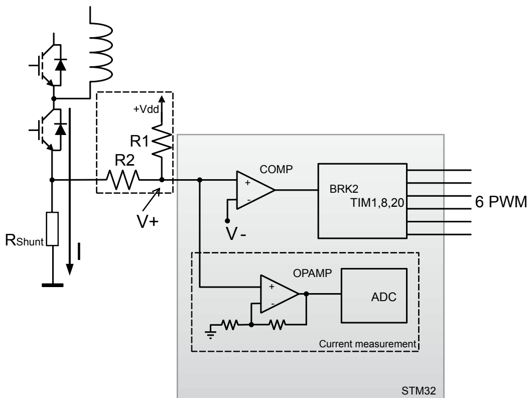
Figure 10. Overcurrent protection network implementation block diagram
