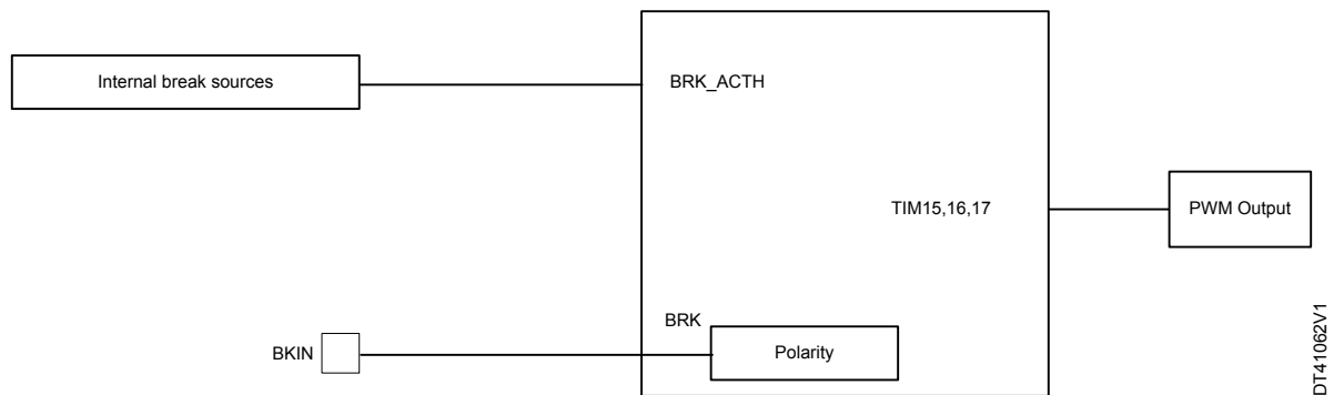
Figure 7. Break feature implementation for TIM15, TIM16, and TIM17 for STM32F3 series devices
