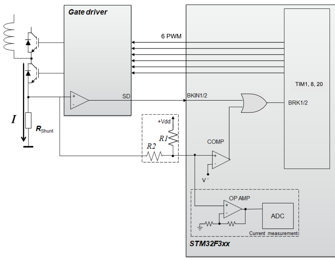
Figure 12. Combining external and internal protection concept
