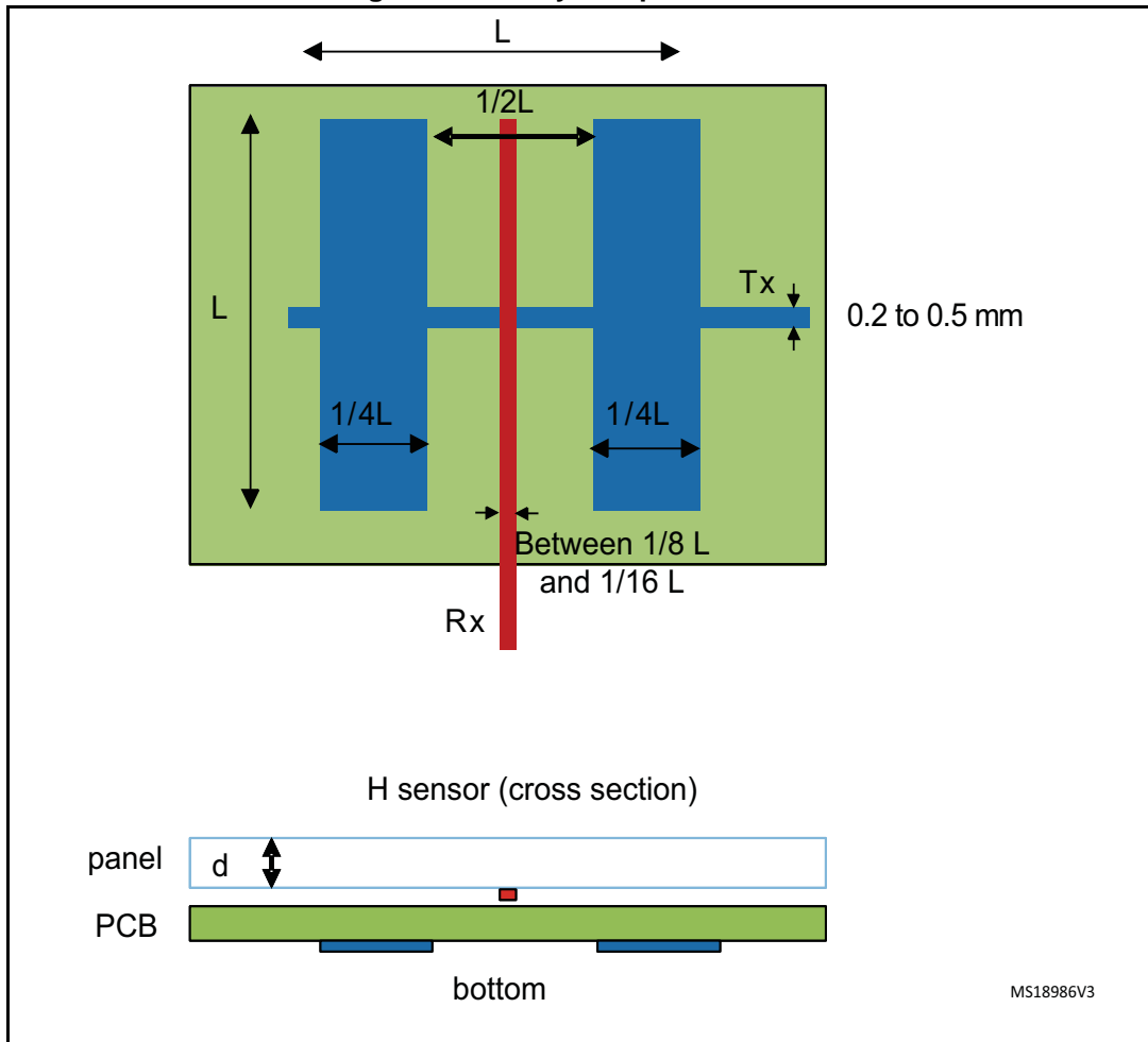
Figure 4. Two-layer implementation
