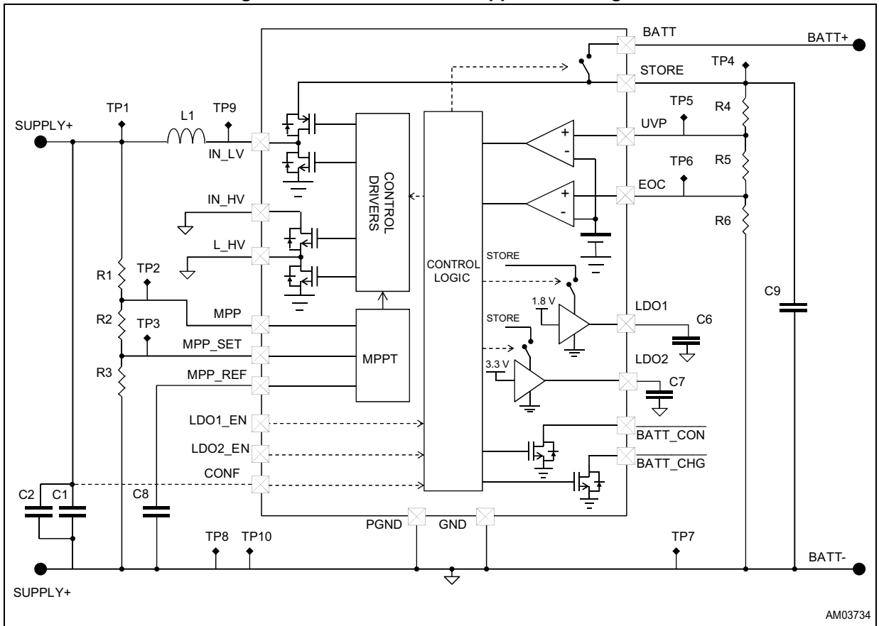
Figure 3. STEVAL-ISV019V1 application diagram
