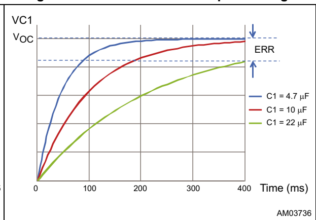
Figure 11. Effect of C1 on sampled voltage
