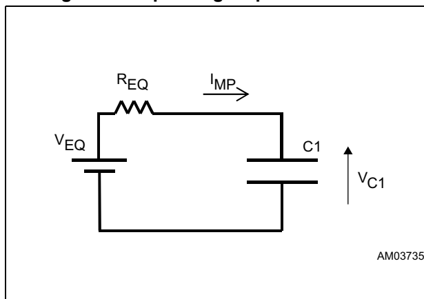
Figure 10. Input stage equivalent circuit
