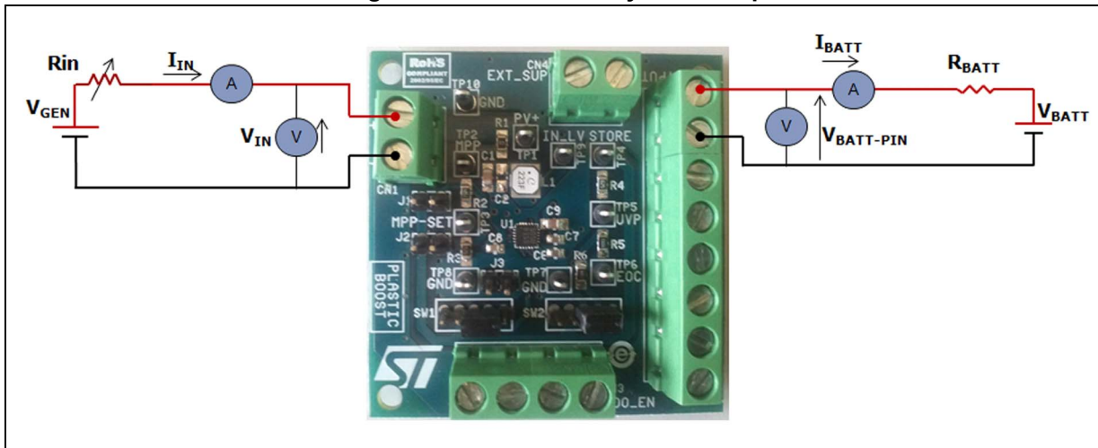
Figure 4. Measurement system setup
