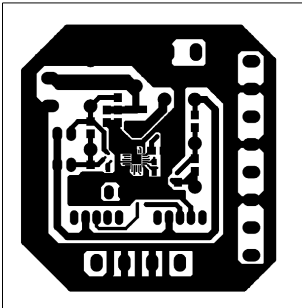
Figure 6. Layout - top view
