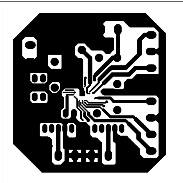
Figure 7. Layout - bottom view
