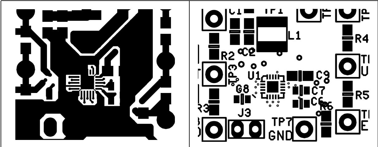
Figure 8. Ground plane detail
