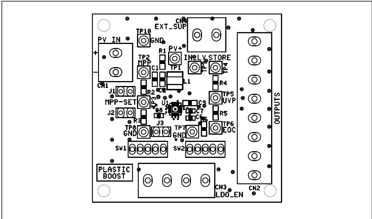
Figure 6. Layout - top view
