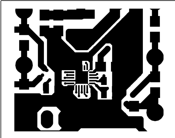
Figure 8. Ground plane detail
