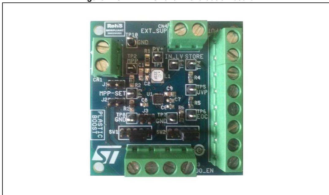
Figure 1. STEVAL-ISV019V1 evaluation board
