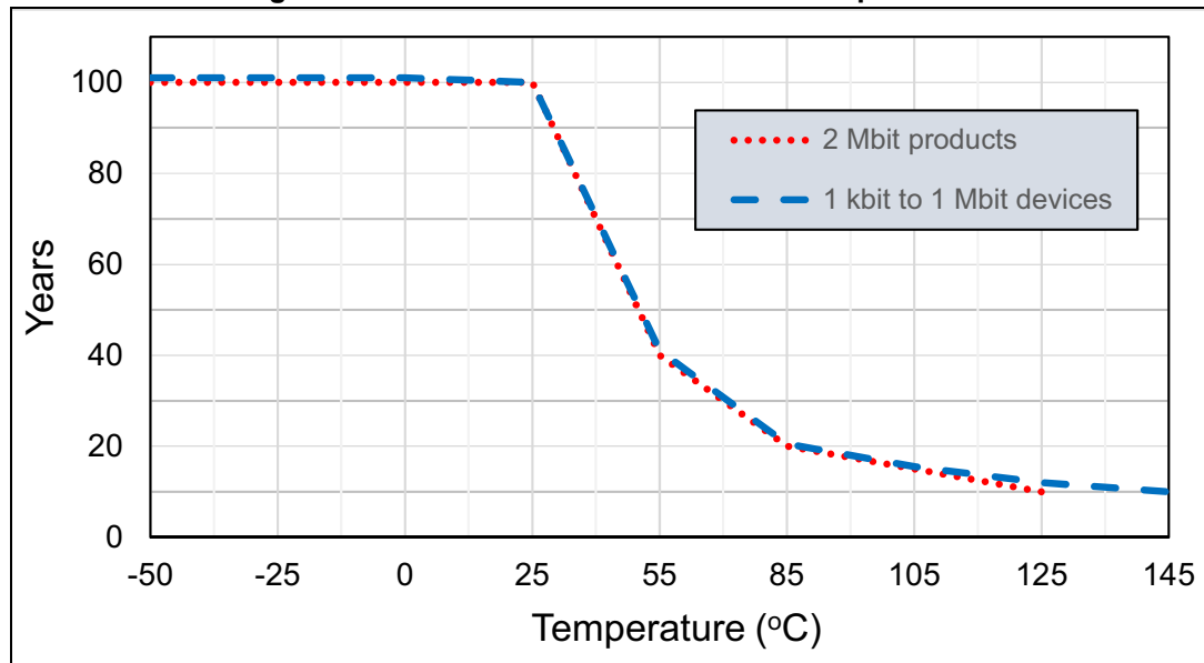
Figure 2. Years of data retention versus temperature
