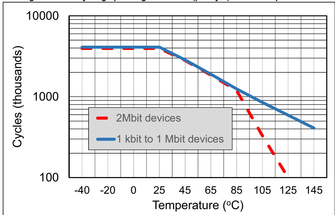
Figure 1. Safe cycling operating conditions (per byte) versus temperature (1)
