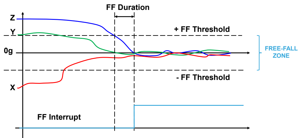
Figure 5. Free-fall interrupt
