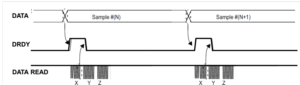
Figure 4. Data-ready signal
