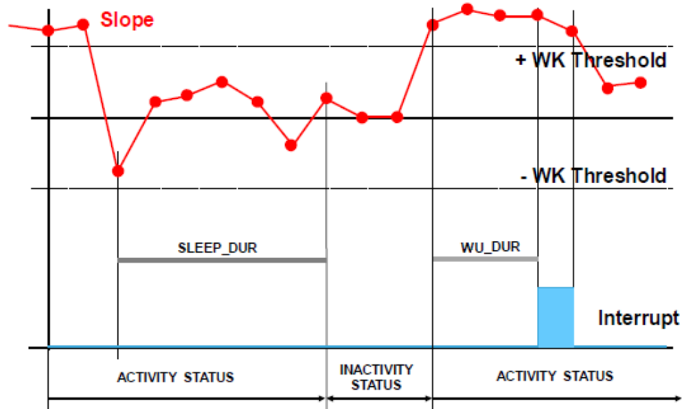
Figure 11. Activity/Inactivity recognition
