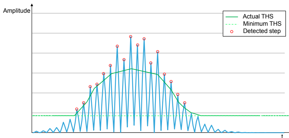
Figure 12. Minimum threshold
