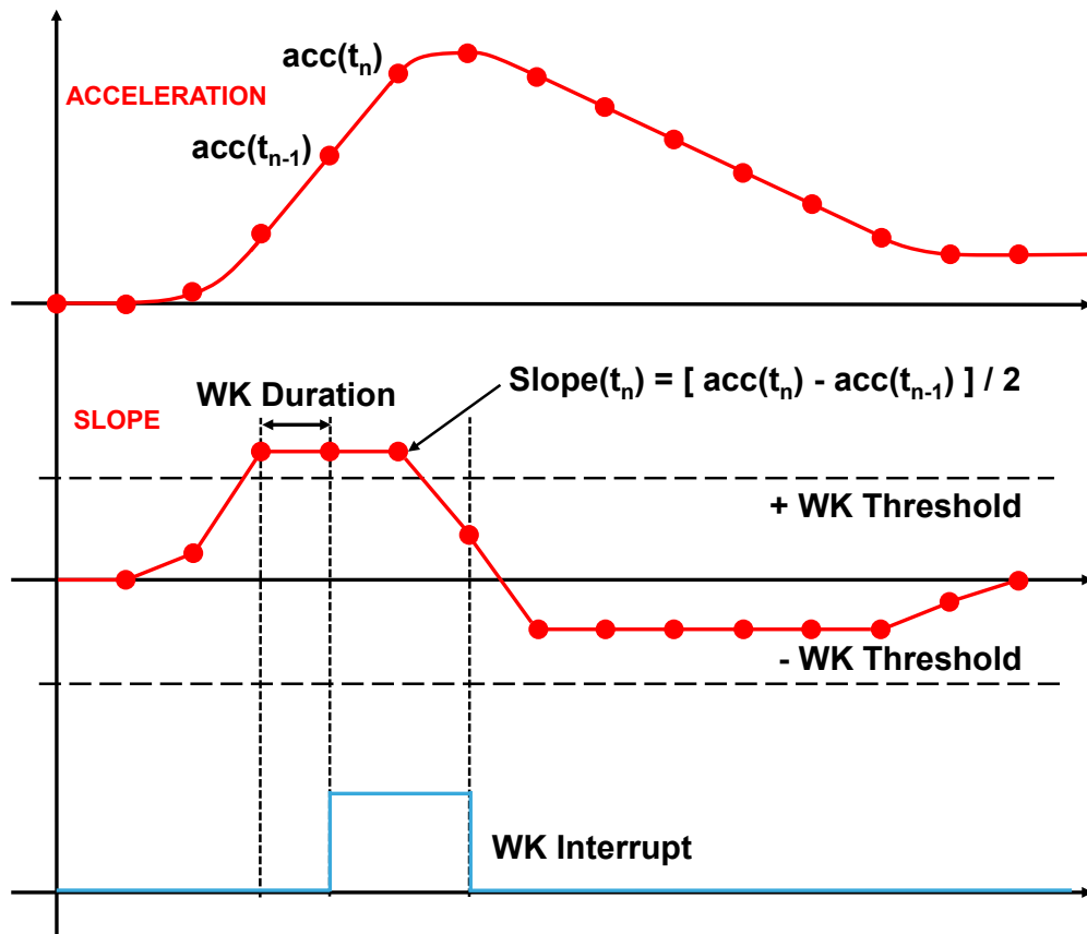
Figure 6. Wake-up interrupt
