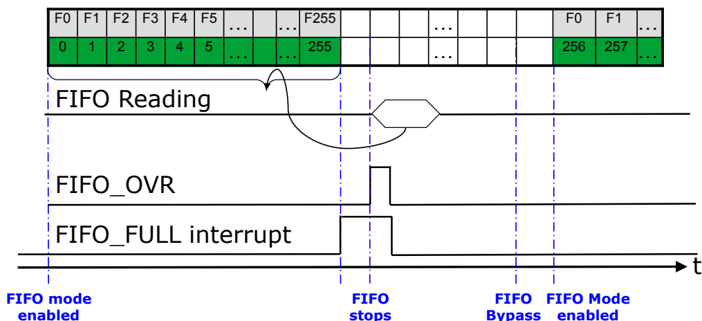
Figure 13. FIFO mode behavior
