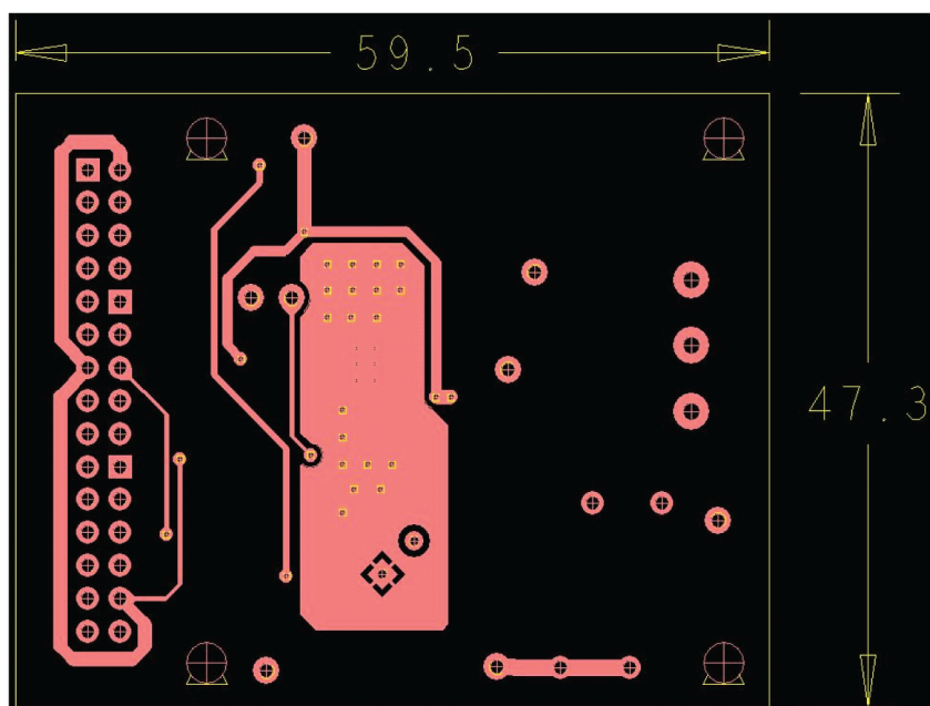
Figure 5. STEVAL-IFP028V1 bottom layout view
