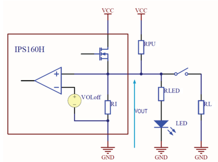
Figure 3. Circuit schematic for typical application case
