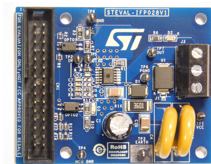
Figure 1. STEVAL-IFP028V1 evaluation board
