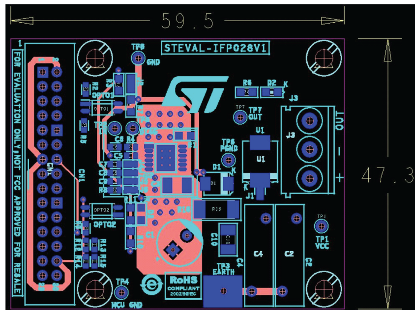
Figure 4. STEVAL-IFP028V1 top and component placement layout view
