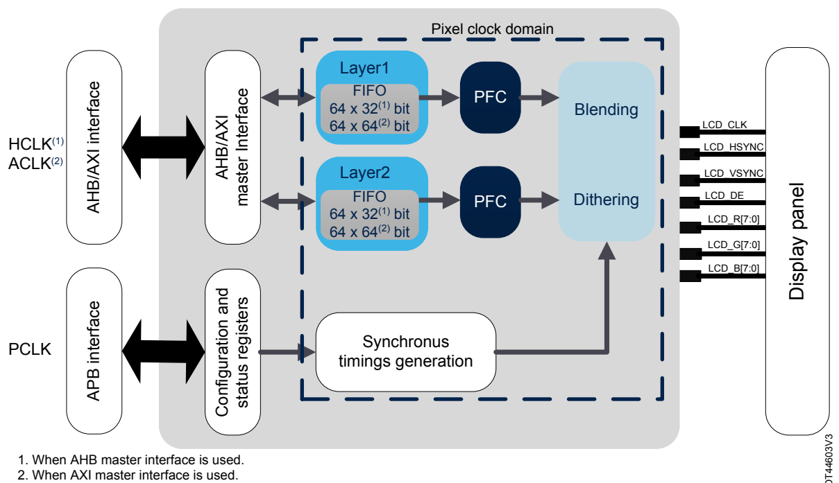
Figure 12. LTDC block diagram
