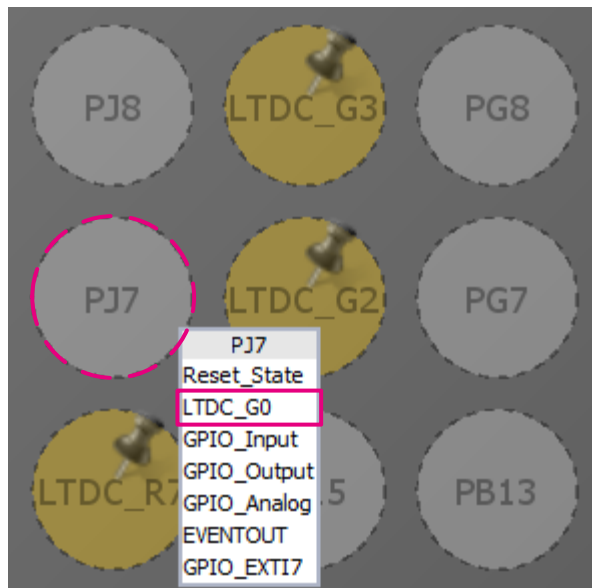
Figure 38. STM32CubeMX: PJ7 pin configuration to LTDC_G0 alternate function
