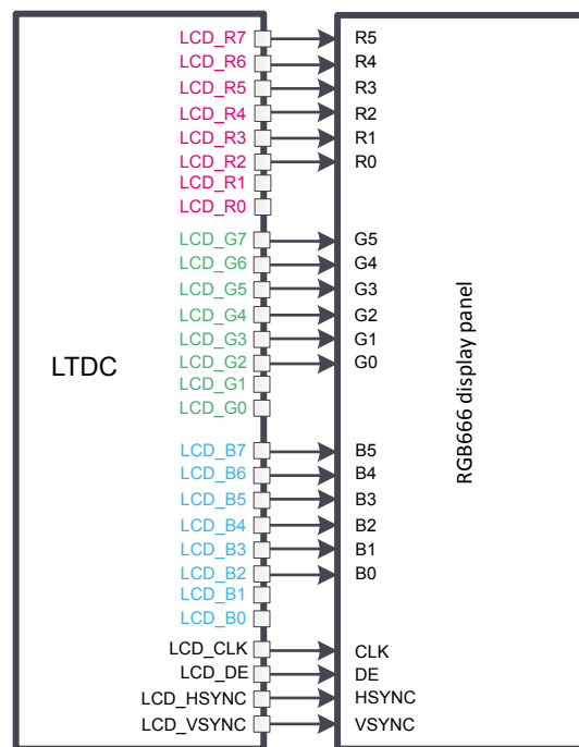
Figure 31. Connecting an RGB666 display panel
