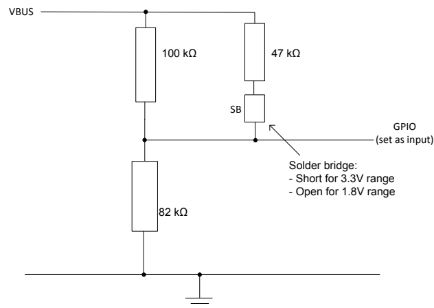
Figure 5. Resistor divider supporting both 1.8 and 3.3V ranges
