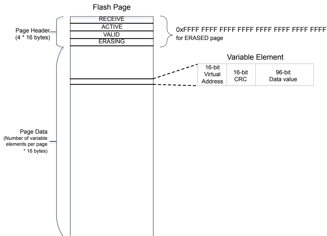
Figure 4. STM32U5 series Flash page and EEPROM variable format
