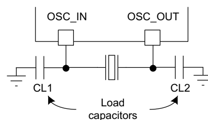
Figure 11. HSE crystal/ceramic resonators
