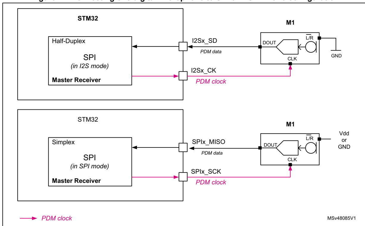
Figure 11. Connecting one digital microphone to SPI or I2S in mono configuration
