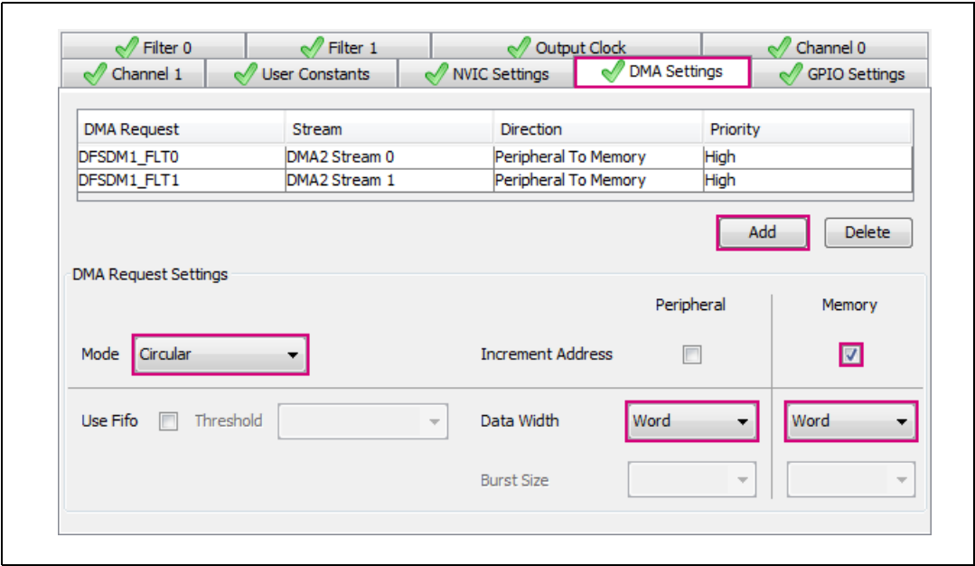
Figure 65. DFSDM DMA setting
