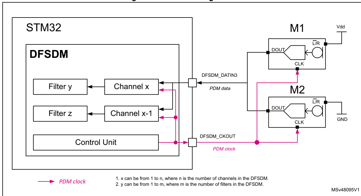
Figure 21. Stereo configuration
