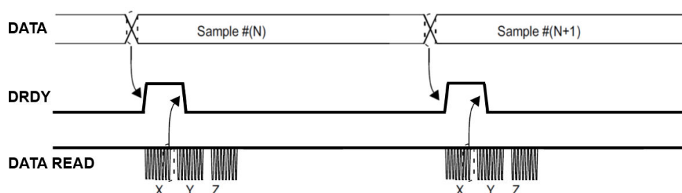
Figure 5. Data-ready signal
