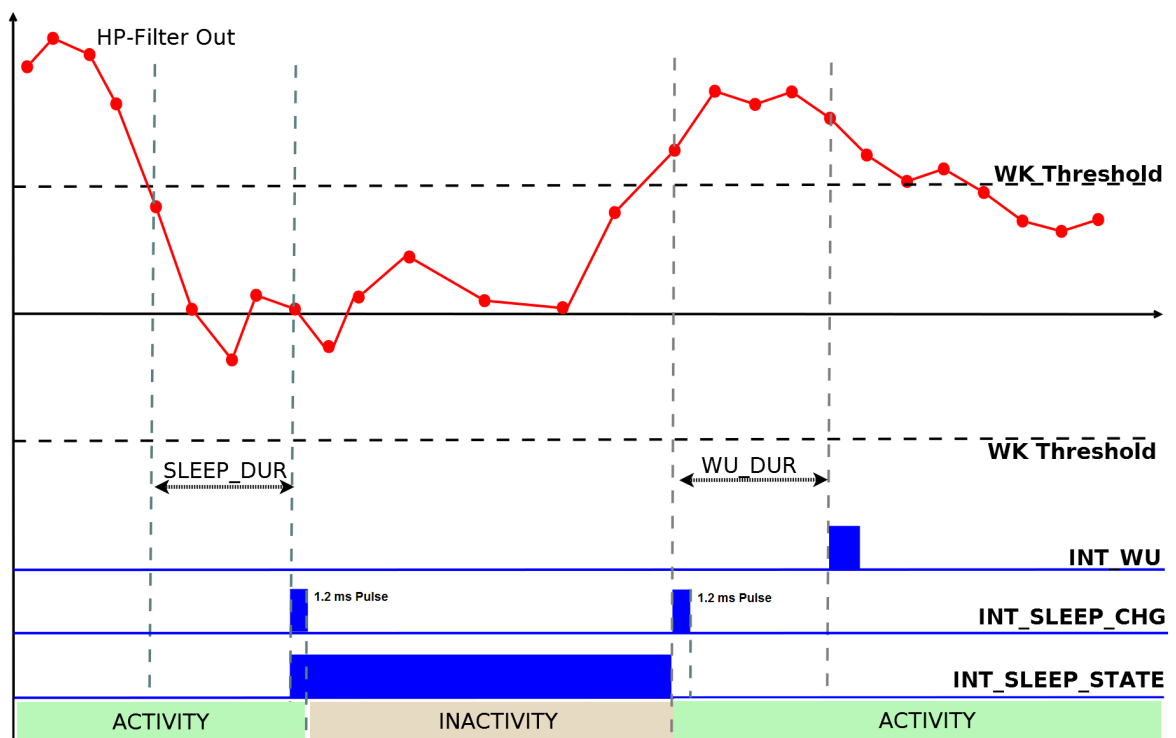
Figure 14. Activity/Inactivity recognition (using the HP filter)
