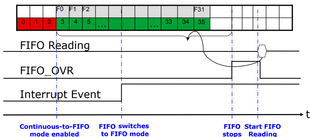
Figure 17. Continuous-to-FIFO mode: interrupt latched and nonlatched
