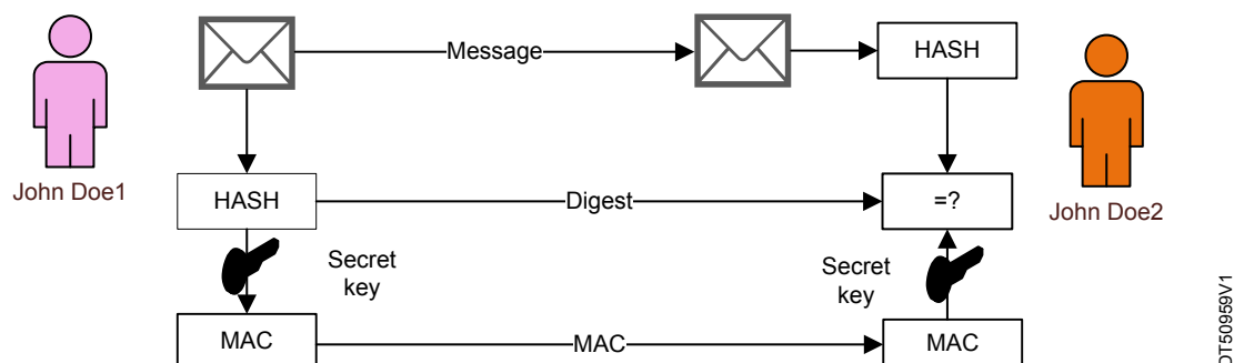
Figure 19. MAC generation with secret key algorithm
