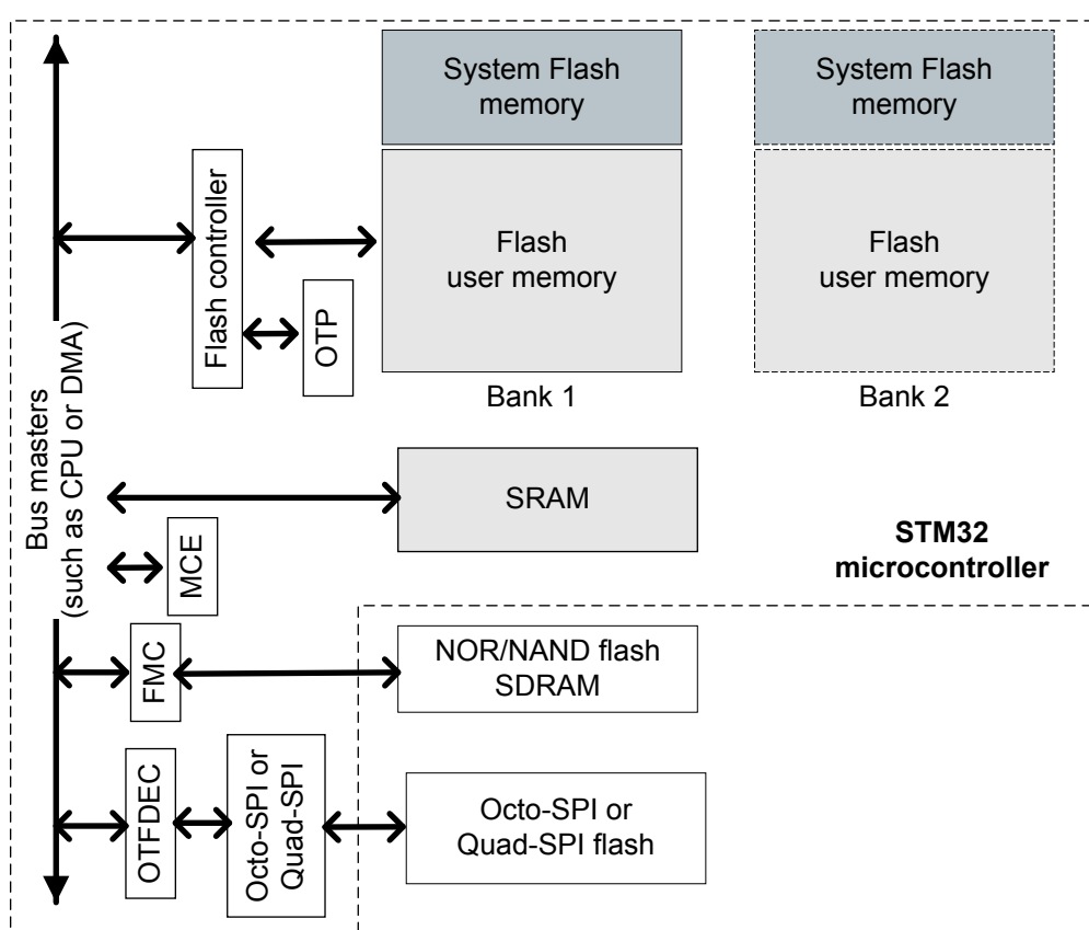
Figure 5. Memory types
