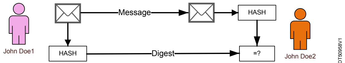
Figure 18. Message hashing
