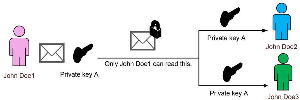
Figure 16. Signature
