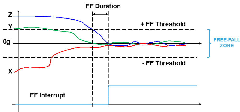
Figure 11. Free-fall interrupt
