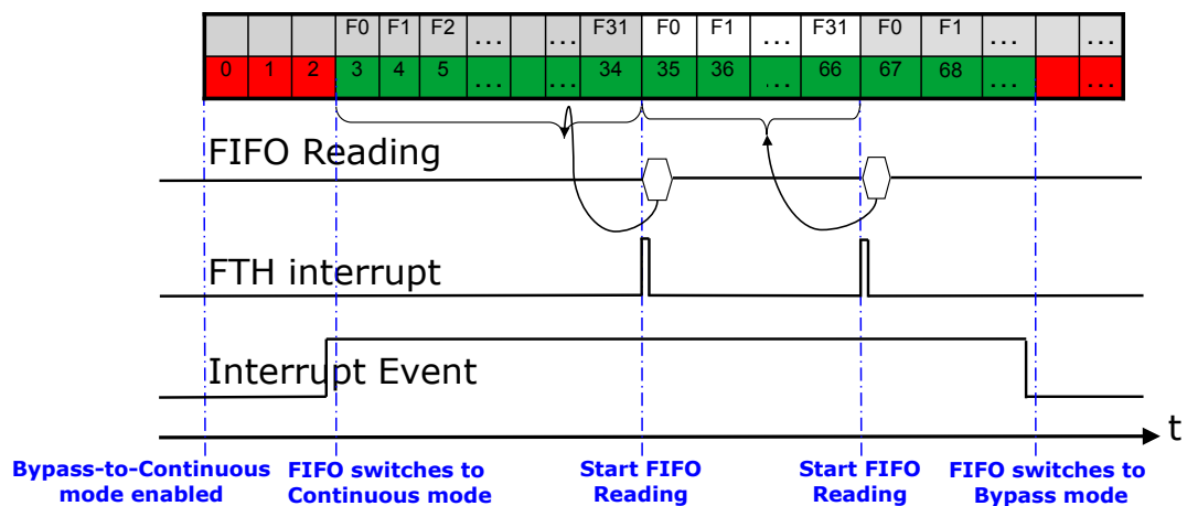
Figure 21. Bypass-to-continuous mode
