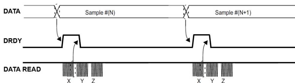
Figure 8. Data-ready signal
