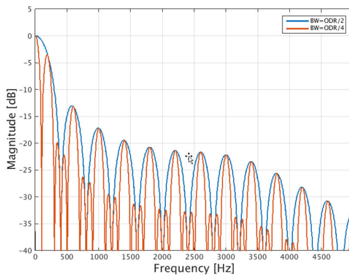
Figure 7. LPF1 / LPF2 - low-power mode 4 - ODR 200 Hz
