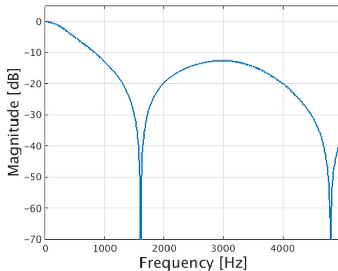
Figure 5. LPF1 - high-performance mode, ODR = 1600 Hz, BW = 400 Hz
