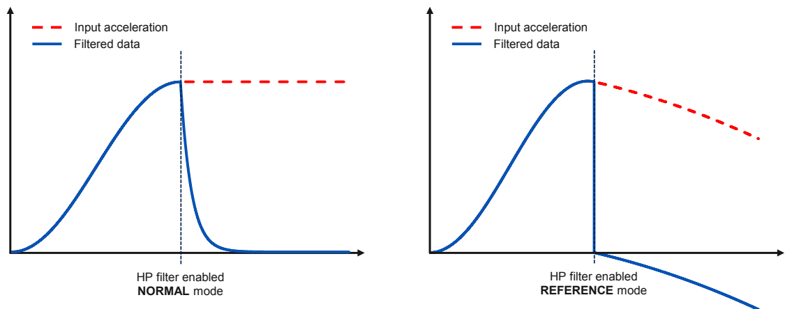
Figure 4. High-pass filter in normal and reference mode
