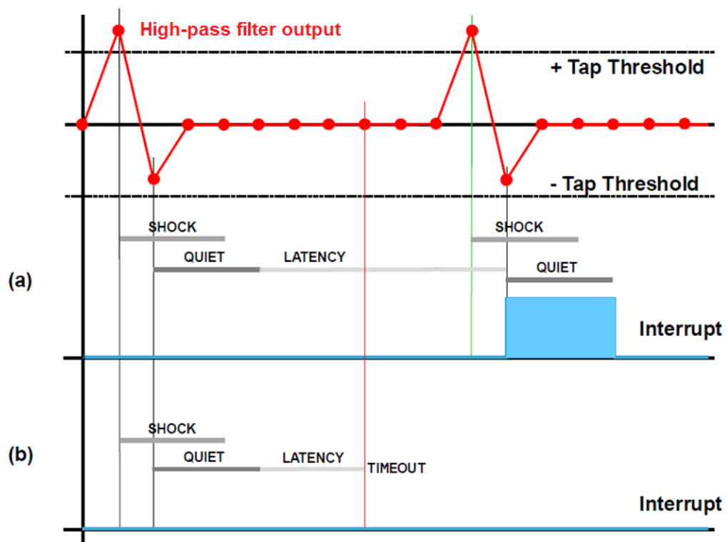
Figure 15. Double-tap event recognition (LIR bit = 0)
