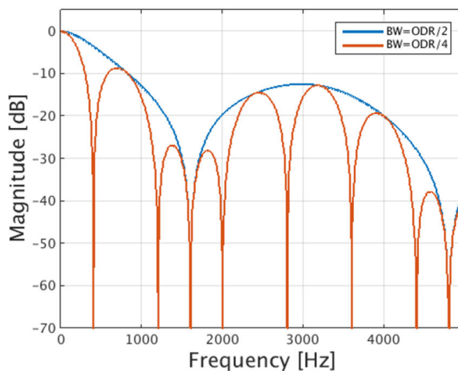
Figure 6. LPF1 / LPF2 - high-performance mode, ODR 800 Hz
