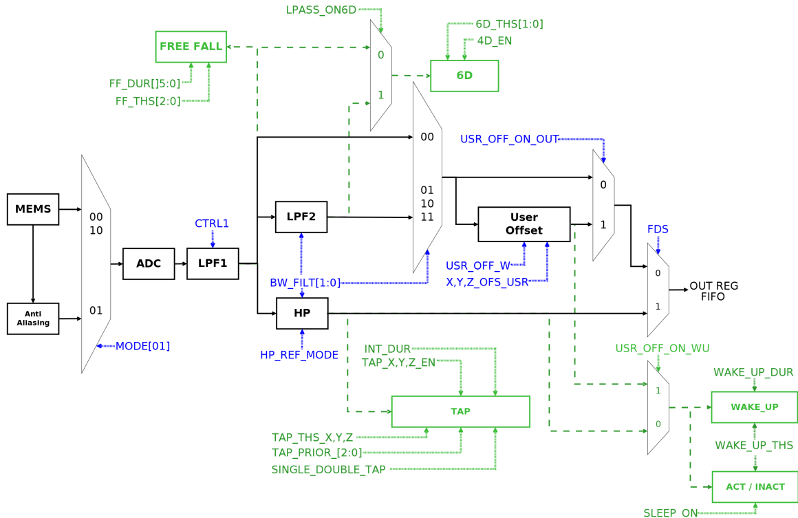
Figure 9. Embedded functions
