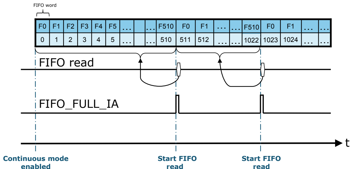
Figure 29. Continuous mode
