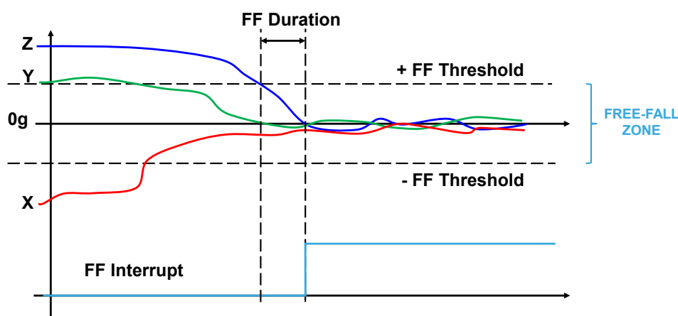
Figure 13. Free-fall interrupt
