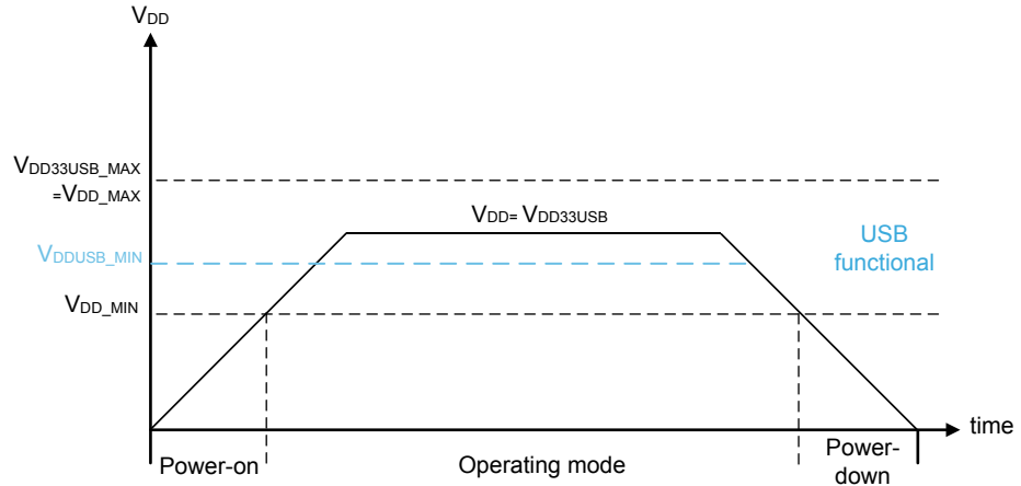
Figure 5. VDD33USB connected to V_{DD} power supply
