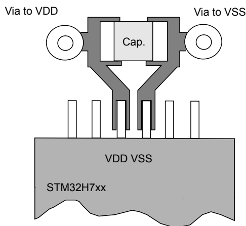
Figure 19. Typical layout for V DD /V SS pair
