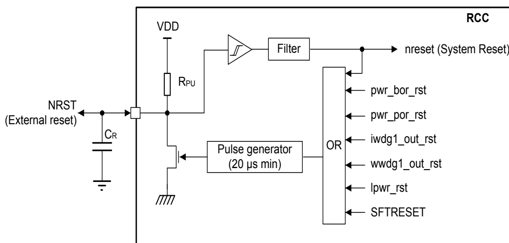
Figure 10. Reset circuit
