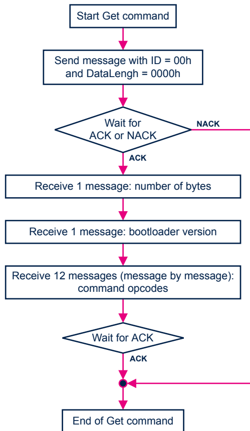
Figure 2. Get command (host side)
