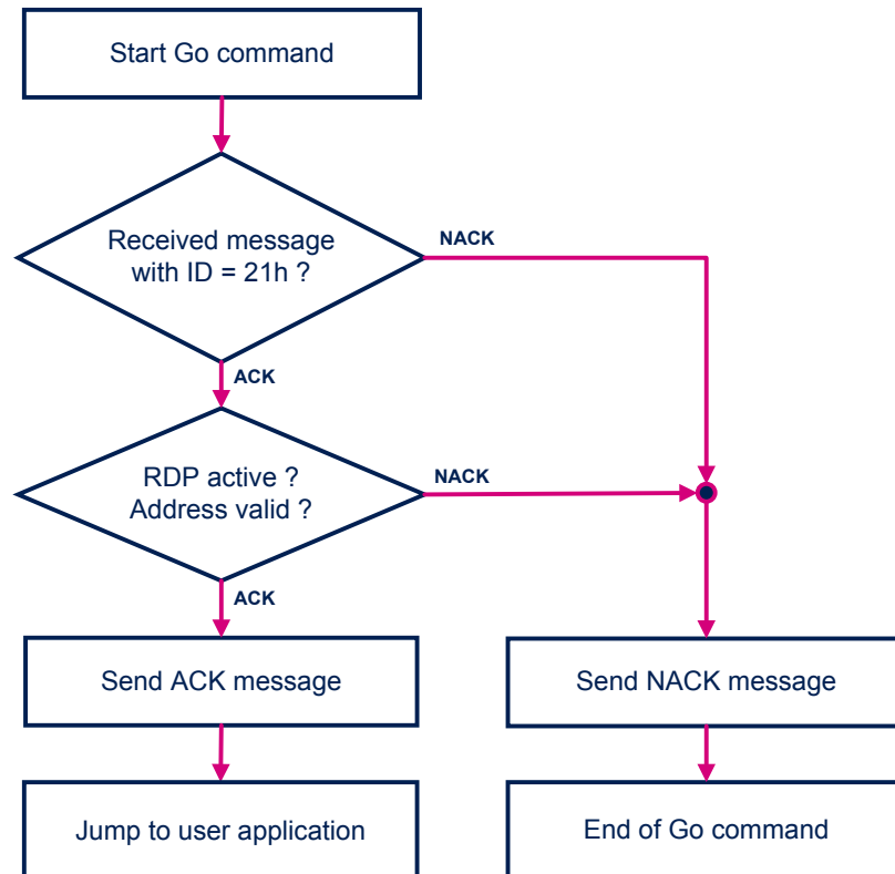
Figure 11. Go command (device side)
