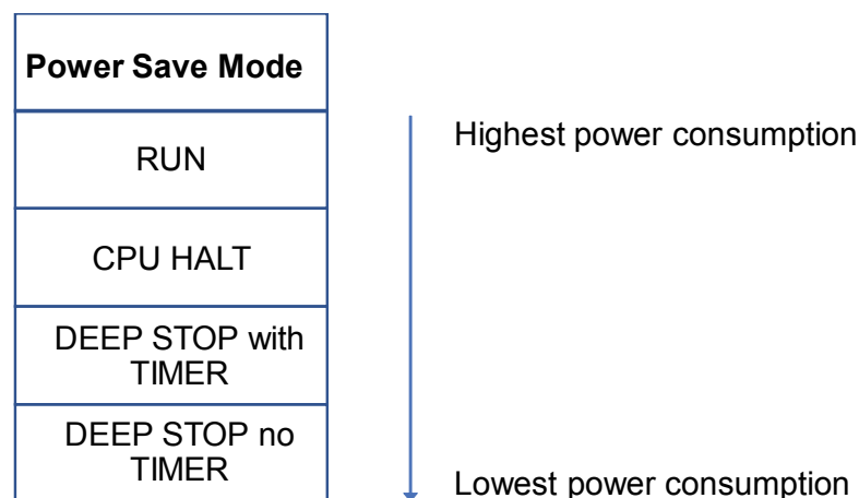
Figure 1. BlueNRG-LP, BlueNRG-LPS power save modes
