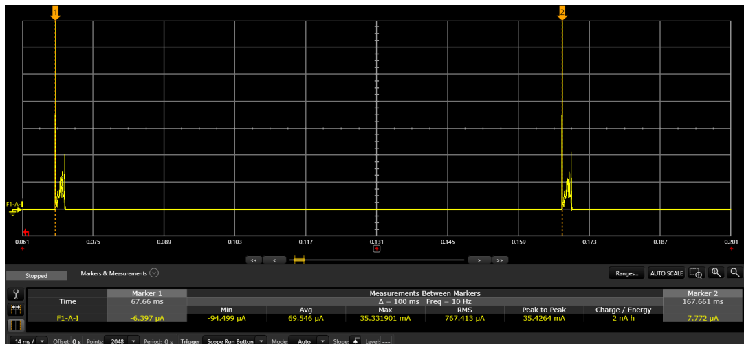
Figure 4. BlueNRG-LP connection procedure: interval 100 ms
