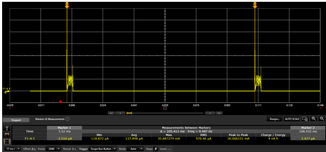
Figure 2. BlueNRG-LP advertising procedure: interval 100 ms
