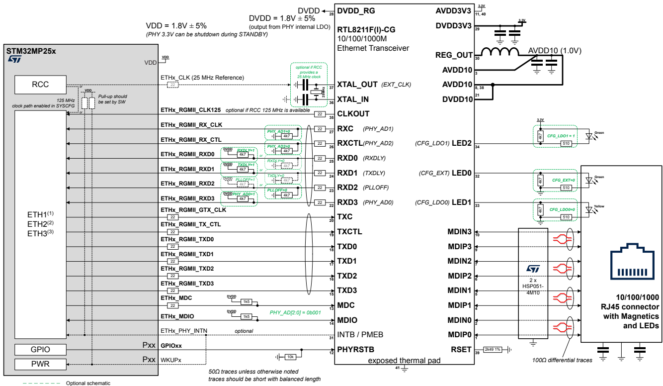
Figure 42. Gigabit Ethernet PHY connection with V_{DD} = 1.8\text{ V} (RTL8211F)
