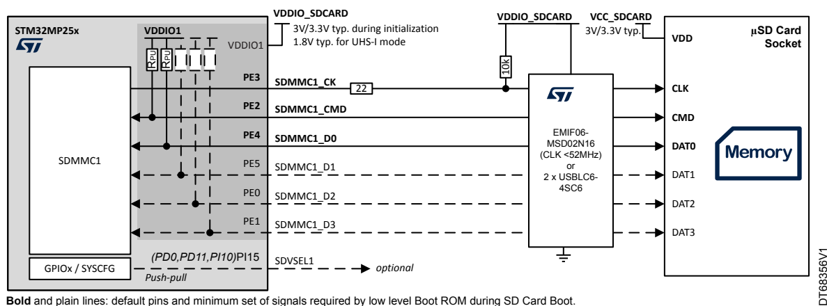
Figure 27. SD-Card with embedded level shifter connection
