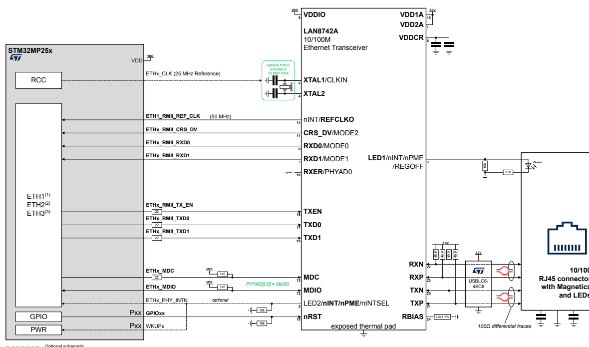
Figure 38. 10/100M Ethernet PHY connection example
