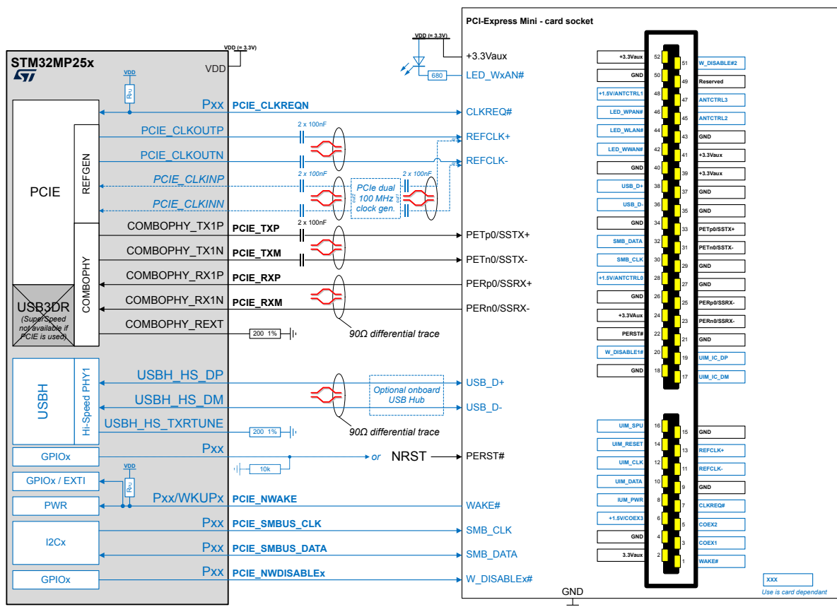
Figure 37. PCIE example with connection to a PCI-Express mini
