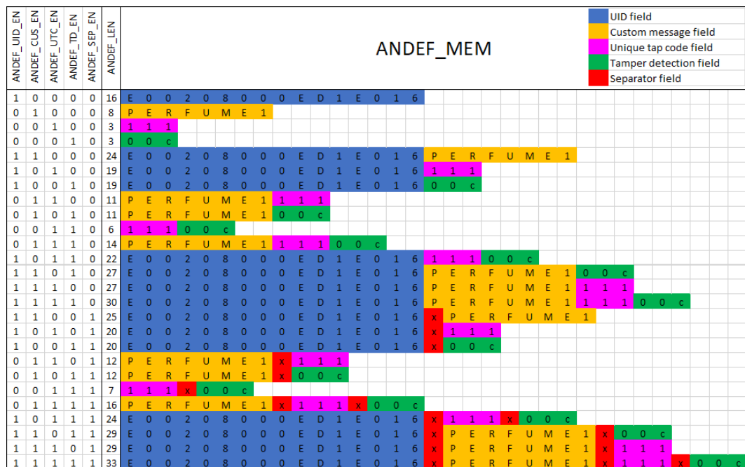
Figure 4. Possible combinations of ANDEF fields in ANDEF_MEM memory
