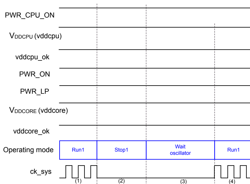
Figure 11. Wake-up sequence from Stop1
