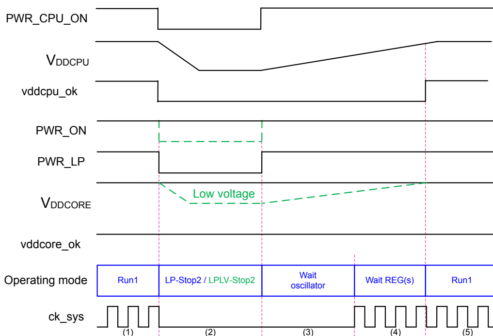
Figure 14. Wake-up sequence from LP-Stop2/LPLV-Stop2
