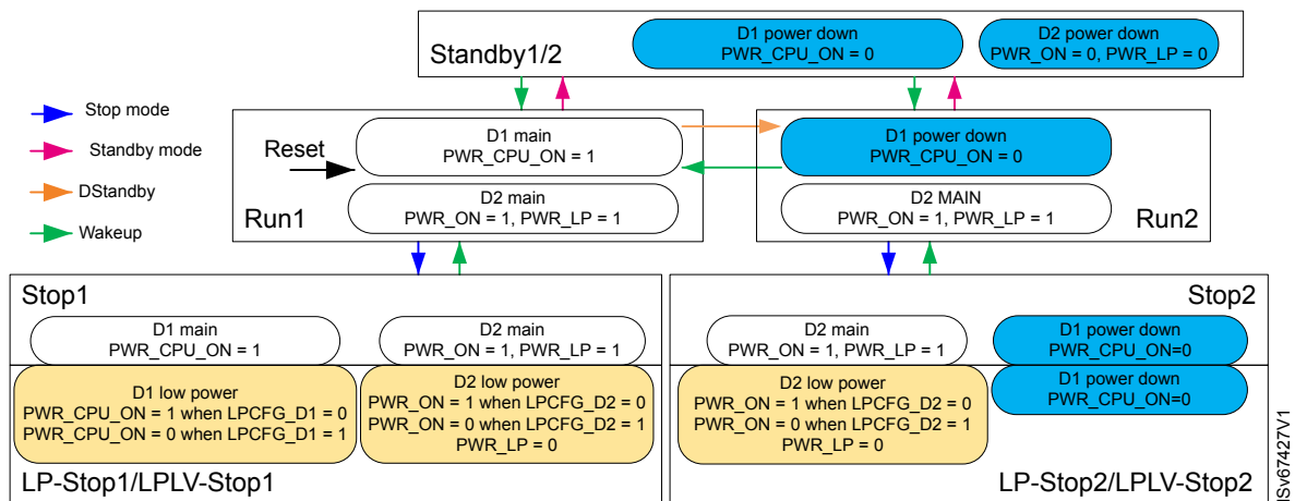
Figure 4. Power states and external regulator control
