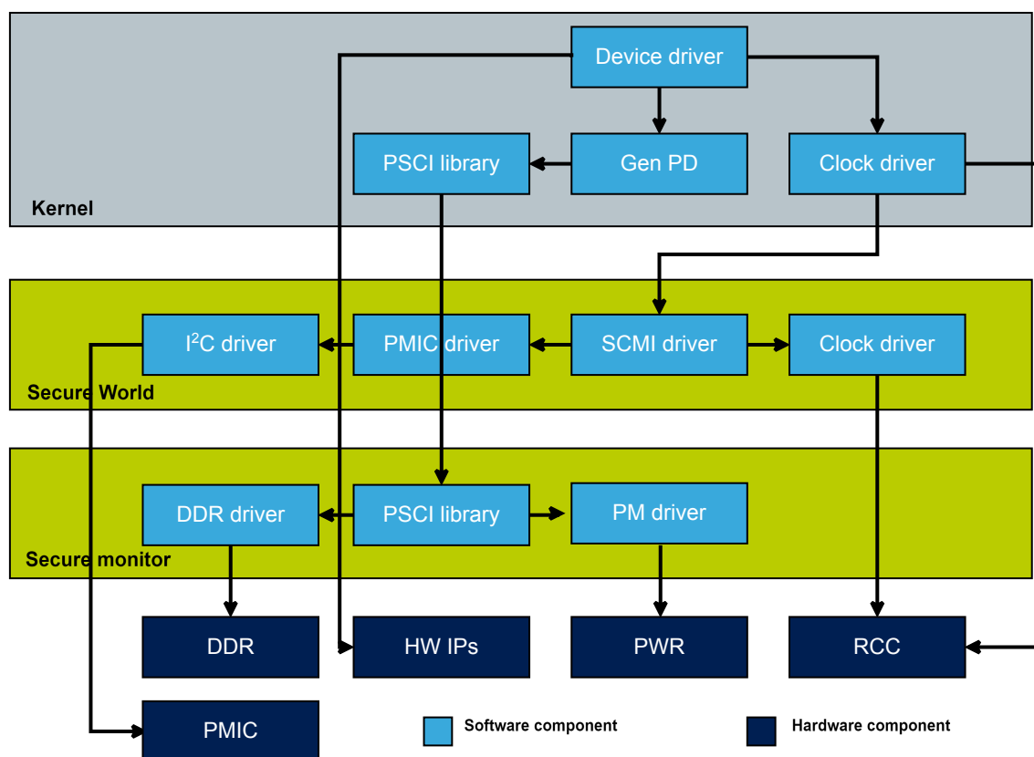
Figure 8. Linux power management software framework
