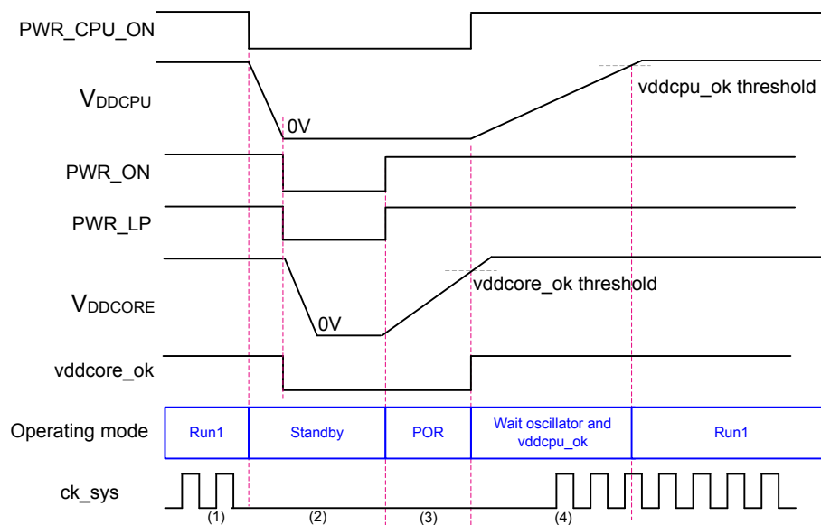
Figure 15. Wake-up sequence from Standby1 and Standby2
