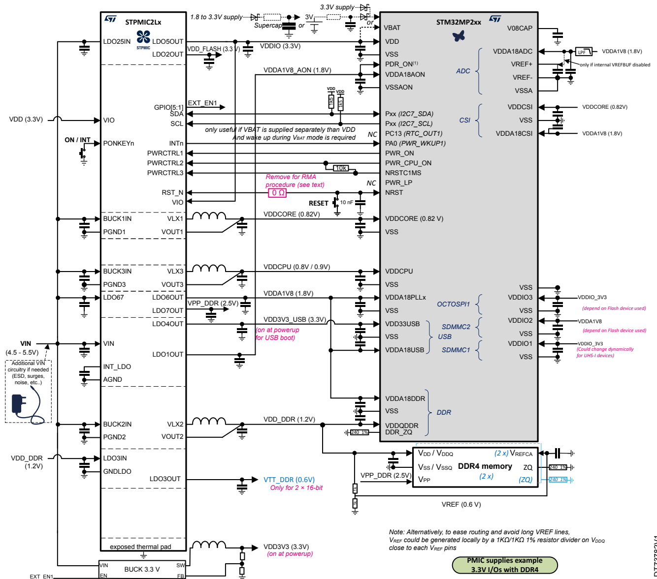
Figure 6. STPMIC2LAPQR example 3.3 V I/Os with DDR4
