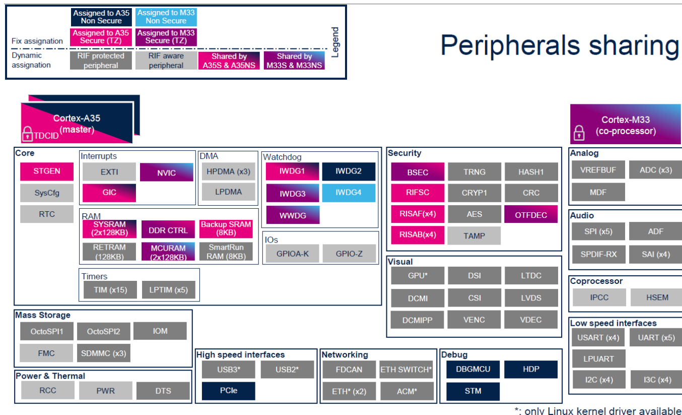
Figure 17. STM32MP2 lines peripheral assignment using OpenSTLinux distribution
