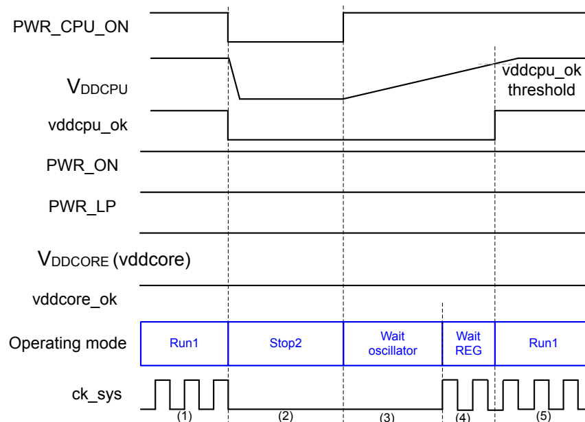
Figure 12. Wake-up sequence from Stop2
