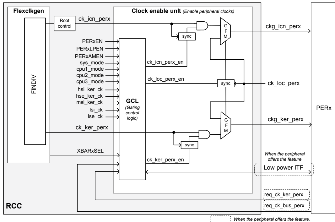
Figure 18. Peripheral clock enable logic details
