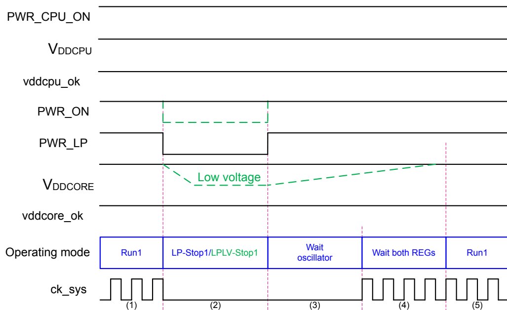
Figure 13. Wake-up sequence from LP-Stop1/LPLV-Stop1
