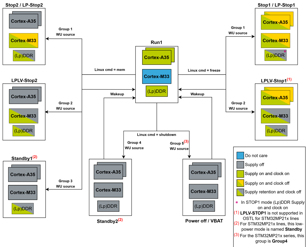
Figure 9. Available power state transitions
