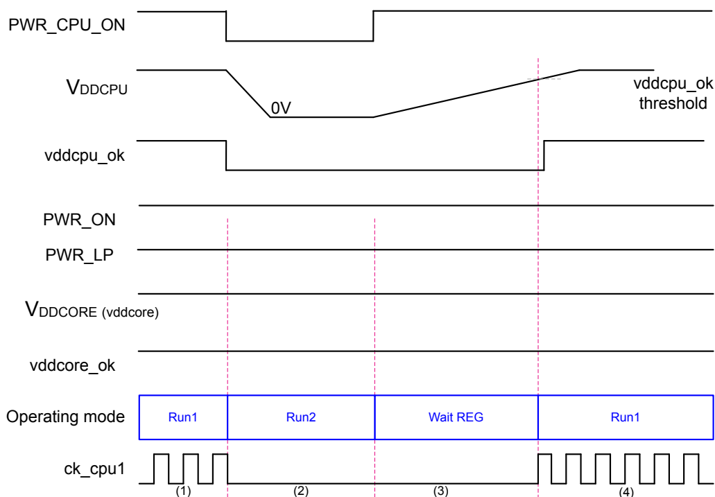
Figure 10. Wake-up sequence from Run2
