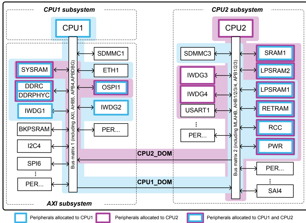
Figure 16. Peripheral allocation example
