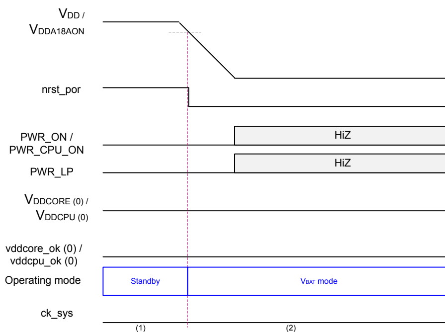
Figure 7. Device VBAT mode power control
