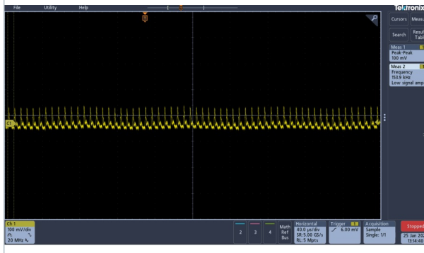
Figure 23. Ripple & noise at 230 Vac input 15 Vout / 3 A Vpeak-peak=100 mV
