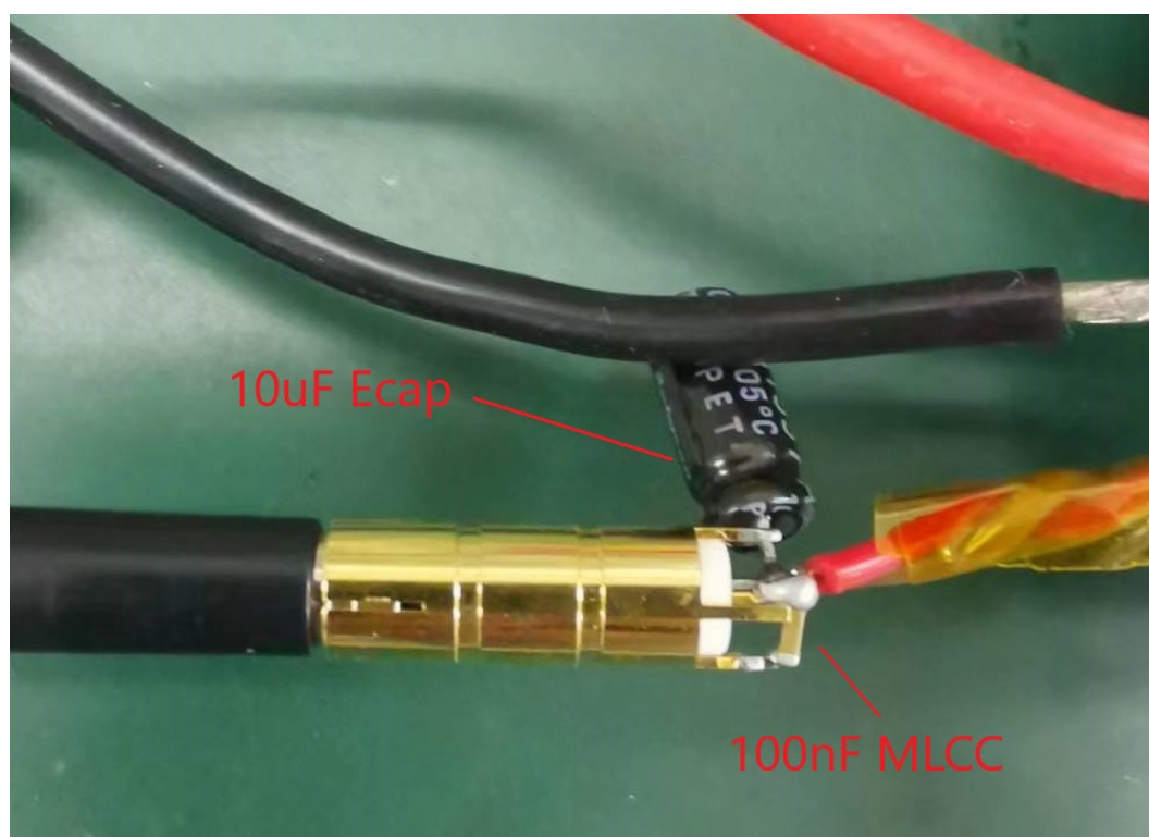
Figure 8. Ripple & noise test setup probe 10 uF E-cap+100 nF ceramic cap added
