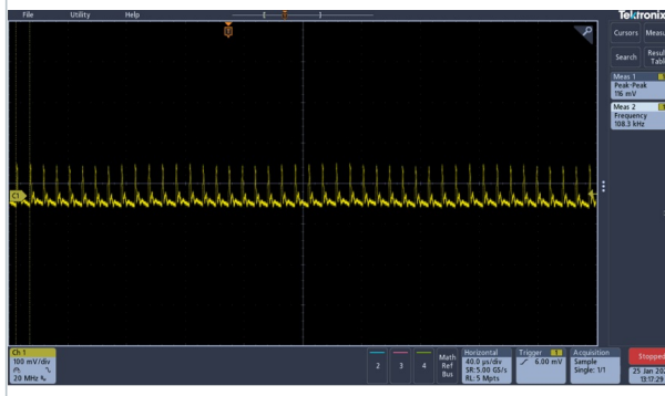
Figure 25. Ripple & noise at 115 Vac input 20 Vout / 2.25 A Vpeak-peak=124 mV
