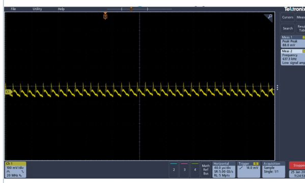
Figure 13. Ripple & noise at 115 Vac input 9 Vout / 3 A Vpeak-peak=88 mV
