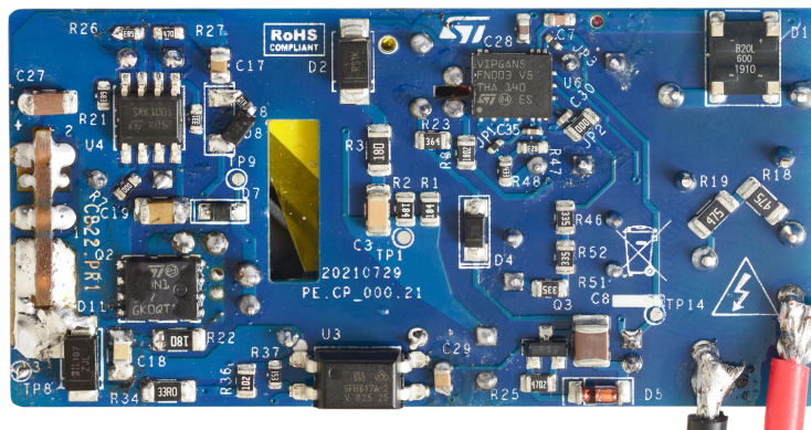
Figure 2. EVLVIPGAN50PD reference design - bottom
