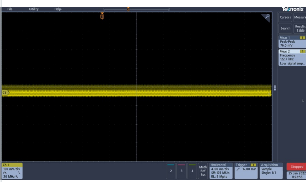
Figure 16. Ripple & noise at 230 Vac input 9 Vout / 3 A Vpeak-peak=76 mV (nr. 2)
