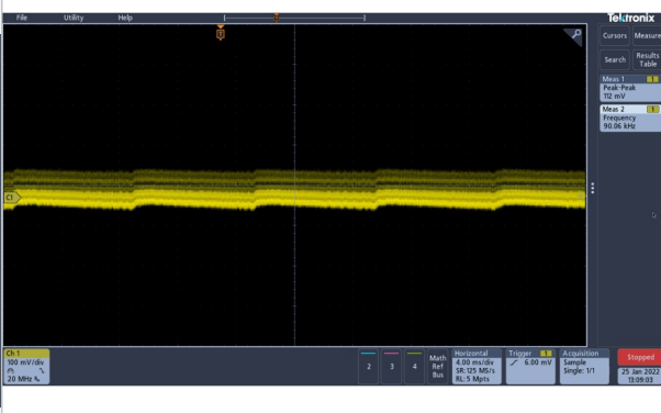
Figure 18. Ripple & noise at 115 Vac input 12 Vout / 3 A Vpeak-peak=112 mV (nr. 2)
