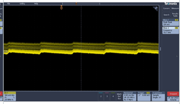
Figure 26. Ripple & noise at 115 Vac input 20 Vout / 2.25 A Vpeak-peak=124 mV (nr. 2)
