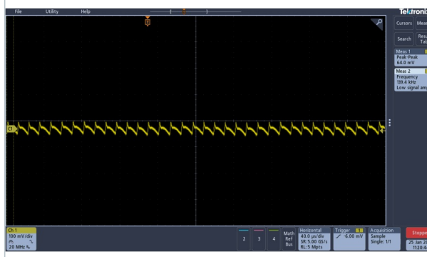
Figure 11. Ripple & noise at 230 Vac input 5 Vout / 3 A Vpeak-peak=64 mV
