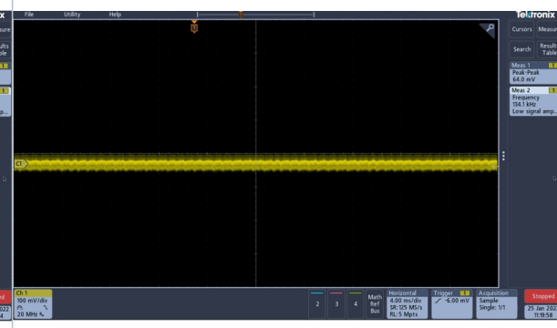
Figure 12. Ripple & noise at 230 Vac input 5 Vout / 3 A Vpeak-peak=64 mV (nr. 2)
