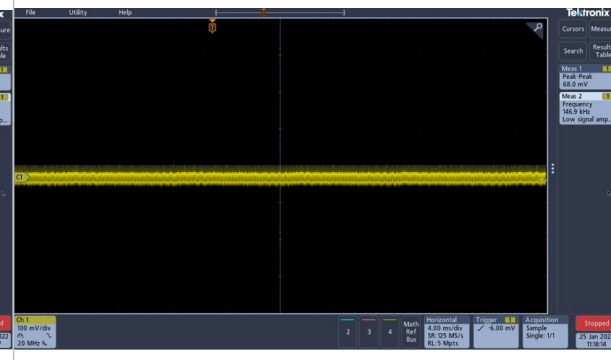
Figure 10. Ripple & noise at 115 Vac input 5 Vout / 3 A Vpeak-peak=68 mV (nr.2)
