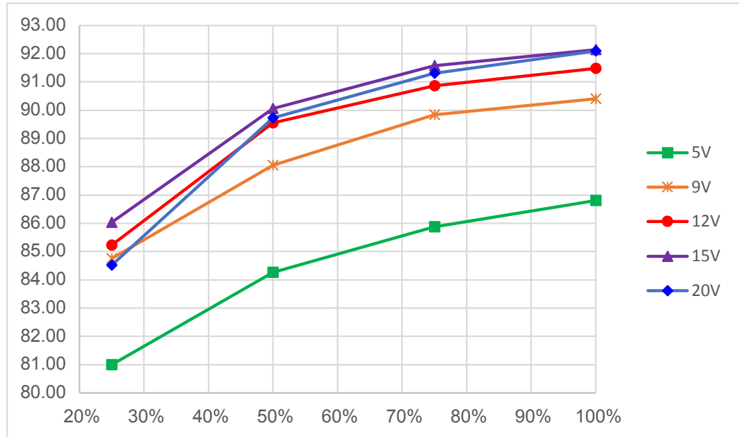
Figure 5. EVLVIPGAN50PD efficiency at 230 Vac input
