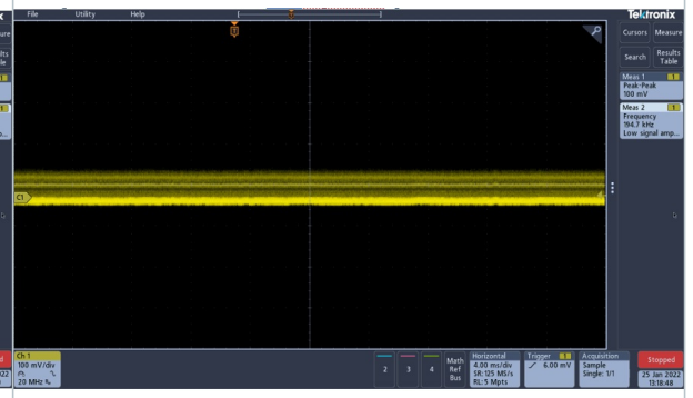
Figure 28. Ripple & noise at 230 Vac input 20 Vout / 2.25 A Vpeak-peak=100 mV (nr. 2)
