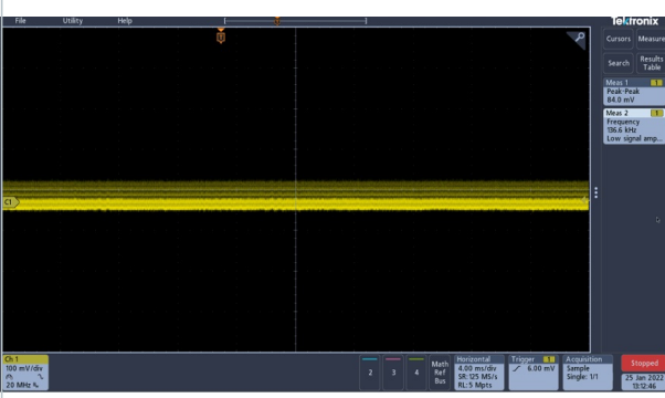
Figure 20. Ripple & noise at 230 Vac input 12 Vout / 3 A Vpeak-peak=84 mV (nr. 2)
