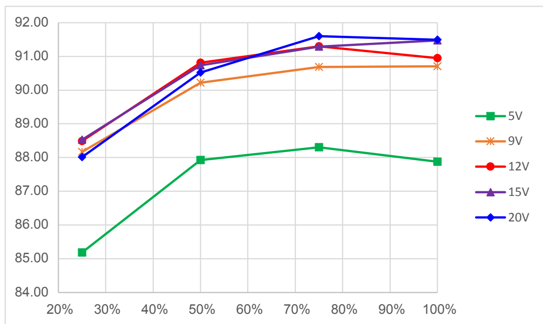
Figure 4. EVLVIPGAN50PD efficiency at 115 Vac input
