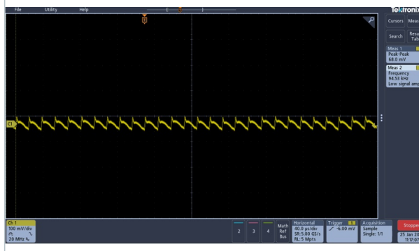
Figure 9. Ripple & noise at 115 Vac input 5 Vout / 3 A Vpeak-peak=68 mV
