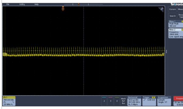
Figure 27. Ripple & noise at 230 Vac input 20 Vout / 2.25 A Vpeak-peak=100 mV
