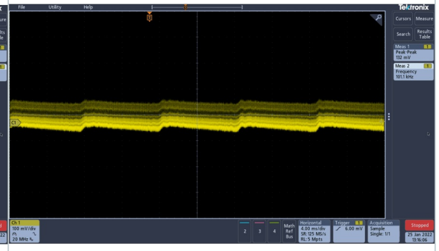
Figure 22. Ripple & noise at 115 Vac input 15 Vout / 3 A Vpeak-peak=132 mV (nr. 2)
