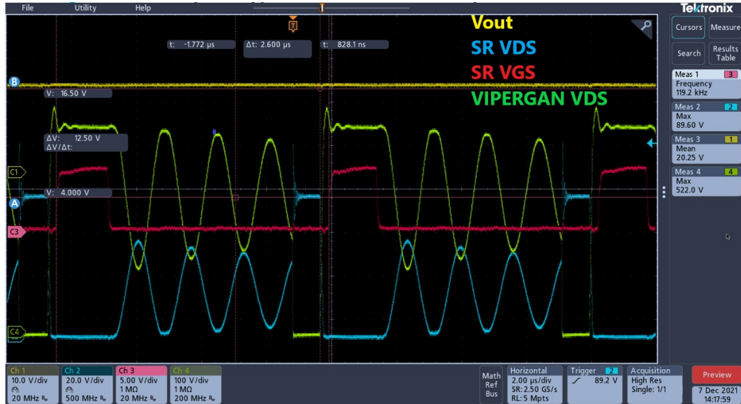
Figure 30. Primary side typical waveforms-normal operation with 230 Vin 20 Vout/0.67 A
