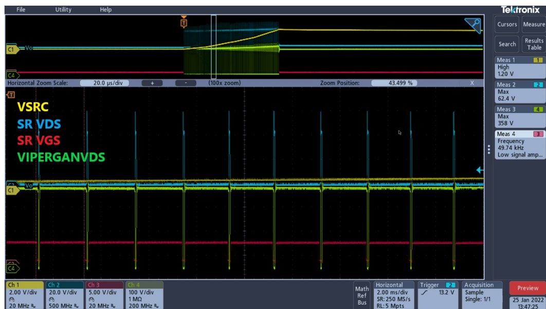
Figure 29. Startup waveform
