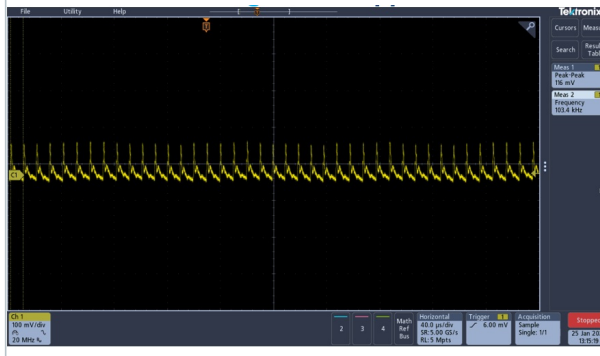
Figure 21. Ripple & noise at 115 Vac input 15 Vout / 3 A Vpeak-peak=132 mV
