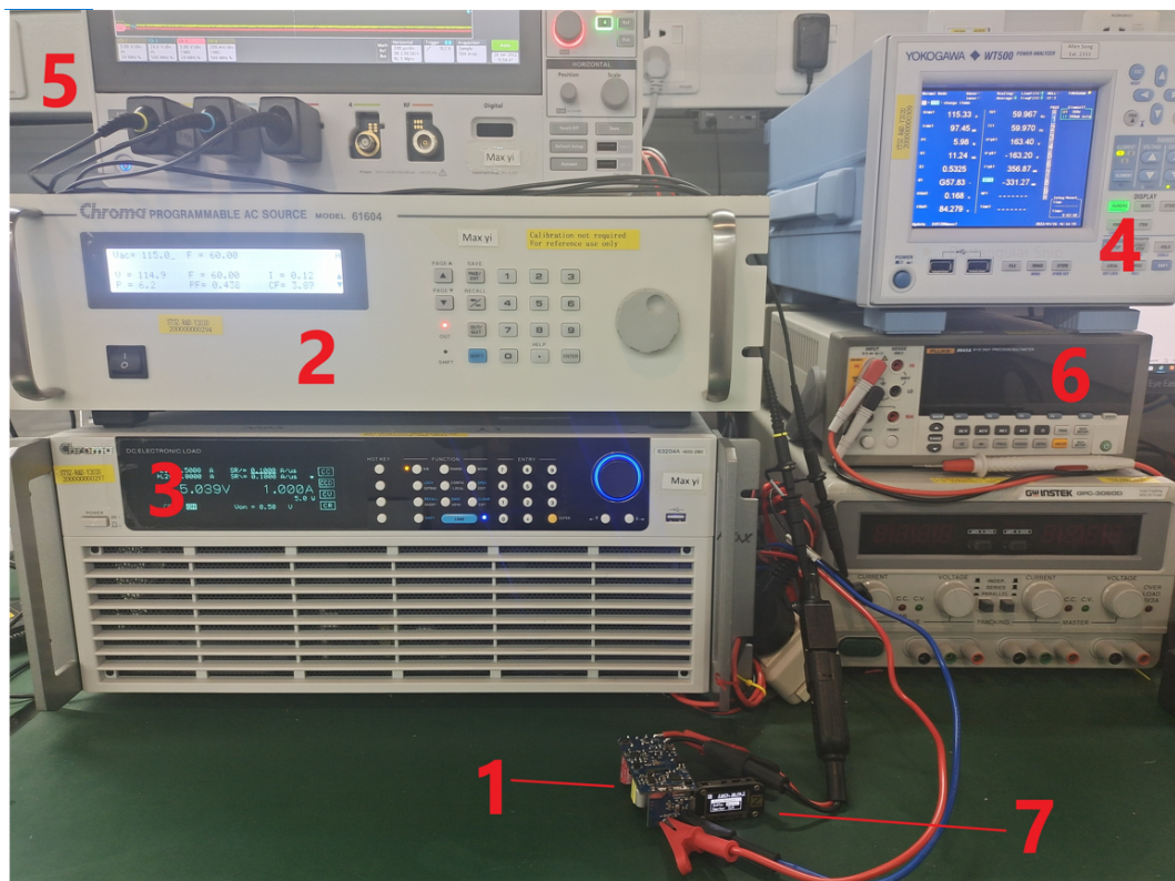
Figure 3. EVLVIPGAN50PD test setup
