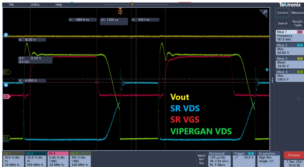
Figure 31. Secondary SR MOSFET Vds at 20 V 2.25 A
