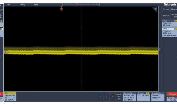
Figure 14. Ripple & noise at 115 Vac input 9 Vout / 3 A Vpeak-peak=88 mV (nr. 2)
