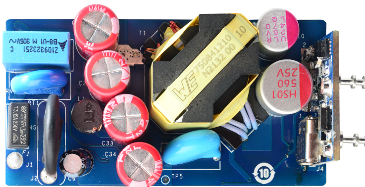
Figure 1. EVLVIPGAN50PD reference design - top
