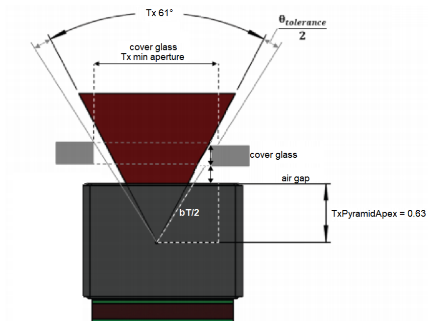
Figure 11. Cover glass Tx aperture with angle tolerance in y direction
