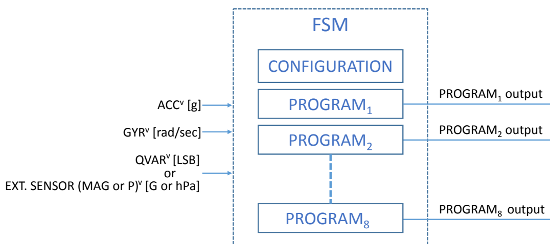
Figure 4. FSM block
