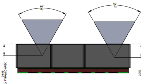
Figure 6. VL53L7CX nominal FoV example
