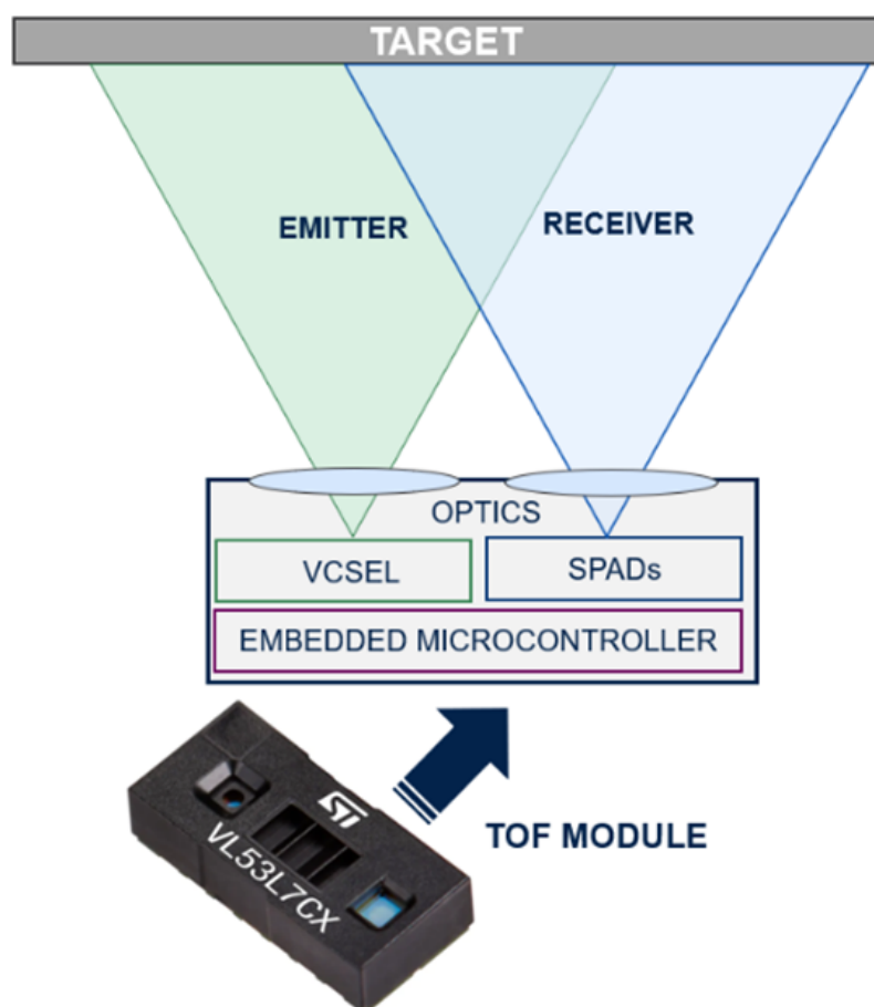
Figure 2. ToF module overview
