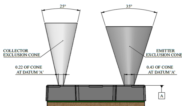
Figure 7. Example of the VL53L3CX exclusion cones/zones
