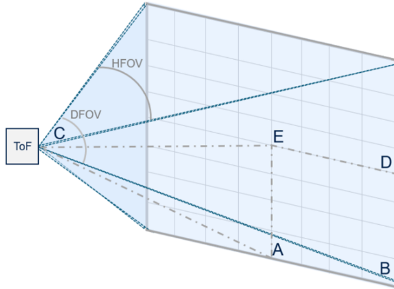
Figure 4. Points used for computing diagonal FoVs
