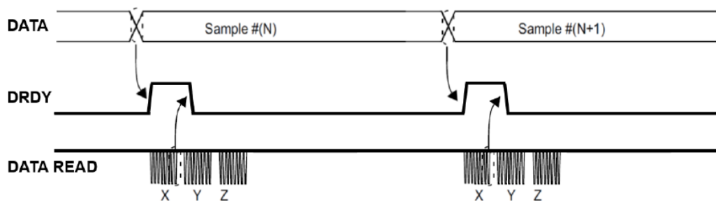
Figure 7. Data-ready signal
