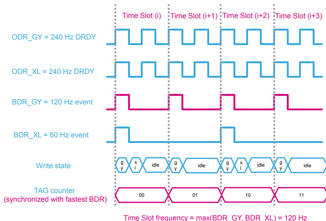
Figure 26. Main sensors and time slot definitions
