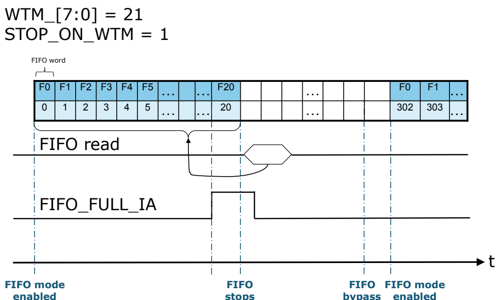
Figure 34. FIFO threshold (STOP_ON_WTM = 1) in FIFO mode
