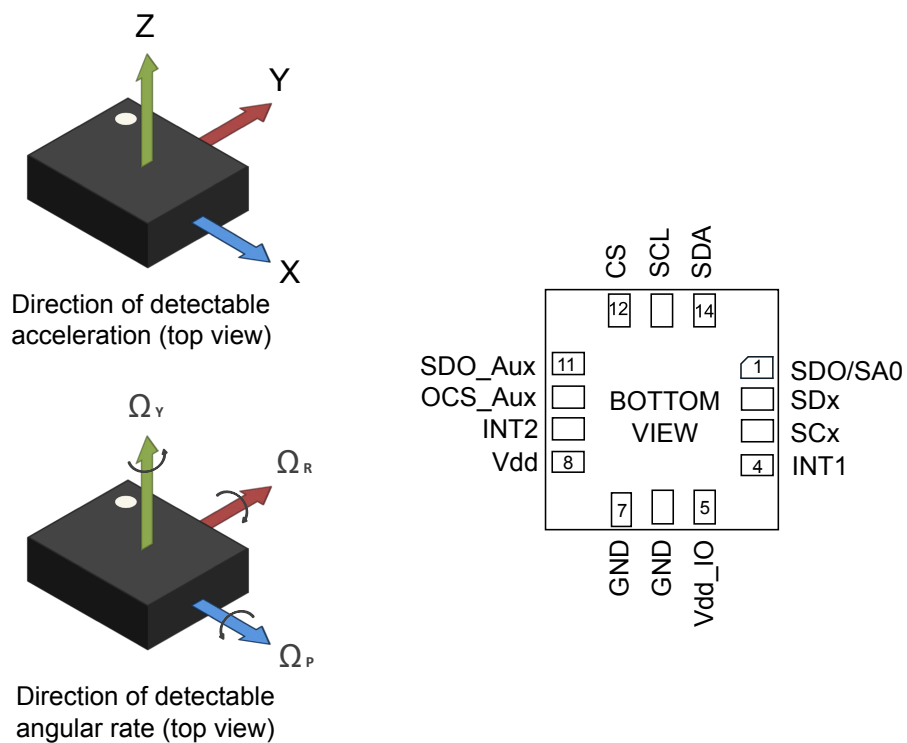
Figure 1. Pin connections
