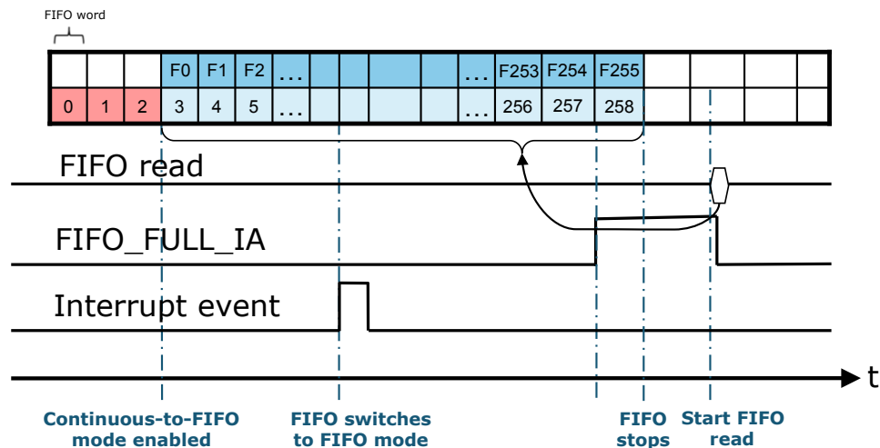
Figure 29. Continuous-to-FIFO mode
