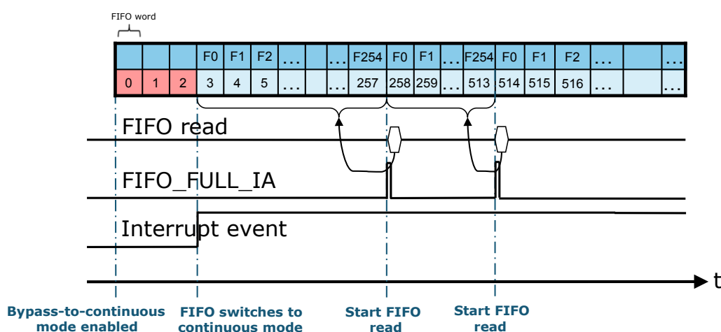
Figure 30. Bypass-to-continuous mode
