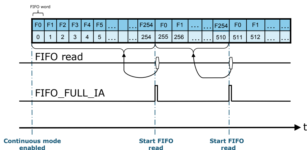
Figure 28. Continuous mode
