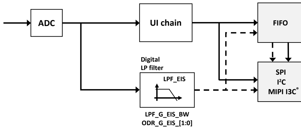
Figure 8. Gyroscope EIS channel
