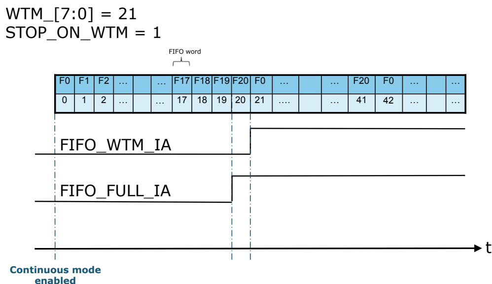
Figure 35. FIFO threshold (STOP_ON_WTM = 1) in continuous mode
