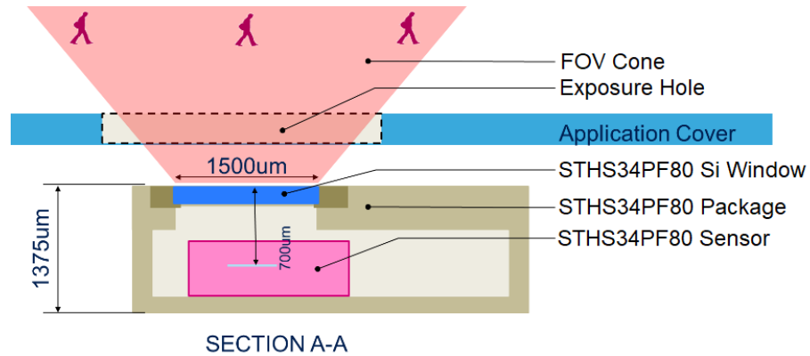
Figure 4. Example of application architecture and corresponding field of view
