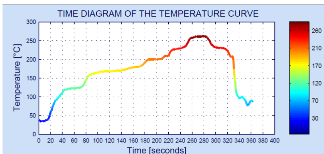
Figure 22. Soldering profile
