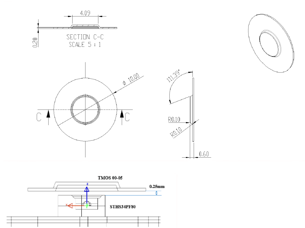
Figure 14. Mechanical dimensions of the TMOS00-05
