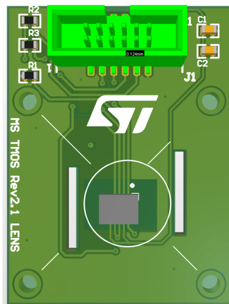
Figure 20. ST evaluation board PCB with trenches near the sensor
