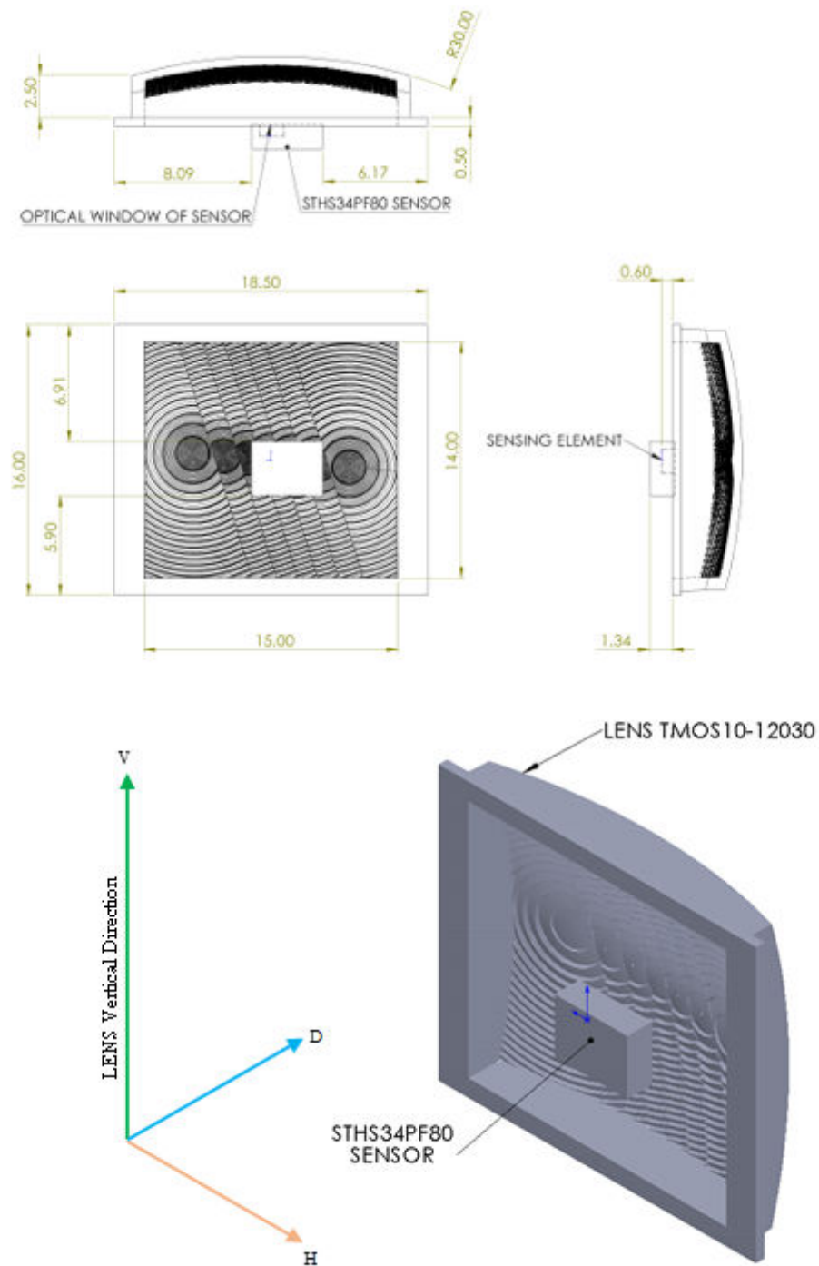
Figure 11. Mechanical dimensions of the TMOS10-12 lens
