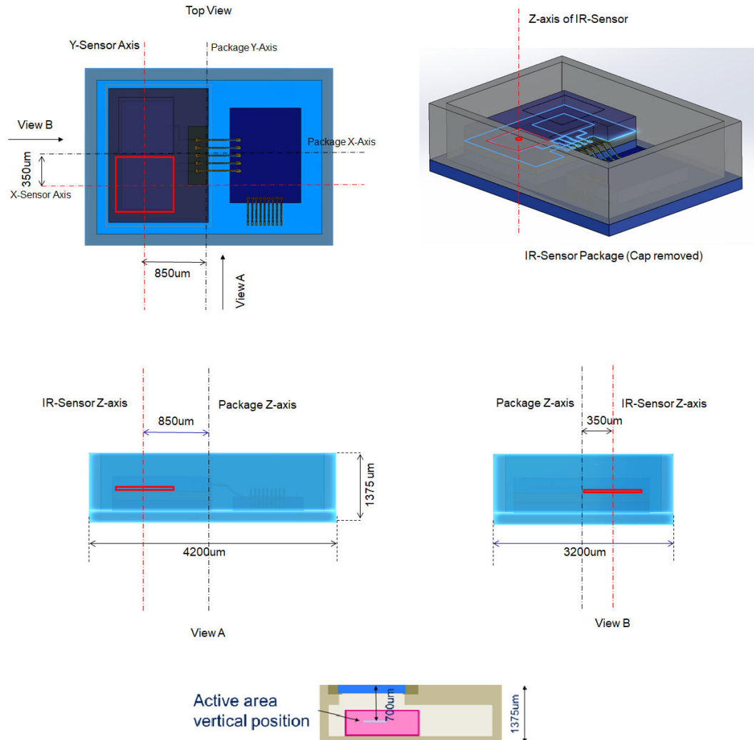
Figure 3. Mechanical dimensions for optical alignment
