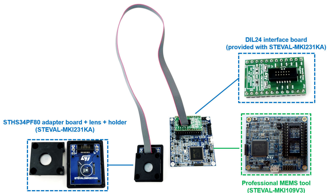
Figure 16. STHS34PF80 evaluation board
