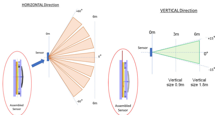
Figure 12. Detectable field of view and distance of TMOS10-12
