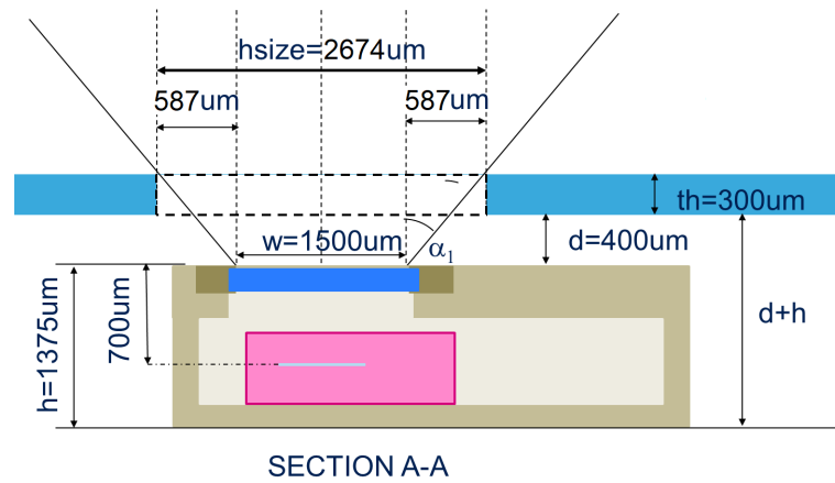
Figure 5. Example 1 of the exposure hole calculation
