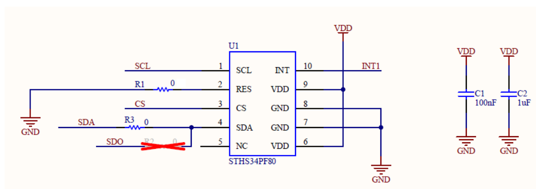
Figure 15. Circuit of the STHS34PF80 evaluation board
