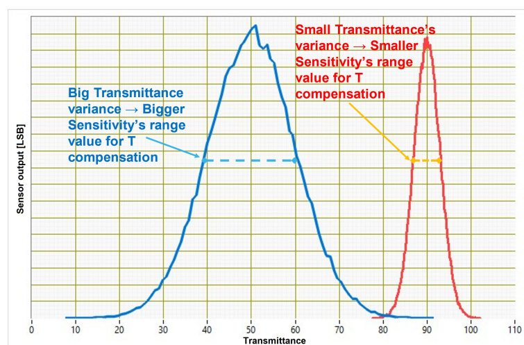
Figure 7. Transmittance variance
