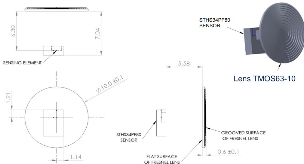
Figure 8. Mechanical dimensions of the TMOS63-10 lens
