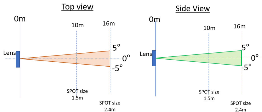
Figure 9. Detectable field of view and distance of TMOS63-10
