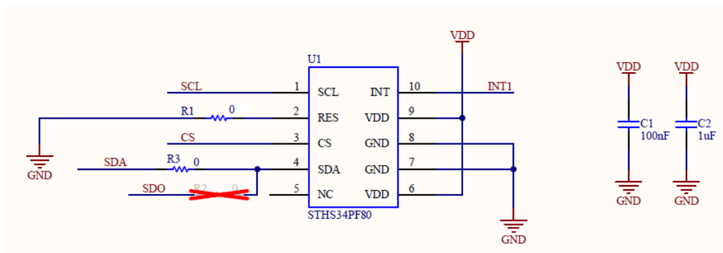
Figure 21. Circuit of STHS34PF80 evaluation board
