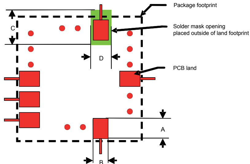
Figure 17. Example of PCB lands (LGA package)
