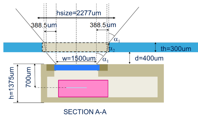
Figure 6. Example 2 of the exposure hole calculation
