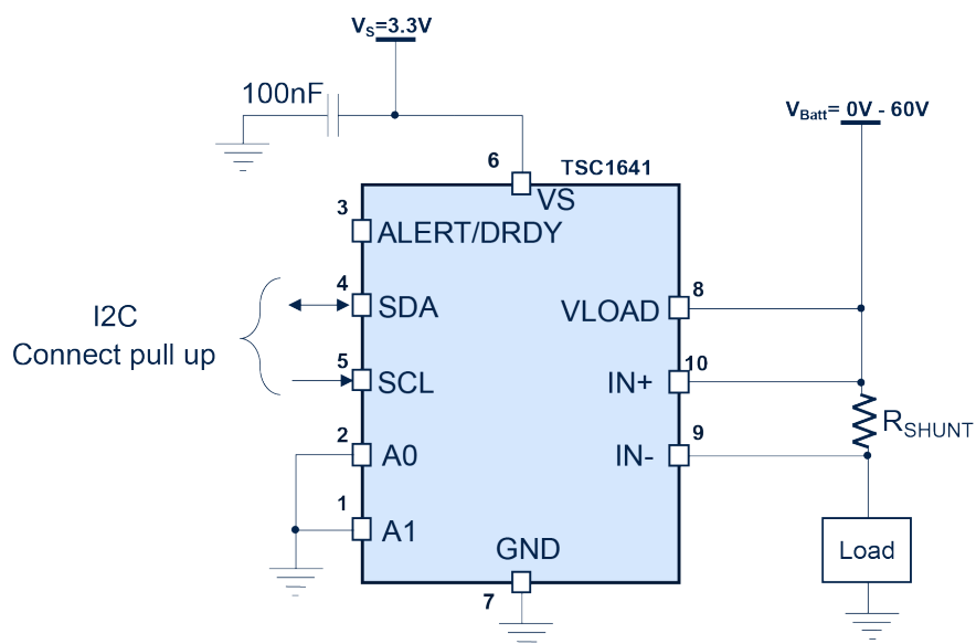
Figure 3. Typical I 2 C hardware configuration
