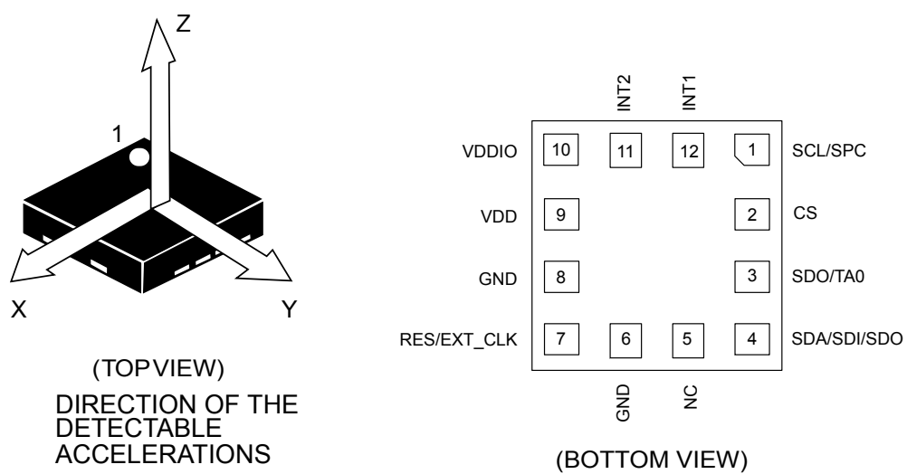
Figure 1. Pin connections
