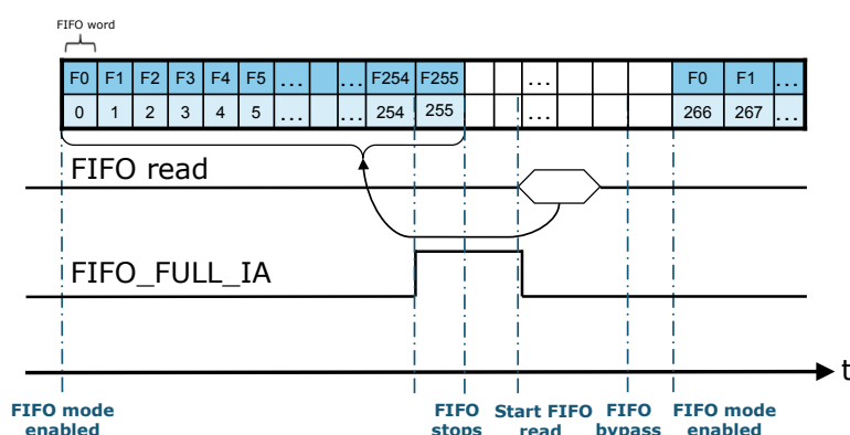
Figure 19. FIFO mode (STOP_ON_WTM = 0)
