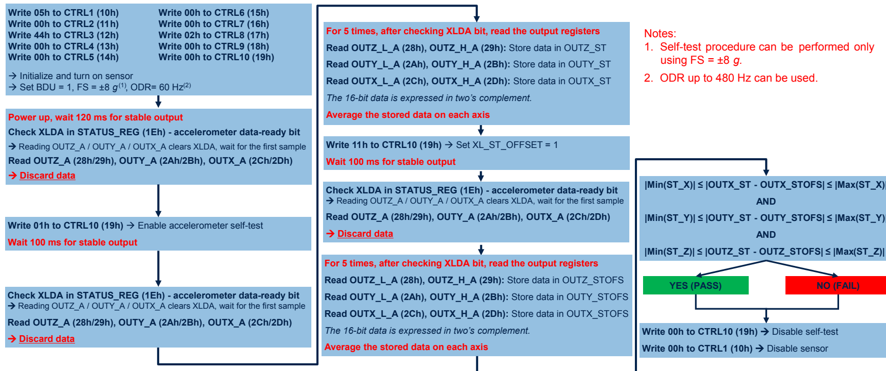
Figure 29. Accelerometer self-test procedure
