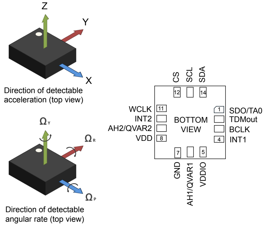
Figure 1. Pin connections
