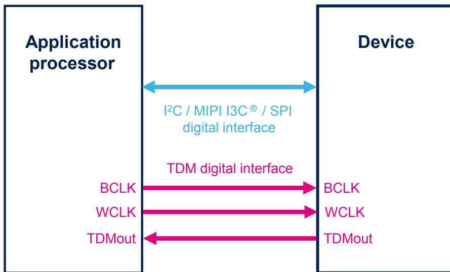
Figure 17. Audio interface connections in mode 2 - TDM mode
