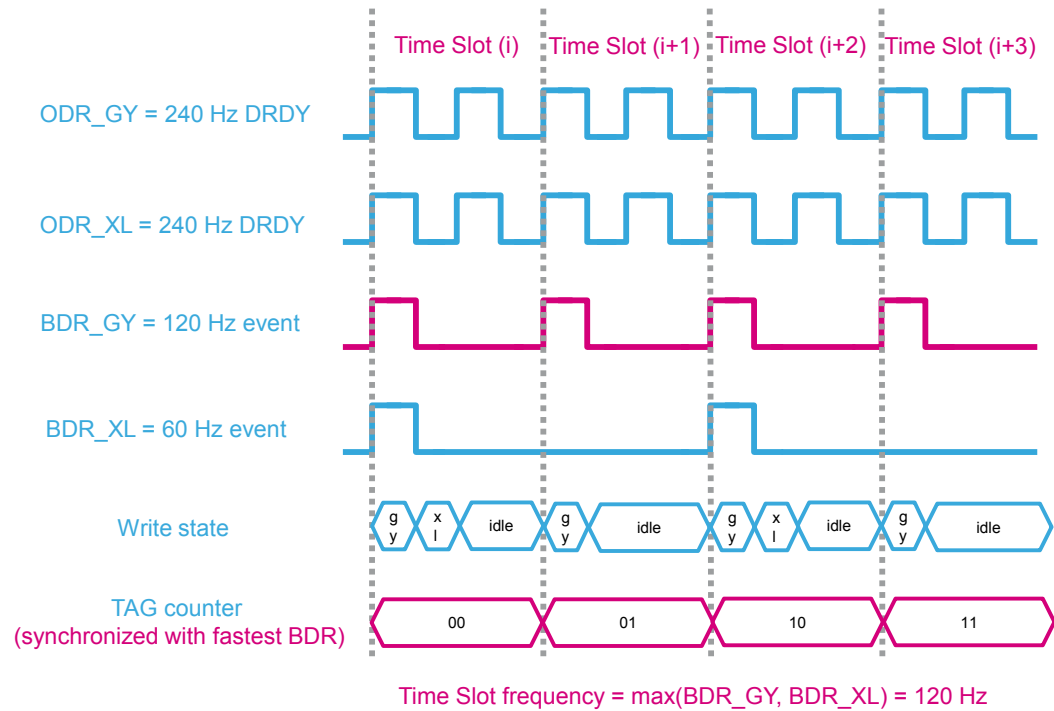
Figure 18. Main sensors and time slot definitions
