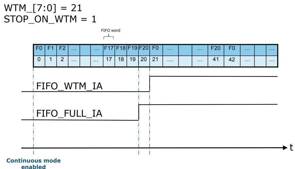
Figure 27. FIFO threshold (STOP_ON_WTM = 1) in continuous mode
