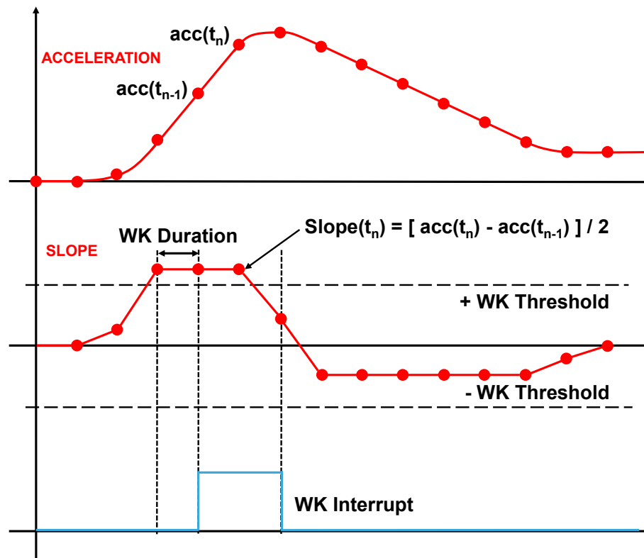
Figure 10. Wake-up interrupt (using the slope filter)
