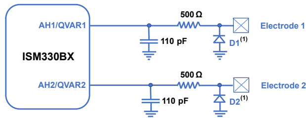
Figure 28. Qvar external connections
