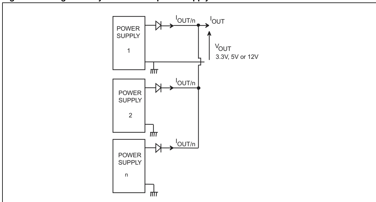
Figure 1. OR-ing Schottky in redundant power supply
