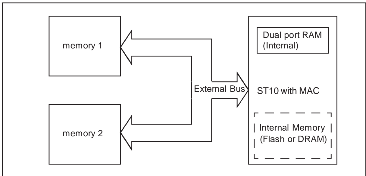
Figure 1 System overview
