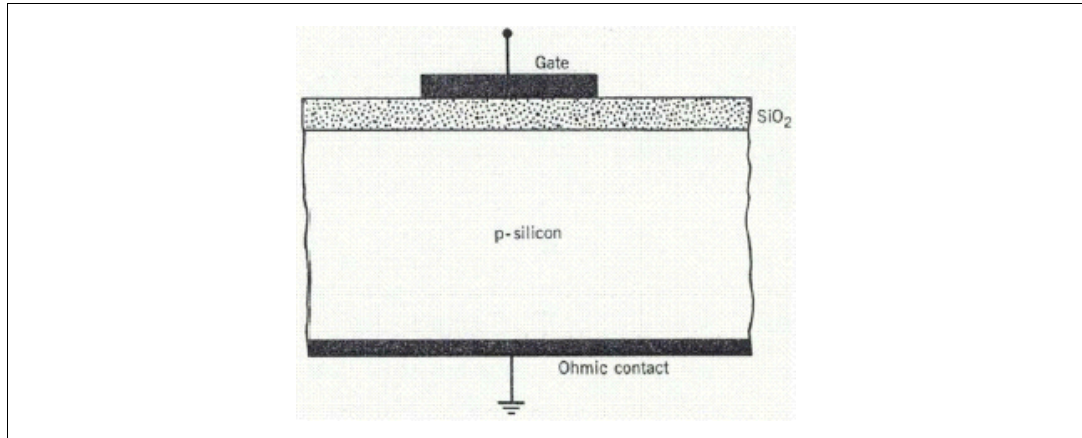
Figure 1. Cross section view of a MOS capacitor
