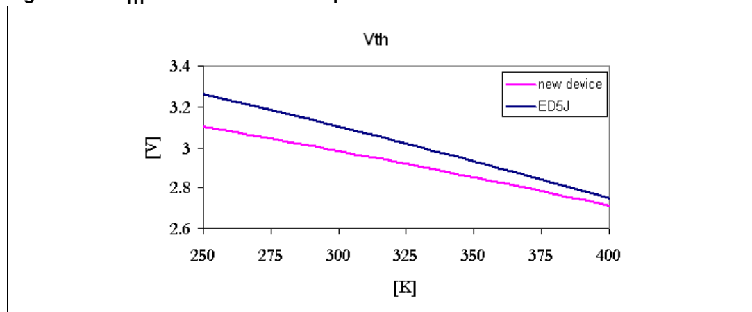
Figure 23. V_{TH} simulated data - comparison between DEVICE1 and the new device
