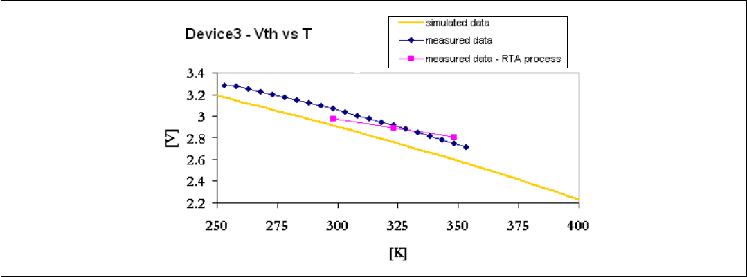
Figure 28. DEVICE3 V_{TH} - comparison between simulated and measured data
