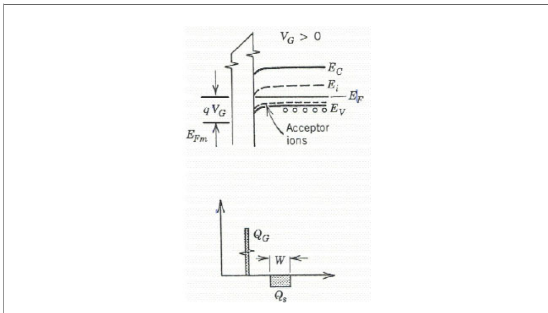
Figure 4. Energy band diagram and charge distribution in an ideal MOS capacitor in depletion condition.
