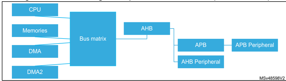
Figure 1. DMA block diagram for products with two DMAs (DMA and DMA2)
