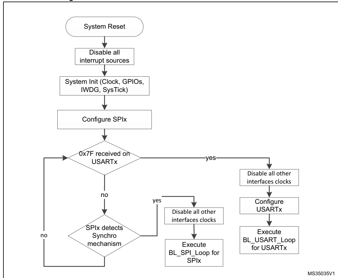
Figure 78. Bootloader selection for STM32L05xxx/06xxx
