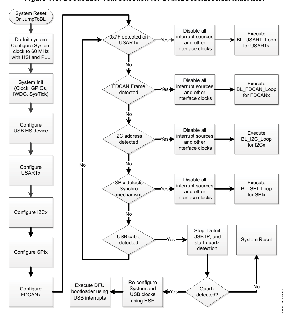
Figure 119. Bootloader V9.x selection for STM32U595xx/99xx/A5xx/A9xx
