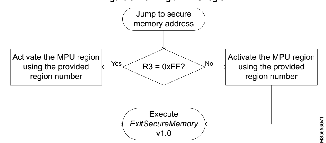
Figure 8. Defining an MPU region
