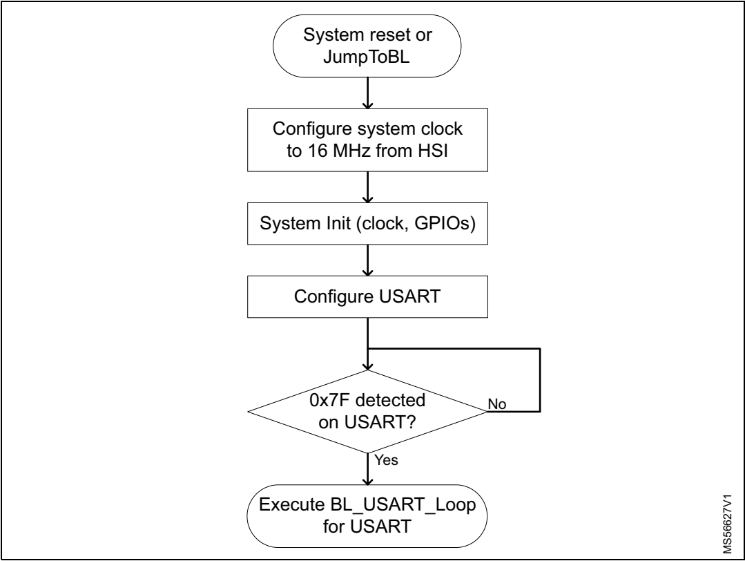
Figure 111. Bootloader V1.x selection for STM32WB09xx
