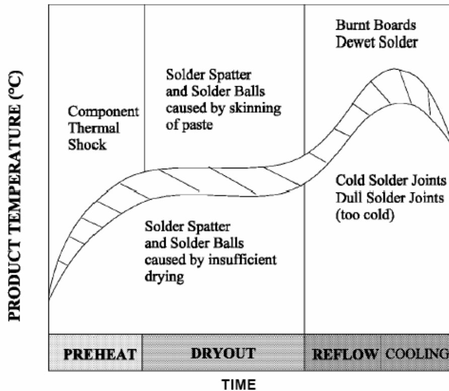
Figure 2. Typical reflow soldering profile
