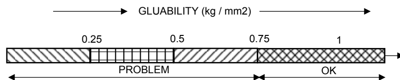
Figure 5. Gluability evaluation with a shear test
