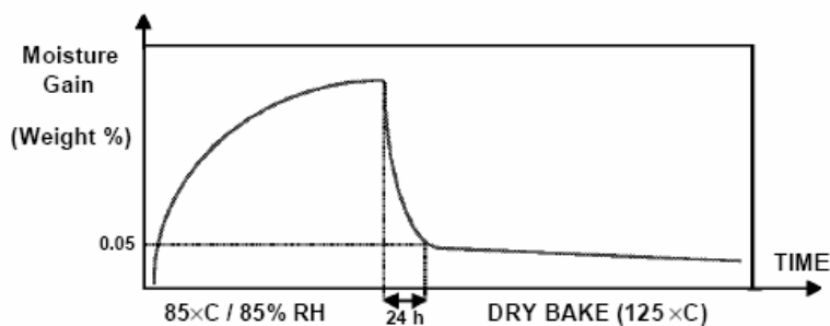
Figure 7. Moisture absorption/drying curve
