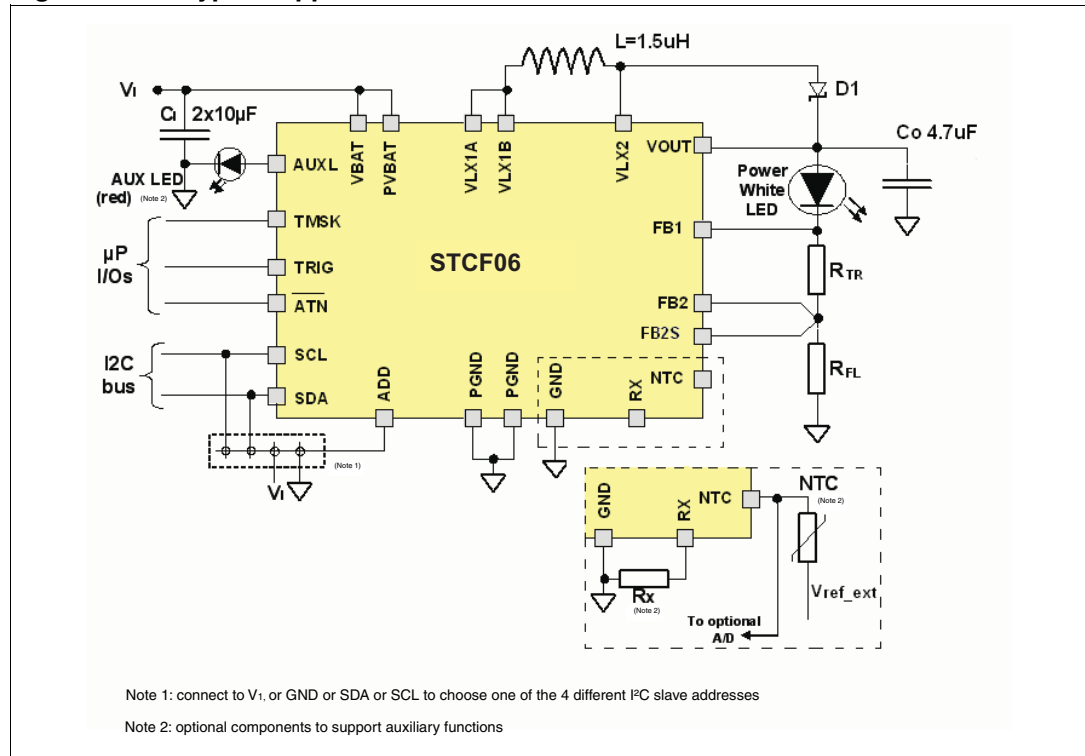
Figure 2. A typical application schematic
