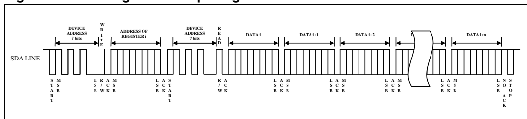
Figure 12. Reading from multiple registers
