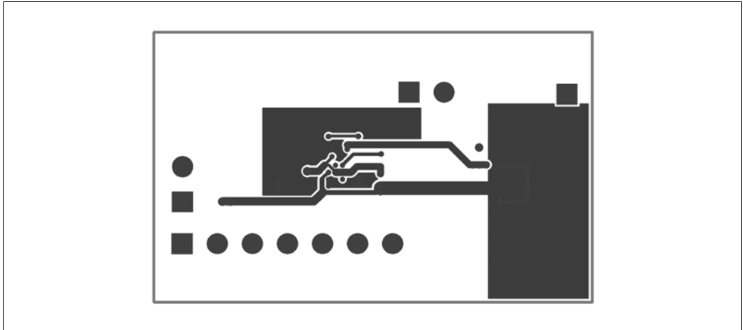
Figure 5. Middle layer 2
