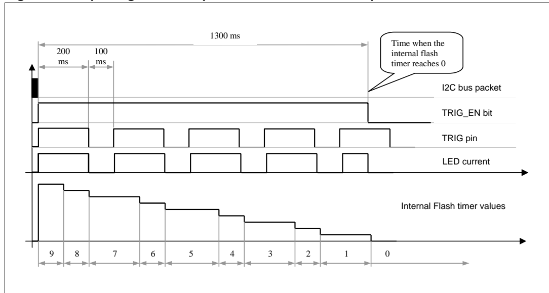
Figure 8. Splitting the Flash pulse into several shorter pulses
