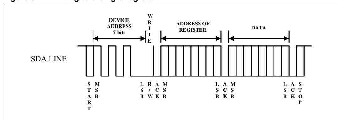
Figure 9. Writing to a single register
