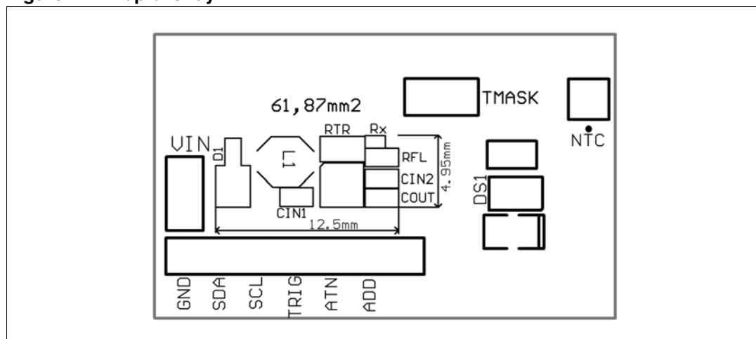
Figure 7. Top overlay
