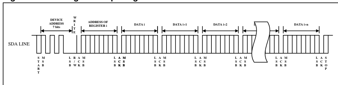
Figure 10. Writing to multiple registers
