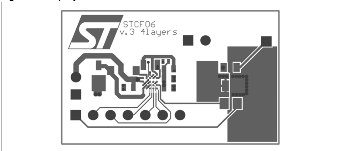
Figure 3. Top layer
