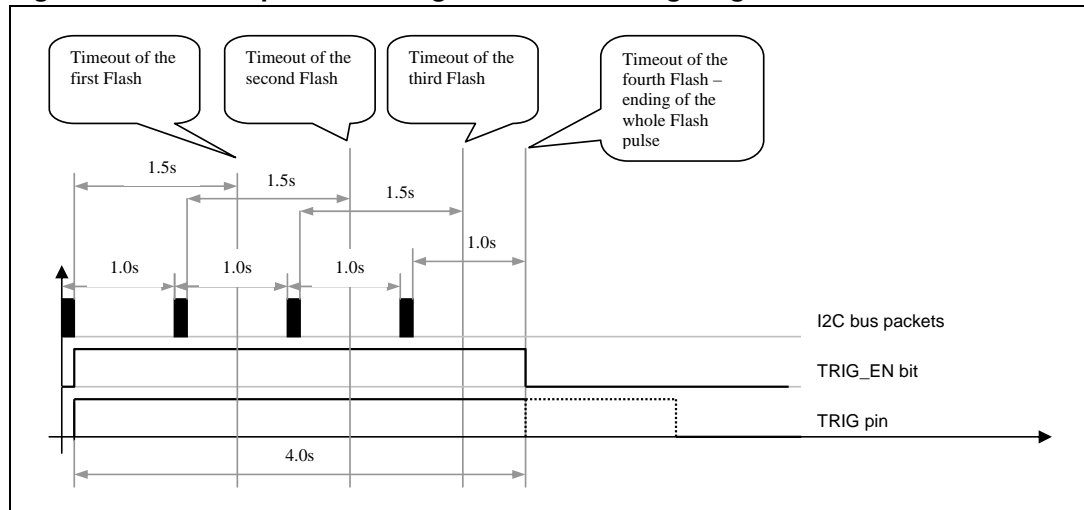
Figure 14. I 2 C bus packets timing for a Flash lasting longer than FTIM max
