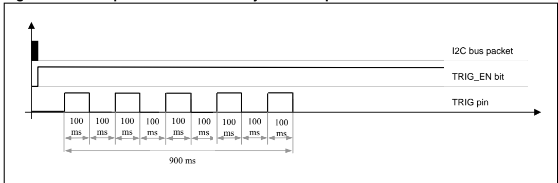
Figure 13. Multiple flashes handled by the TRIG pin
